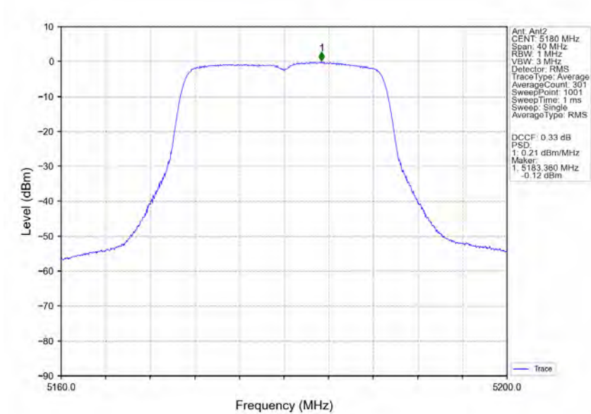
802.11ac(VHT20) LCH_5180MHz_Ant2_NTNV
