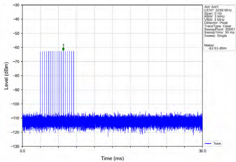
Signal Calibration_802.11ax(HEW160)_2A_5250MHz_RadarType3_Trial0
