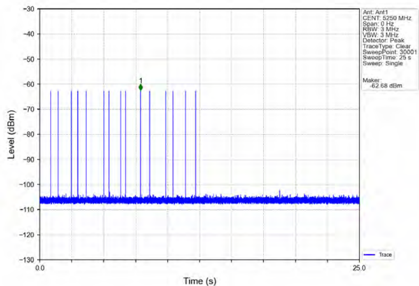
Signal Calibration_802.11ax(HEW160)_2A_5250MHz_RadarType5_Trial0
