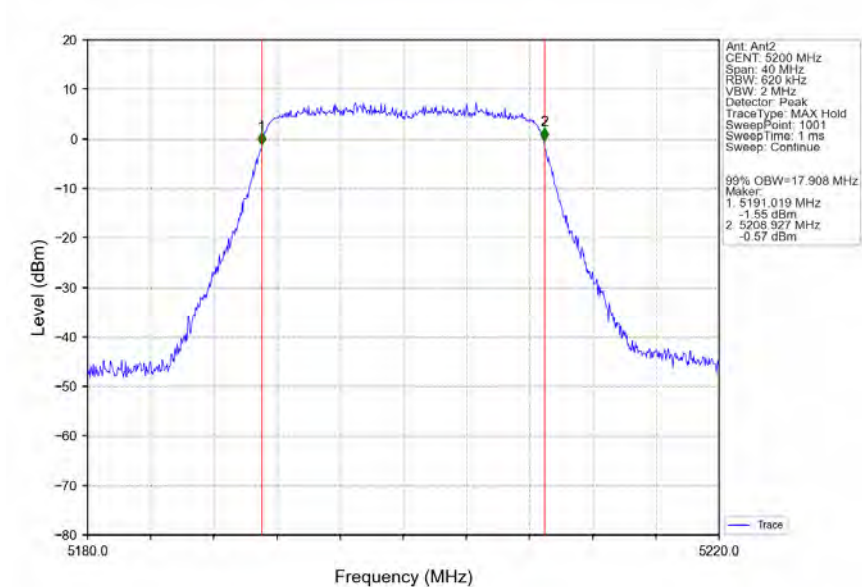
802.11ac(VHT20) MCH_5200MHz_Ant2_NTNV
