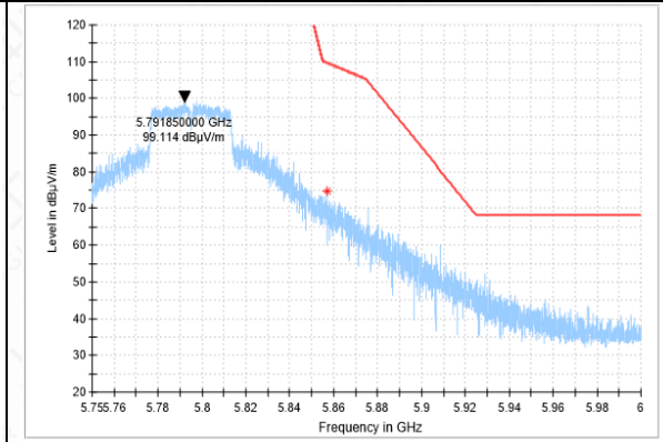
Bandedge-11N(40M)-CH159-PK
