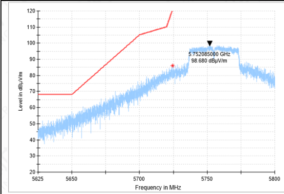
Bandedge-11N(40M)-CH151-PK
