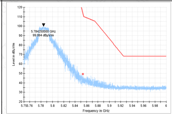
Bandedge-11AC(40M)-CH151-PK
