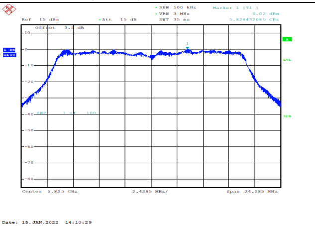
U-NII-3 Power spectral density-802.11 ac(VHT20),5825MHz,Ant1
