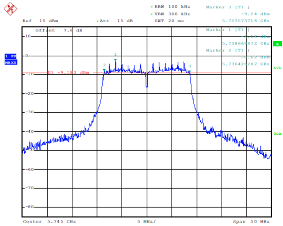
Occupied 6dB Bandwidth ( MHz) (802.11ac-VHT20, 5745MHz)
