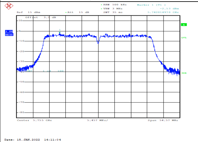
U-NII-3 Power spectral density-802.11 ac(VHT40),5755MHz,Ant1
