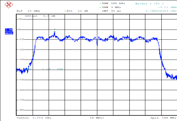
U-NII-3 Power spectral density-802.11 ac(VHT80),5775MHz,Ant1
