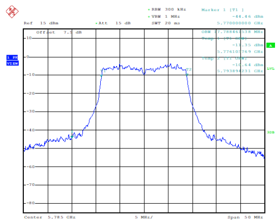
99% Occupied Bandwidth ( MHz) (802.11ac-VHT20, 5785MHz)
