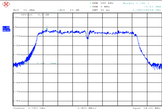
U-NII-3 Power spectral density-802.11 ac(VHT40),5795MHz,Ant1
