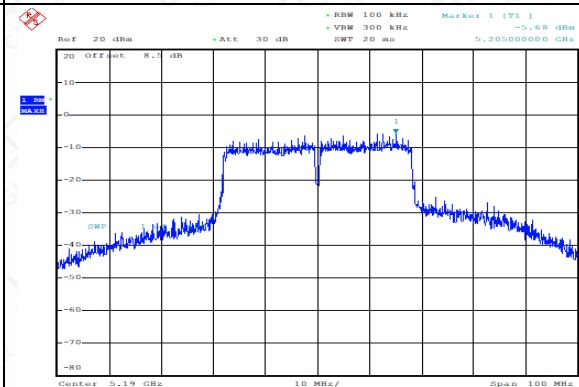
Power Spectral Density(dBm/MHz) (802.11ac-VHT40), 5190MHz)
