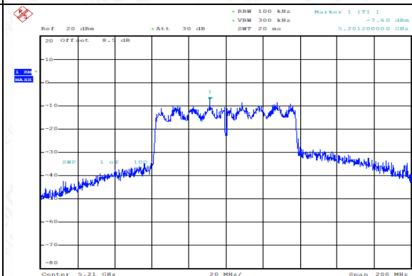
Power Spectral Density(dBm/MHz) (802.11ac-VHT80), 5210MHz)
