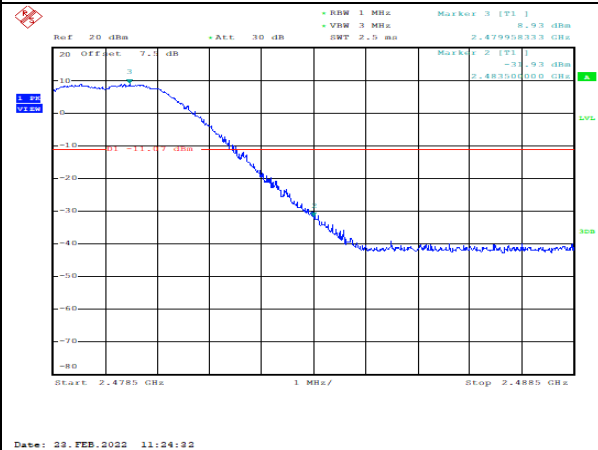
Frequency Band Edge: 8DPSK, Ch78, Hopping ON
