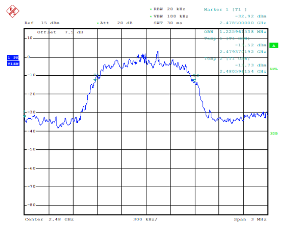
99% Bandwidth: DQPSK, Ch78
