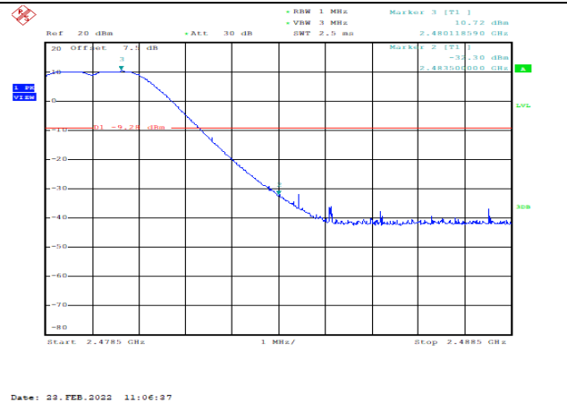
Frequency Band Edge: GFSK, Ch78, Hopping ON
