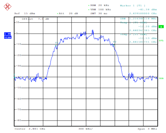
99% Bandwidth: 8DPSK, Ch39
