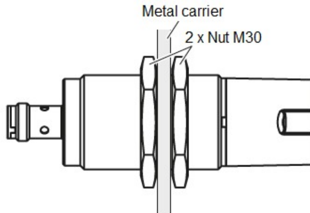
Figure 2: BF-IDU08 mounted on metal carrier using 2 x Nut M30
