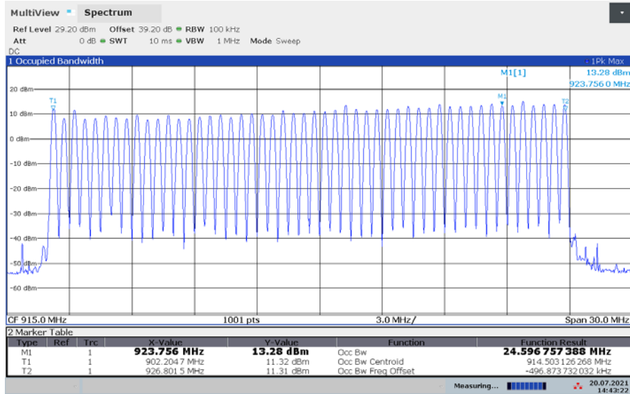
Plot 1: Number of hopping channels
