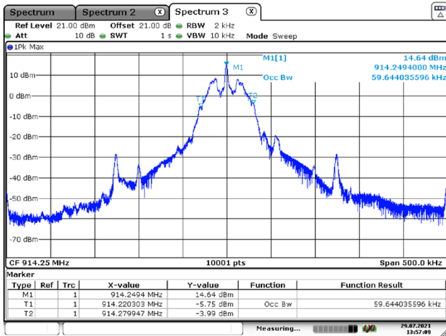
Plot 4: mid channel, 99% OBW
