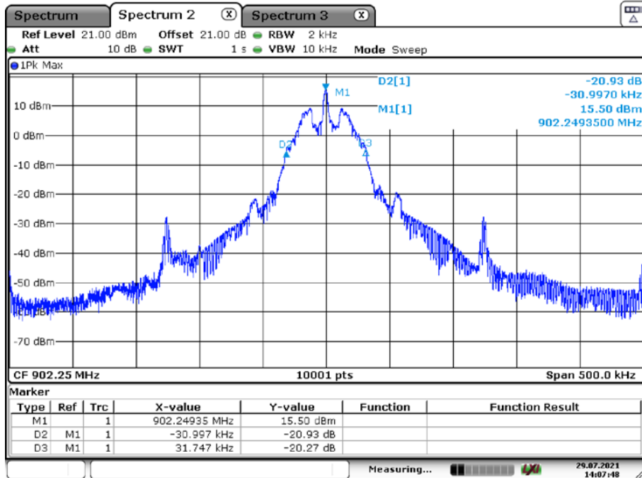
Plot 1: low channel, 20 dB BW
