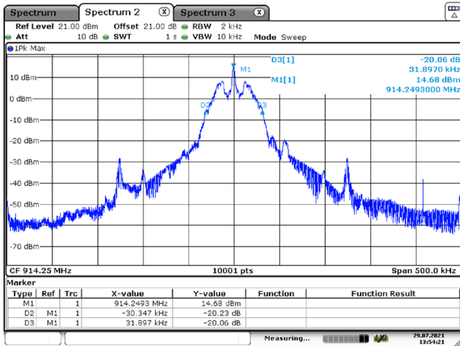
Plot 3: mid channel, 20 dB BW
