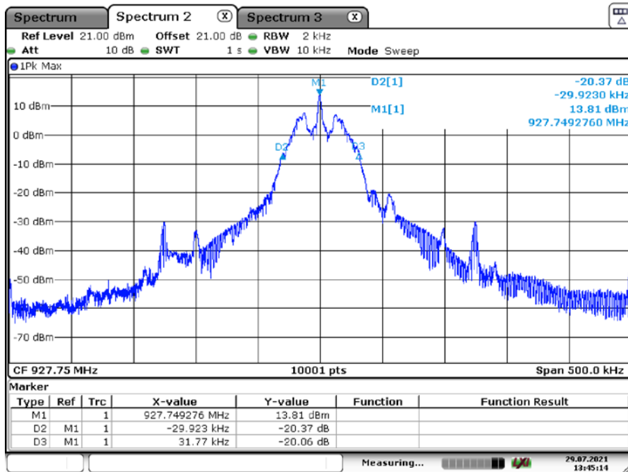
Plot 5: high channel, 20 dB BW
