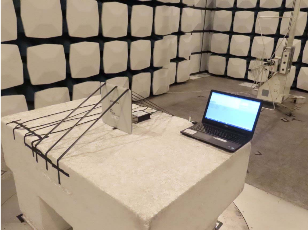
Front View of Spurious Emission Test (BIS U-626-069-111-06-ST31)
