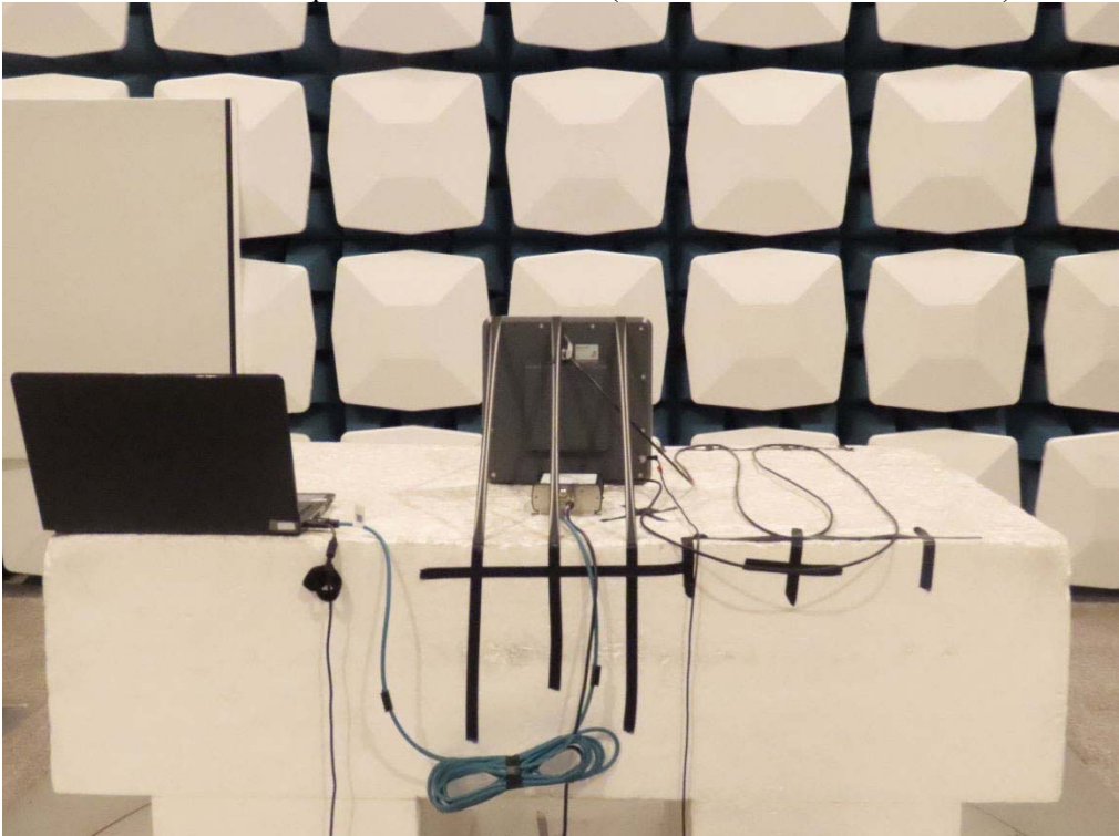
Back View of Spurious Emission Test (BIS U-626-069-111-06-ST31)
