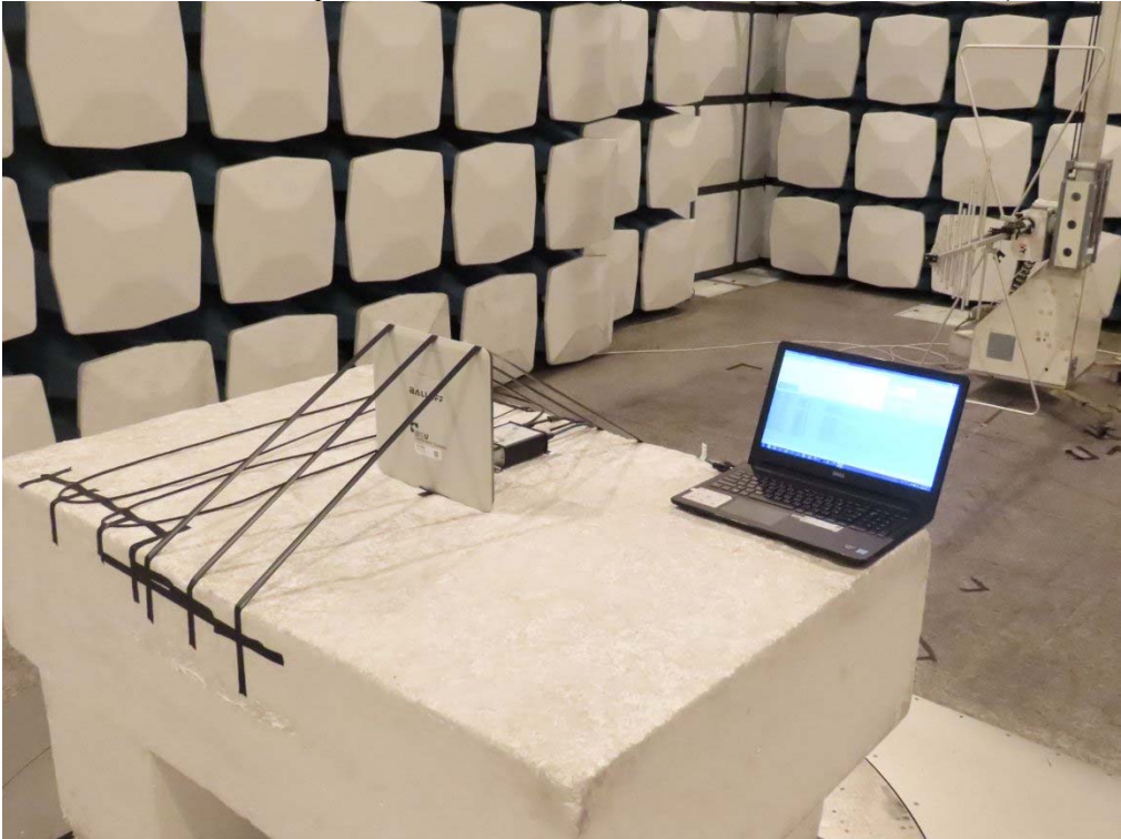
Front View of Spurious Emission Test (BIS U-626-069-111-06-ST32)
