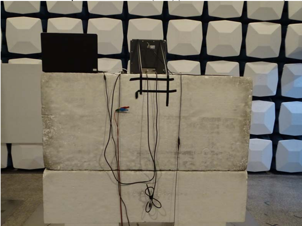
Back View of Spurious Emission Test (Horn) (BIS U-620-068-111-00-ST29)
