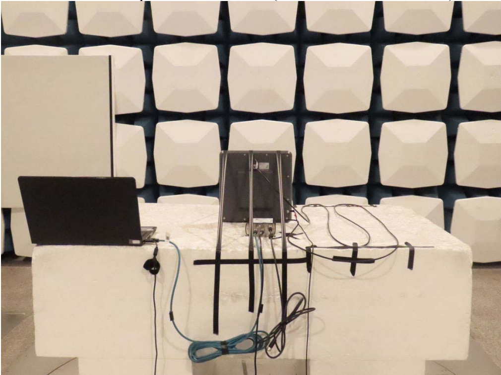
Back View of Spurious Emission Test (BIS U-626-069-111-06-ST32)
