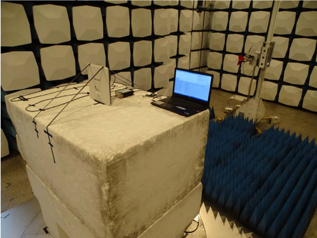
Front View of Spurious Emission Test (Horn) (BIS U-620-068-111-00-ST29)
