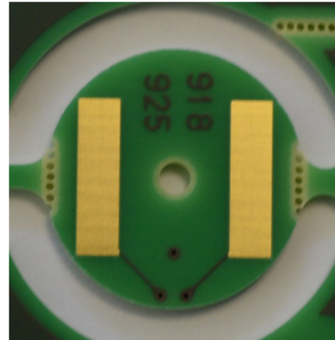
Antenna Top
