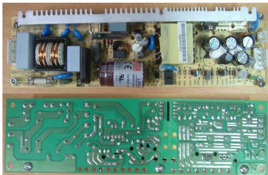
Power supply board (Mean Well, Model LPS-50-15)
