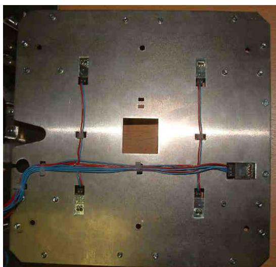
LED board (rear face)
