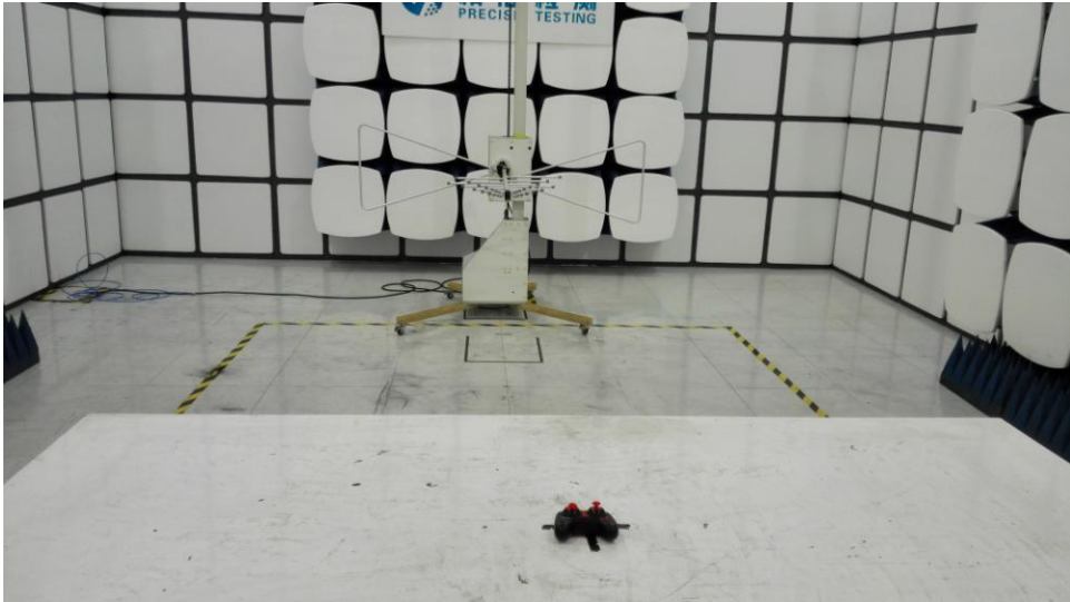
Radiated Emission Test below 1GHz
