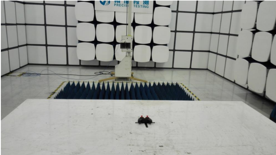
Radiated Emission test above 1GHz
