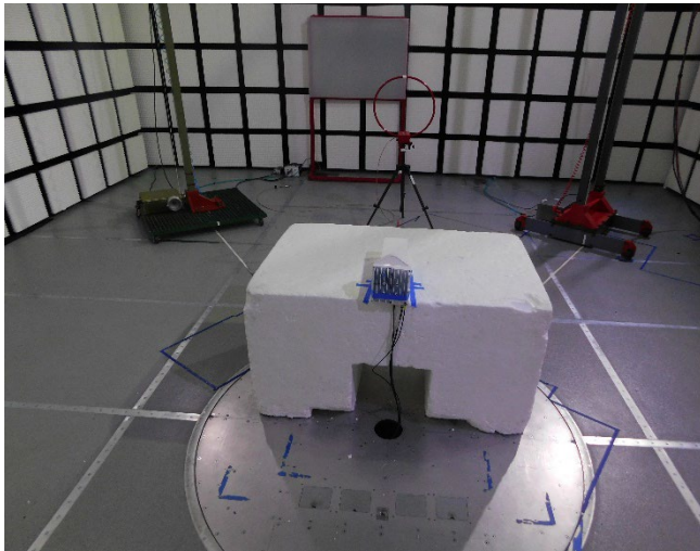
BLE/UNII BL30M 0 Deg
