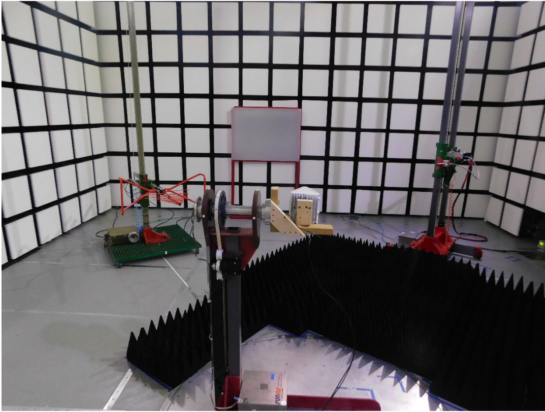
BLE/UNII A1G Back
