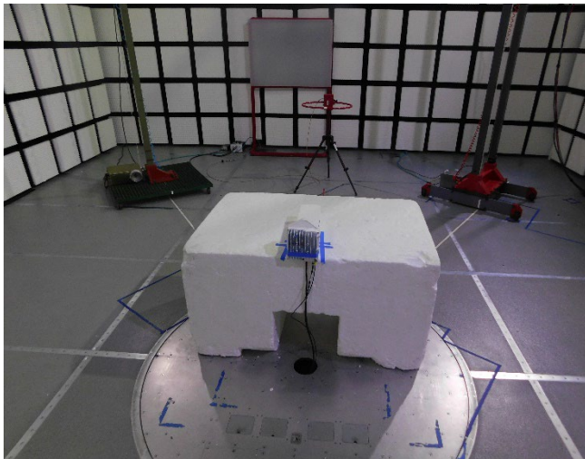
BLE/UNII BL30M Flat
