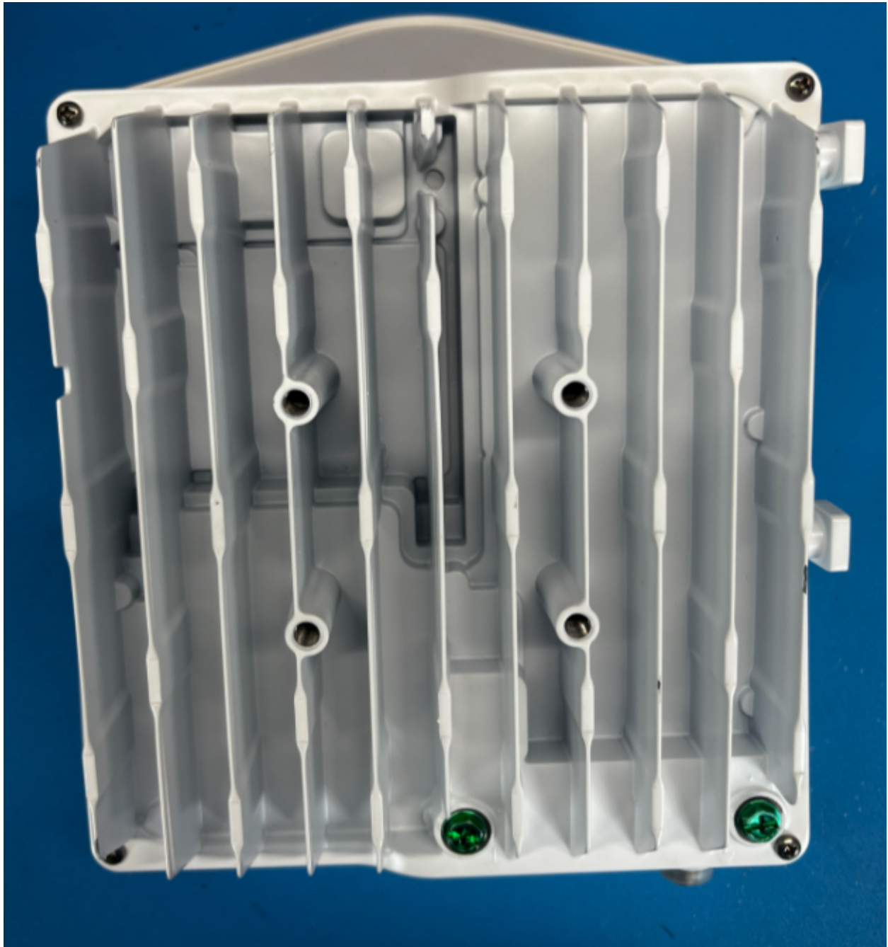
Figure 2: Back assembly view, external
