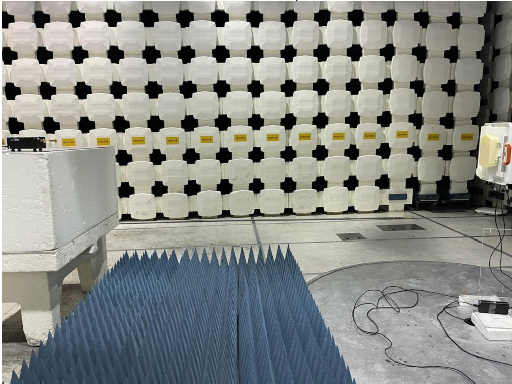
40-100 GHz Test Setup Photo 1
