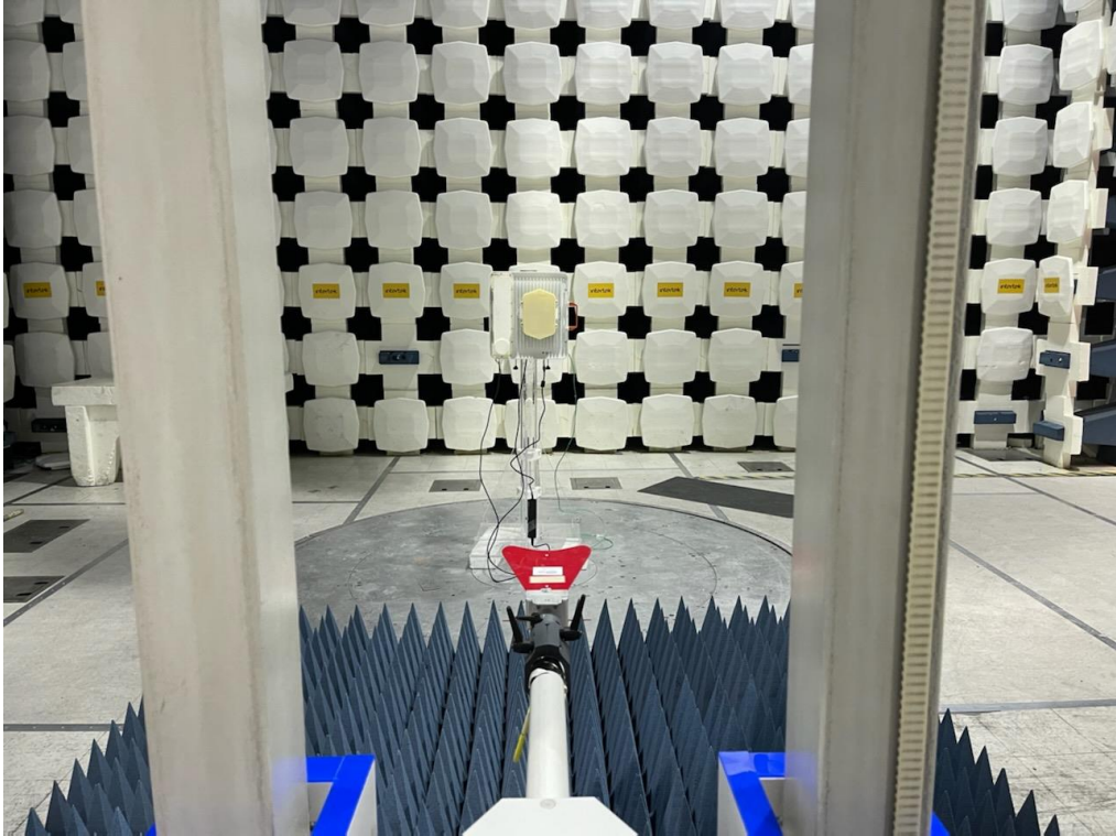
1-18 GHz Test Setup Photo 1
