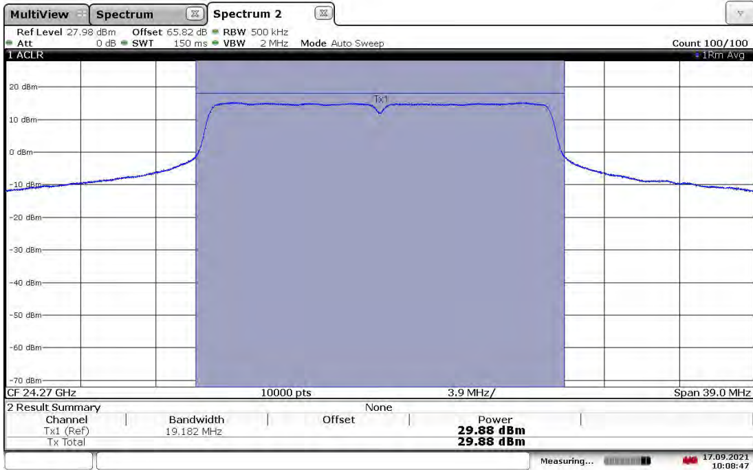
EIRP Output Power (Vertical Polarity) – S01411_24.27GHz_BW20M_MCS8_Path 3_att16.5
