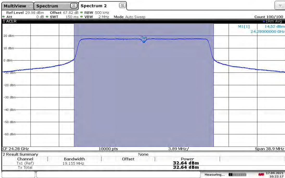
EIRP Output Power (Vertical Polarity) – S01411_24.28GHz_BW20M_MCS8_Path 3_att16
