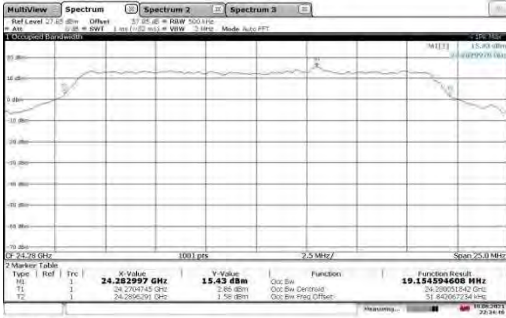
Occupied Bandwidth (Vertical Polarity) – S01411_24.28GHz_BW20M_MCS8_Path 3
