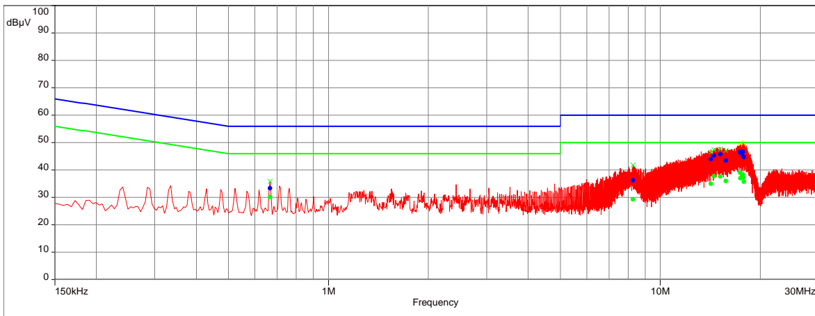
test name Single Phase Under 15 Amp_150kHz to 30 MHz ESCI_120VAC 60Hz_Titan 24_Tx/Normal operation mode Time ate 18/6/2021 18:1
