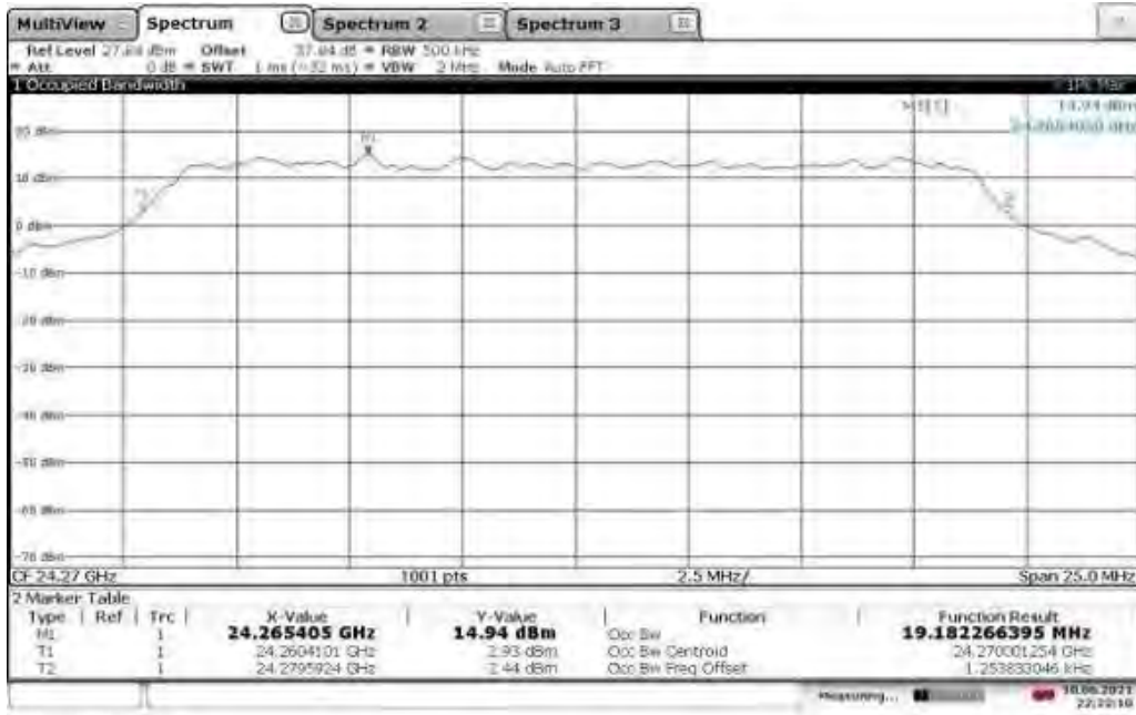
Occupied Bandwidth (Vertical Polarity) – S01411_24.27GHz_BW20M_MCS8_Path 3
