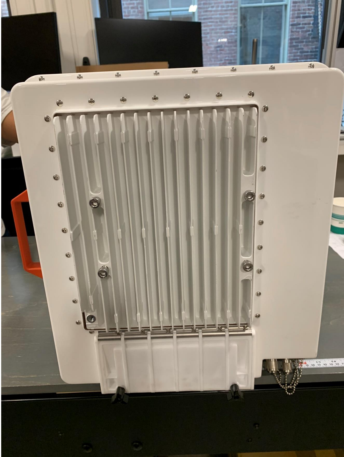
Figure 2. Rear Assy View, External
