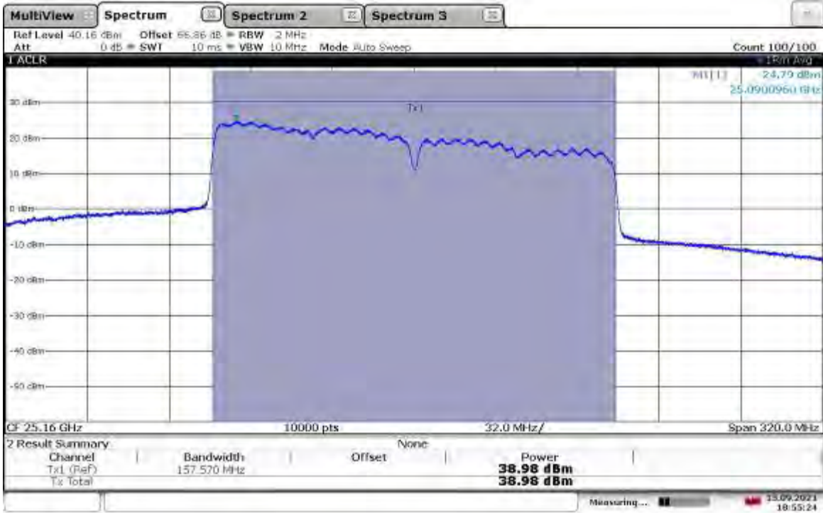
EIRP Output Power (Vertical Polarity) – 25.16_160MHz BW_MCS0_att0.5_Mixer23
