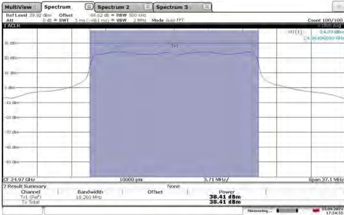
EIRP Output Power (Vertical Polarity) – 24.97GHz_20MHz BW_MCS8_att0.25_Mixer25
