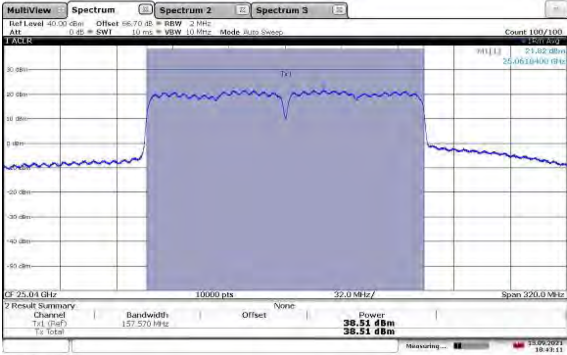
EIRP Output Power (Vertical Polarity) – 25.04_160MHz BW_MCS0_att0.5_Mixer23
