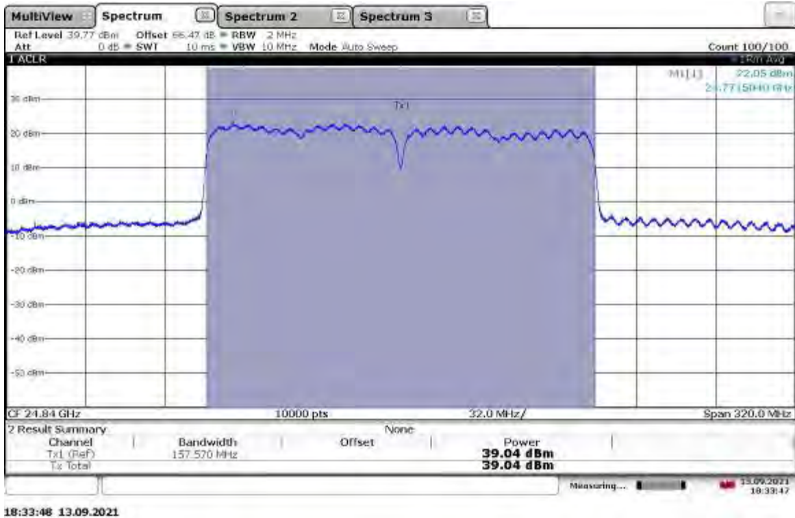
EIRP Output Power (Vertical Polarity) – 24_24.84_160MHz BW_MCS0_att0.25_Mixer23
