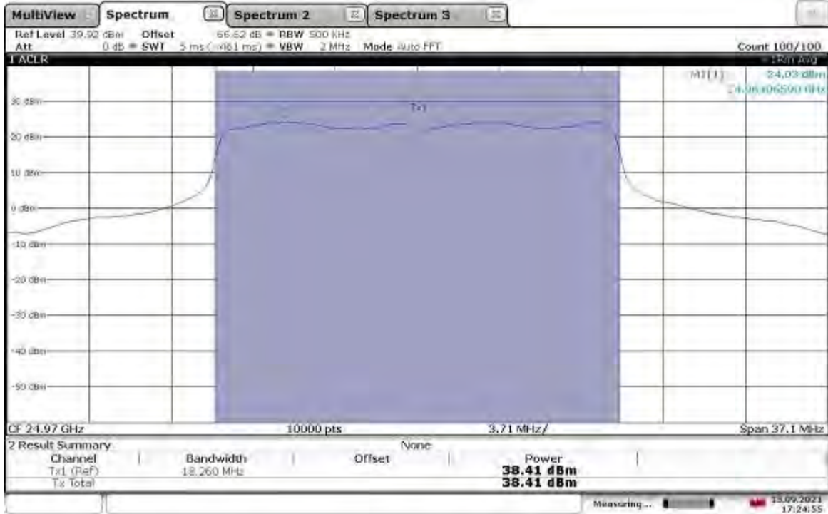
EIRP Output Power (Horizontal Polarity) – 24.97GHz_20MHz BW_MCS8_att0_Mixer27
