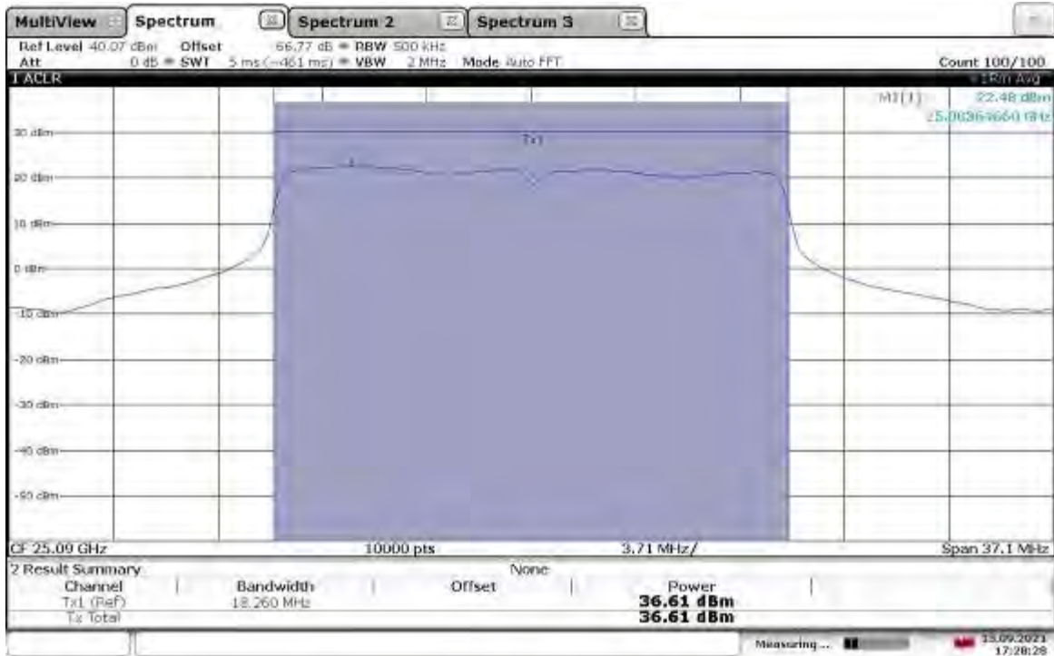
EIRP Output Power (Horizontal Polarity) – 25.09GHz_20MHz BW_MCS8_att0.5_Mixer24
