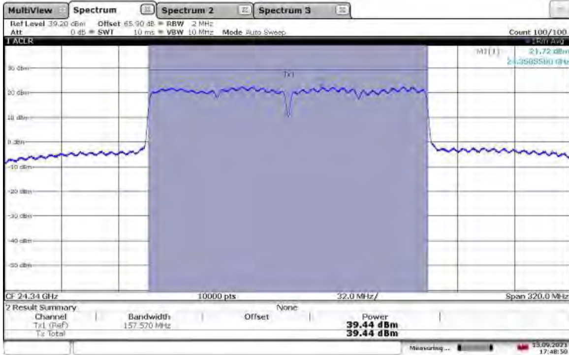
EIRP Output Power (Vertical Polarity) – 24.34_160MHz BW_MCS0_att0.5_Mixer26
