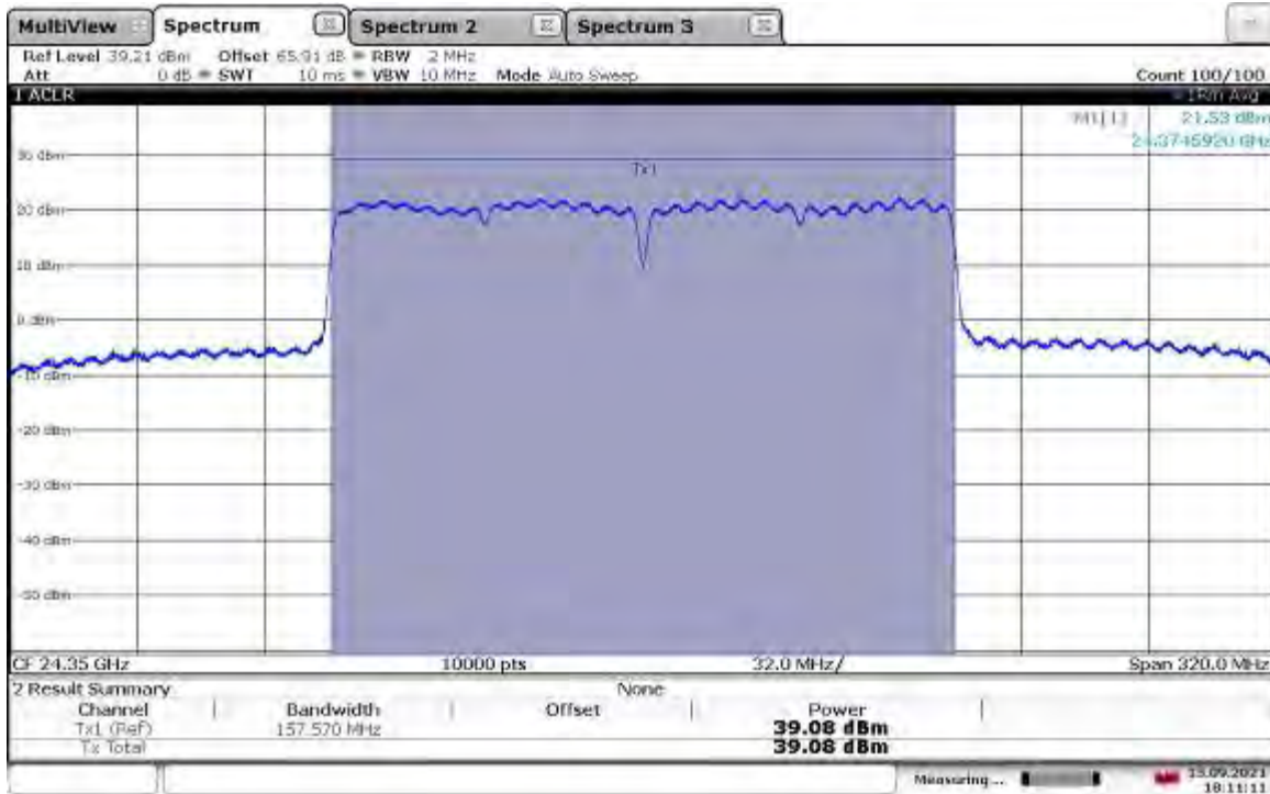
EIRP Output Power (Vertical Polarity) – 24.35_160MHz BW_MCS0_att0.75_Mixer26
