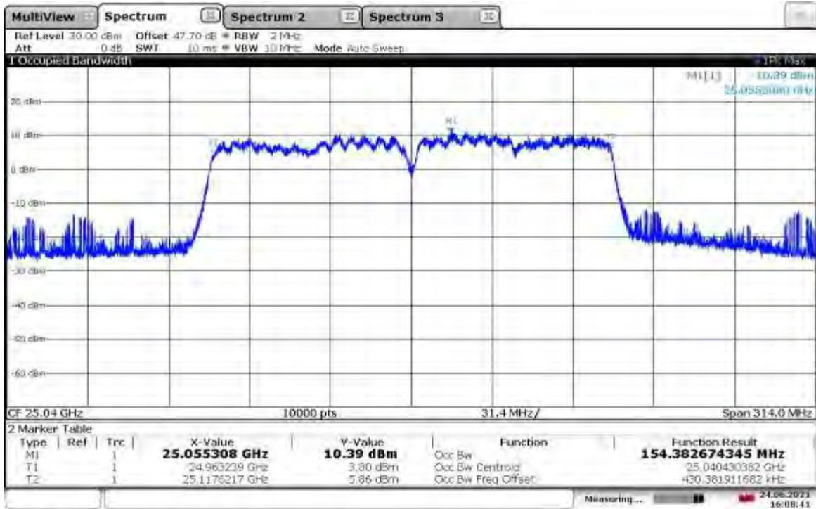
Occupied Bandwidth (Vertical Polarity) – 25.04GHz_BW160M_MCS0_Path 0
