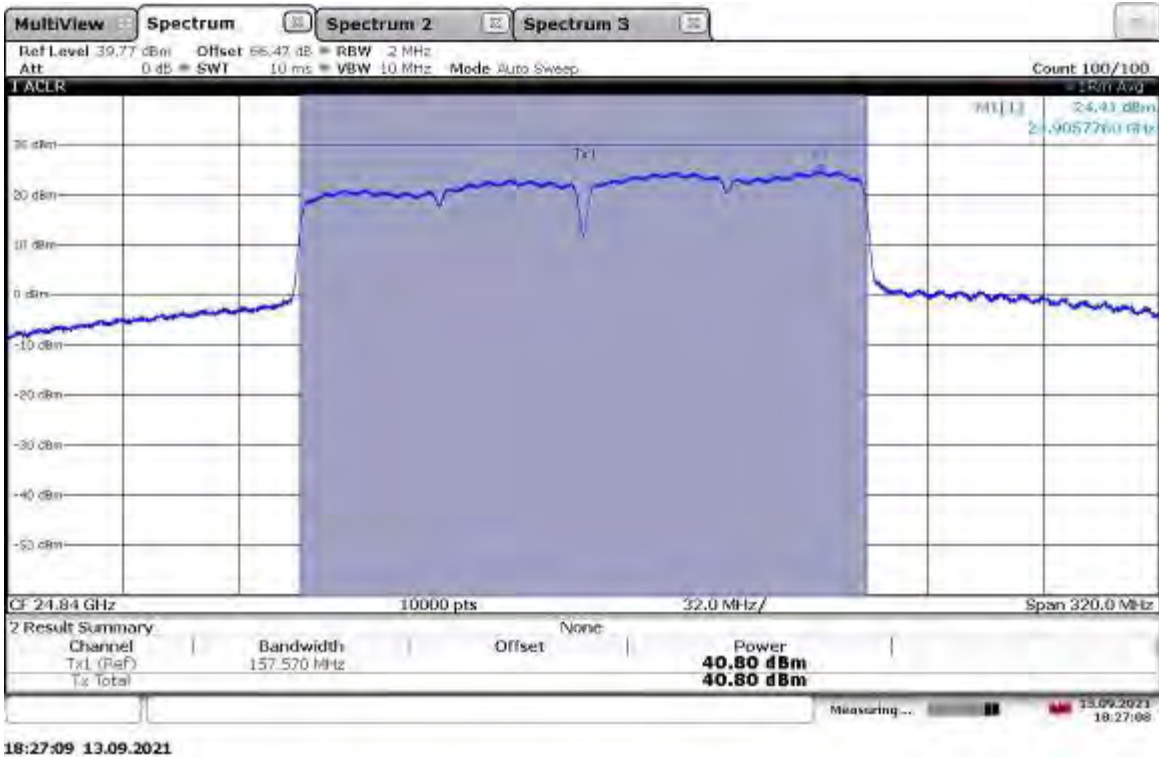
EIRP Output Power (Horizontal Polarity) – 24.84GHz_160BW_MCS0_att0.75_Mixer25
