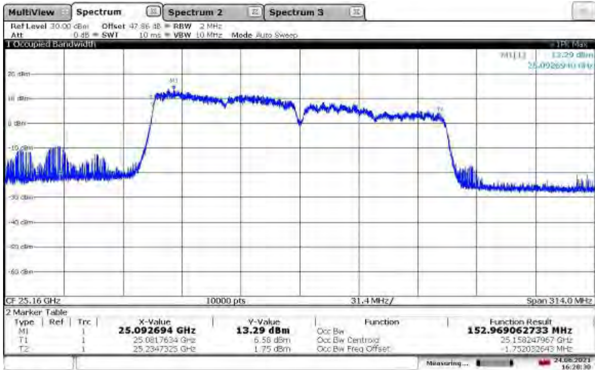
Occupied Bandwidth (Vertical Polarity) – 25.16GHz_BW160M_MCS0_Path 0
