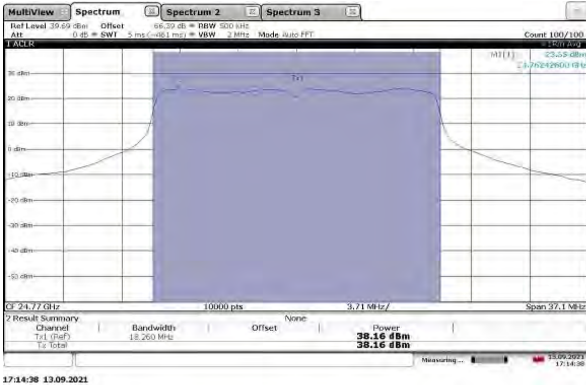
EIRP Output Power (Vertical Polarity) – 24.77GHz_20MHz BW_MCS8_att0_Mixer24
