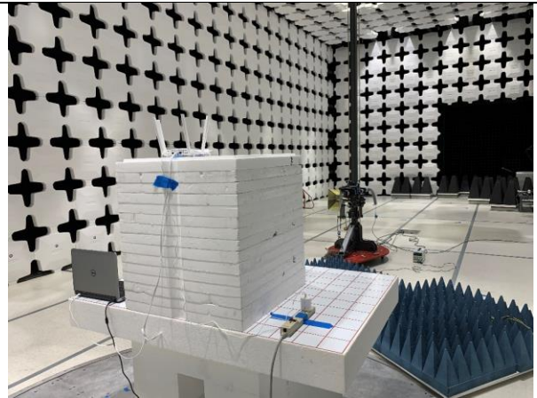
RE Above 1GHz – Rear View
