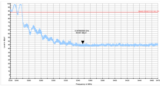
802.11ac HT80 -Channel 42: Peak
