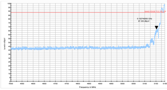
802.11n HT40-Channel 46: Peak
