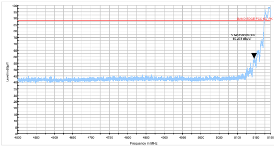
802.11ac HT40-Channel 46: Peak
