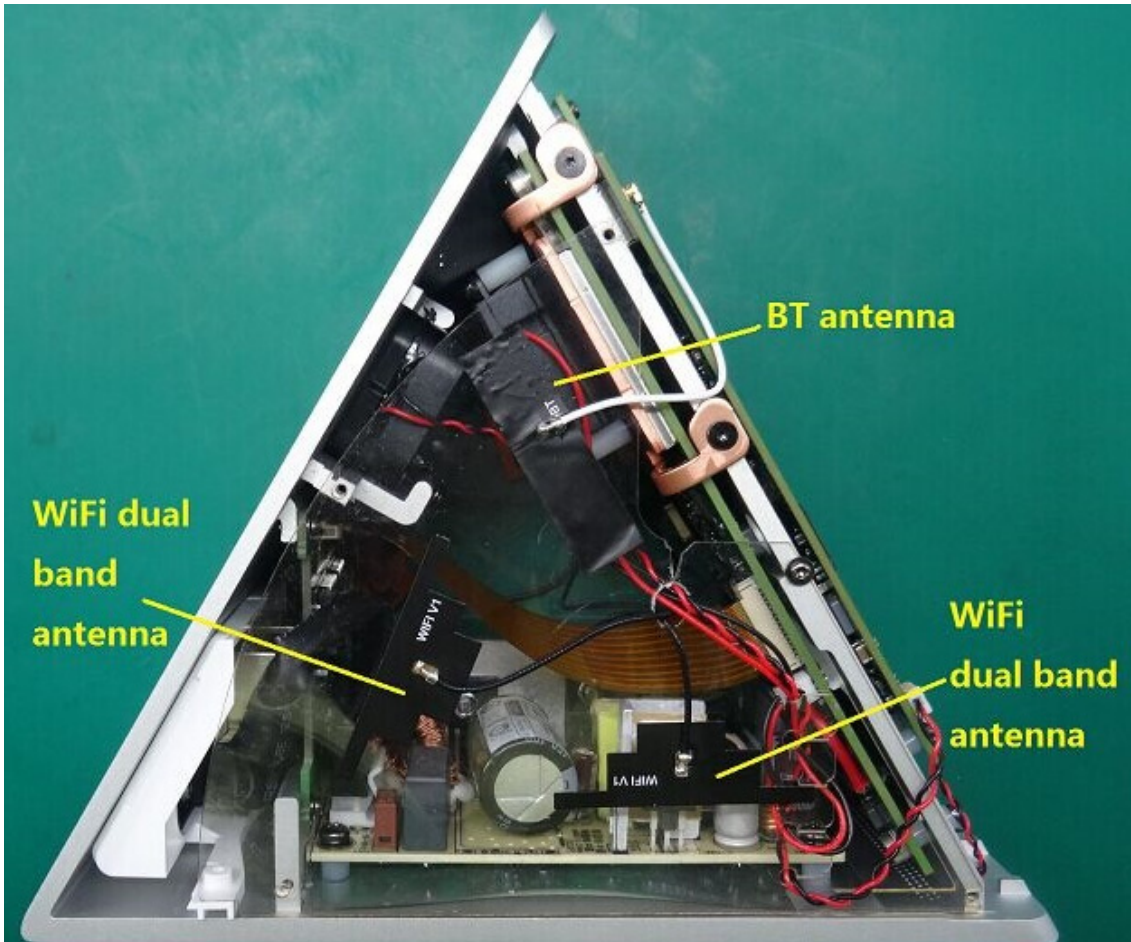
2AGZ3S00111 Internal photo
