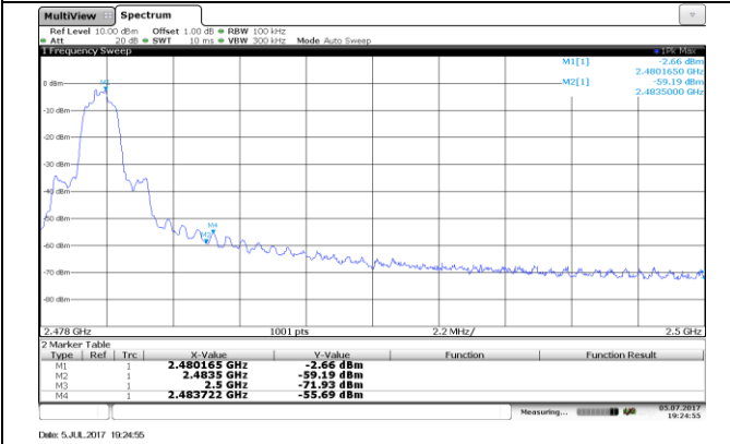
CH78 Bandedge (no hopping mode)
