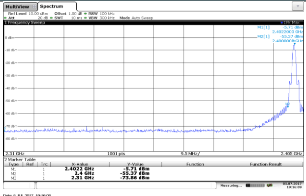
CH00 Bandedge (no hopping mode)
