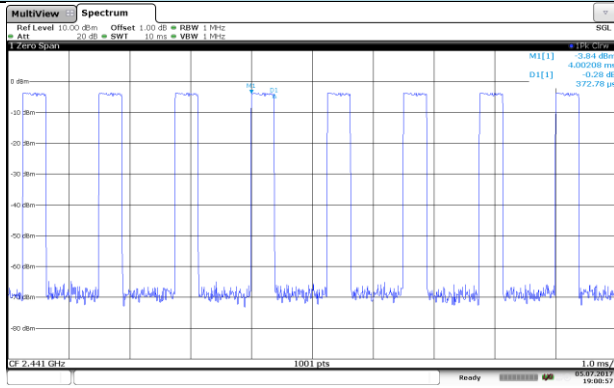
3-DH1
