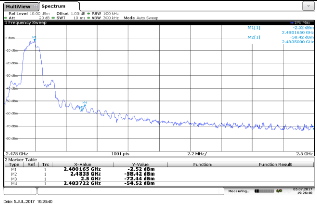
CH78 Bandedge (no hopping mode)
