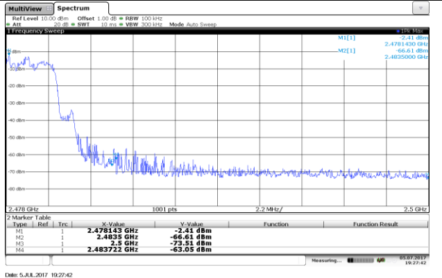
CH78 Bandedge (hopping mode)
