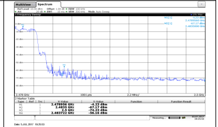
CH78 Bandedge (hopping mode)
