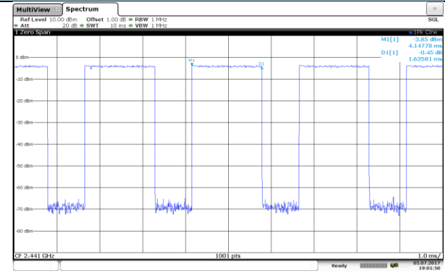
3-DH3
