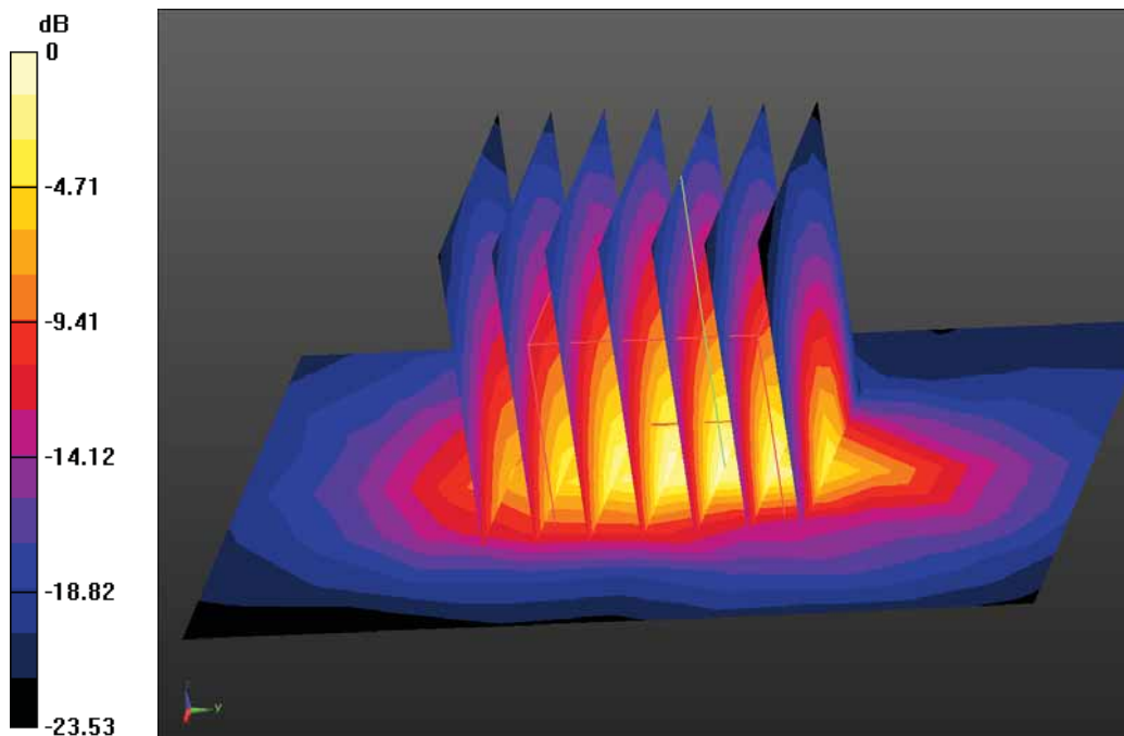
Fig. 2 - Bottom Side High 802.11b Channel 11
