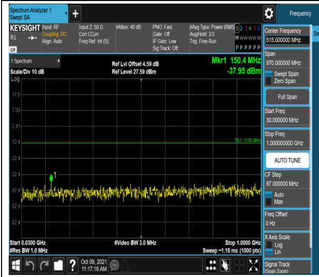
Band4-20MHz-16QAM-20300-1RB#0-Range1:30~1000MHz
