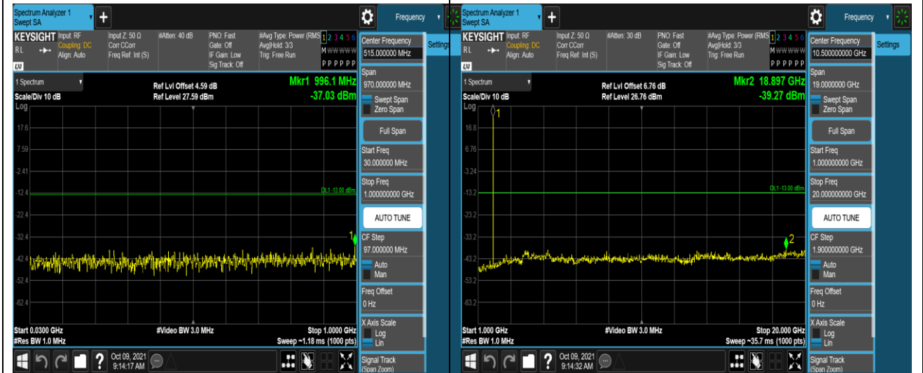
Band2-1.4MHz-QPSK-18900-1RB#0-Range1:30~1000MHz
