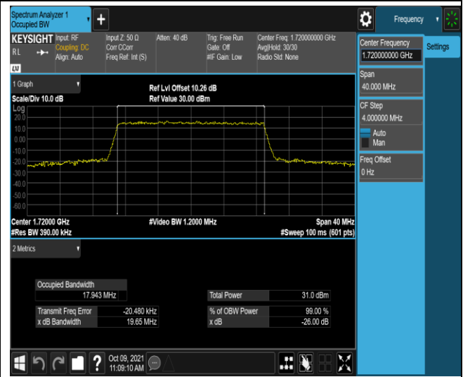
Band4-20MHz-16QAM-20050-100RB#0
