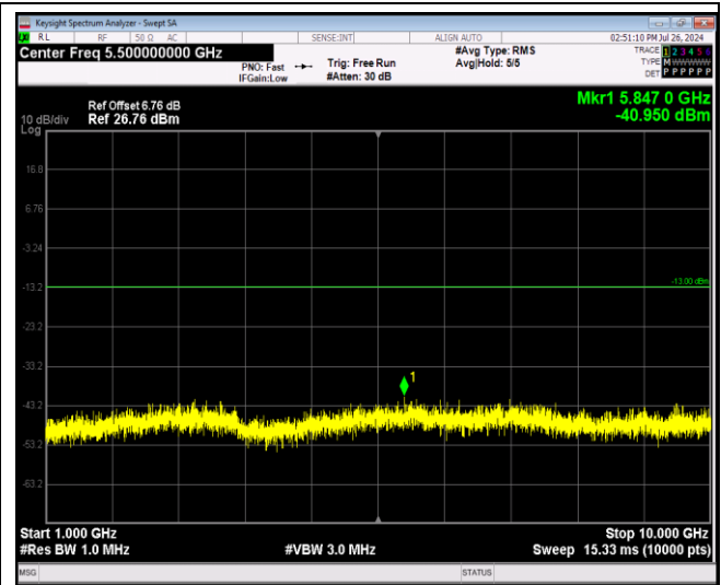
Band17-5MHz-64QAM-23755-1RB#0-Range2:1000~10000MHz
