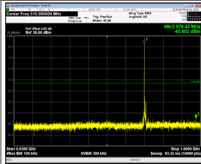
Band17-5MHz-QPSK-23825-1RB#0-Range1:30~100 0MHz
