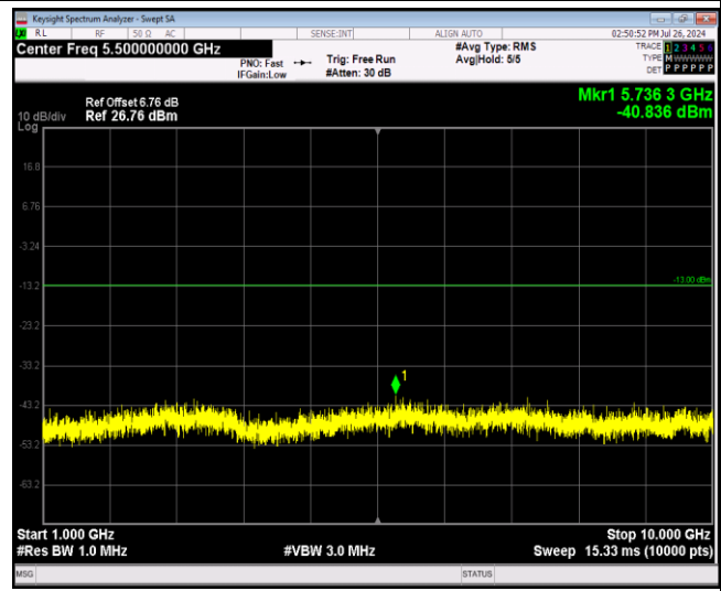
Band17-5MHz-QPSK-23825-1RB#0-Range2:1000~1 0000MHz
