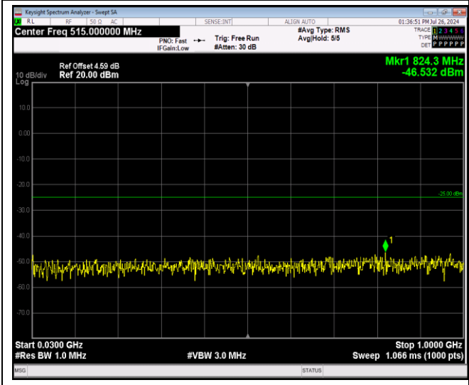
Band7-5MHz-QPSK-20775-1RB#0-Range1:30~1000MHz
