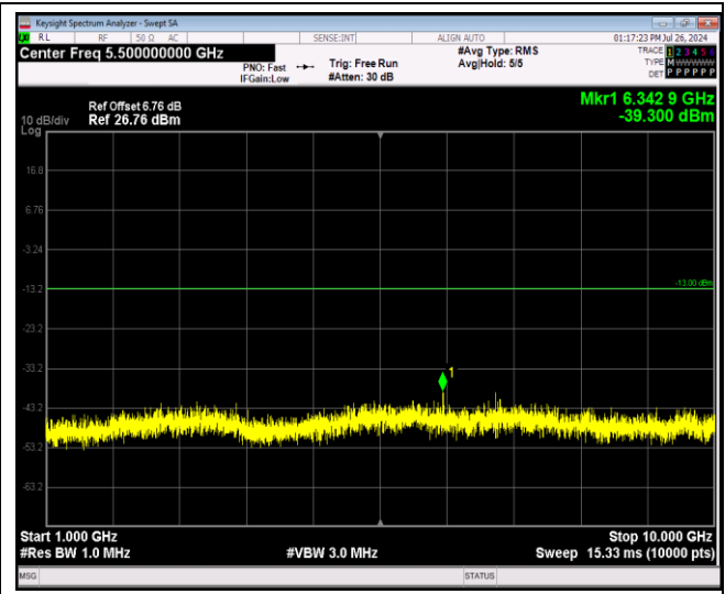
Band5-10MHz-16QAM-20450-1RB#0-Range2:1000~10000MHz
