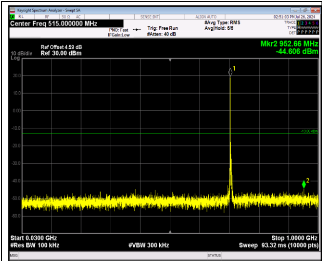
Band17-5MHz-64QAM-23755-1RB#0-Range1:30~1000MHz
