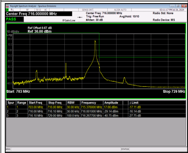
Band17-10MHz-64QAM-23800-1RB#49
