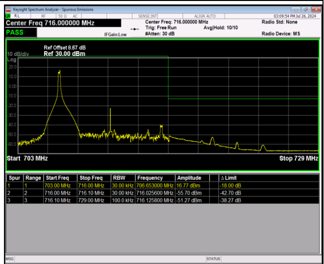
Band17-10MHz-64QAM-23800-50RB#0
