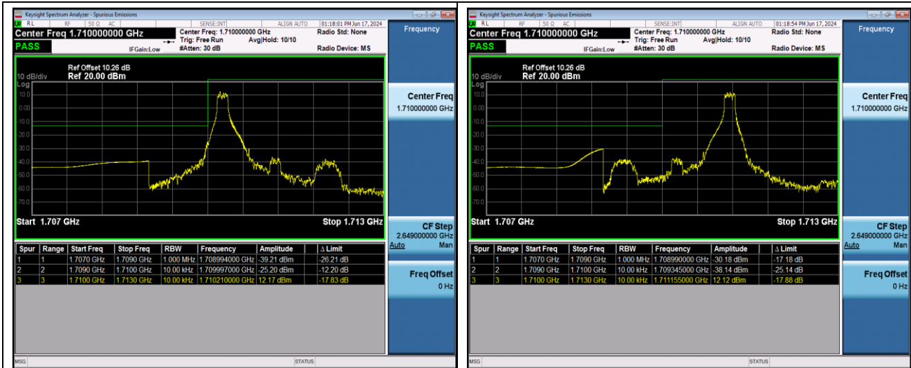
Band4-1.4MHz-16QAM-19957-6RB#0
