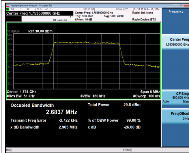
Band4-3MHz-64QAM-20175-15RB#0
