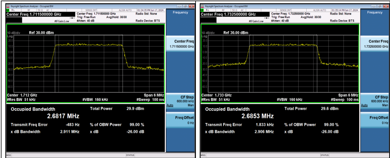
Band4-3MHz-16QAM-20385-15RB#0
