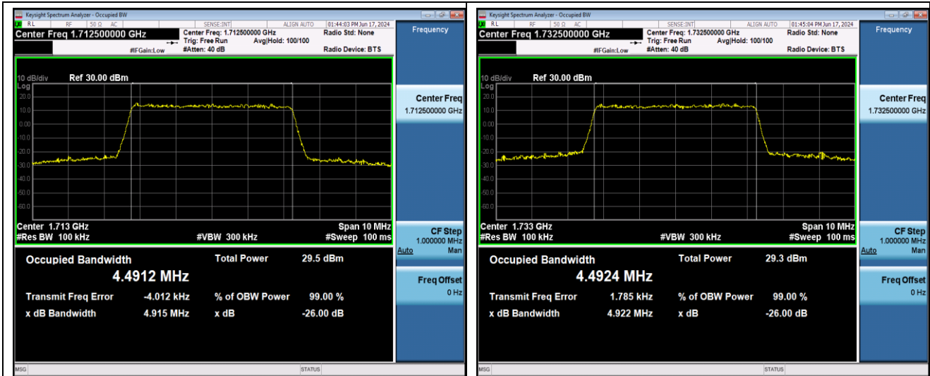
Band4-5MHz-64QAM-20375-25RB#0
