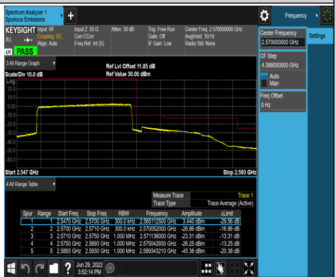
Band7-20MHz-16QAM-2085-1RB#99
