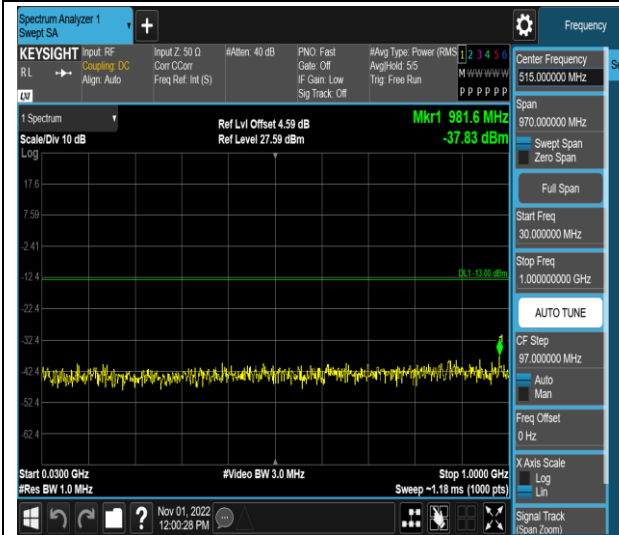
Band4-20MHz-QPSK-20175-1RB#0-Range1:30~1000MHz
