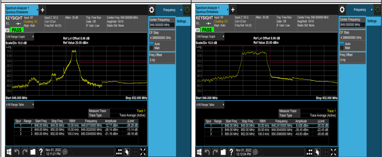
Band5-1.4MHz-16QAM-20407-1RB#0
