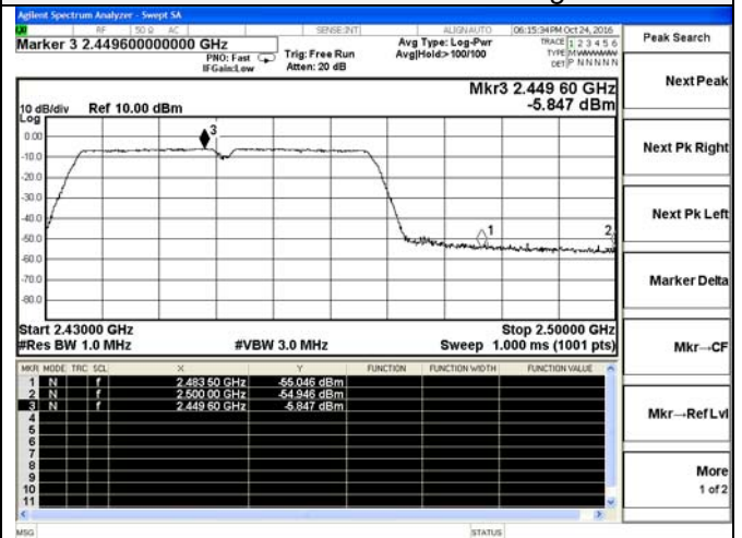
Channel 9 / 2452 MHz - Peak
