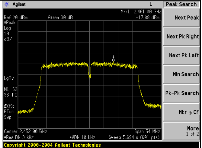
Channel 9 / 2452 MHz
