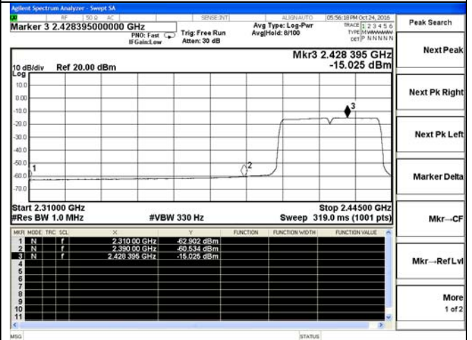
Channel 3 / 2422 MHz - Average
