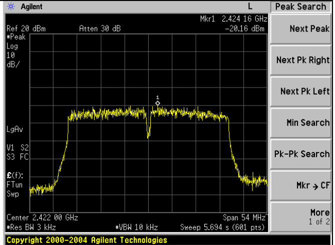
Channel 3 / 2422 MHz
