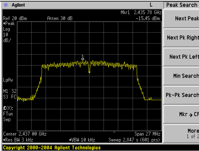
Channel 6 / 2437 MHz
