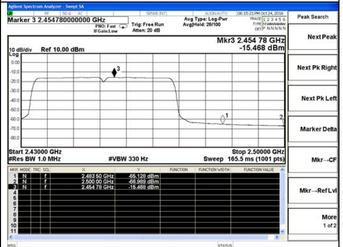
Channel 9 / 2452 MHz - Average
