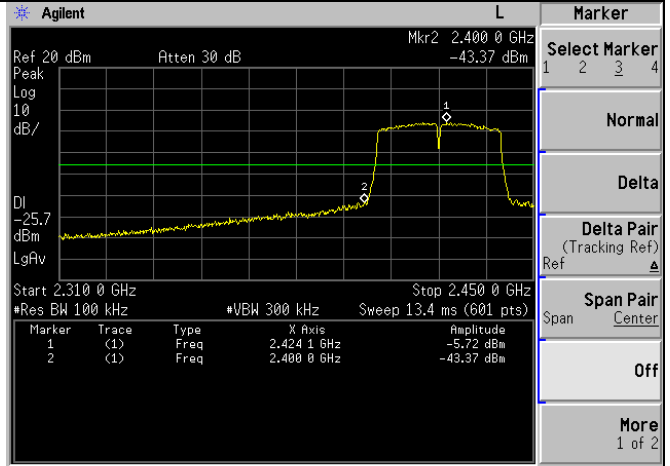
Channel 3 / 2422 MHz
