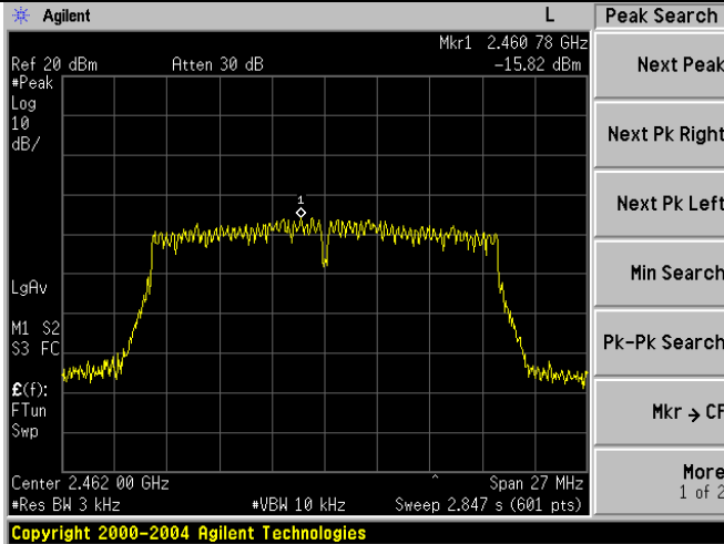
Channel 11 / 2462 MHz
