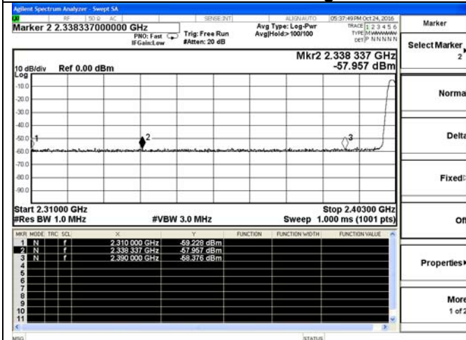
Channel 00 / 2402 MHz – Peak
