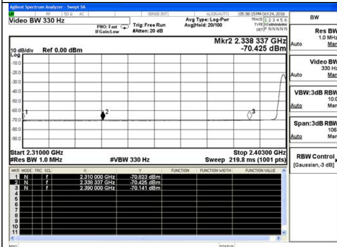
Channel 00 / 2402 MHz – Average
