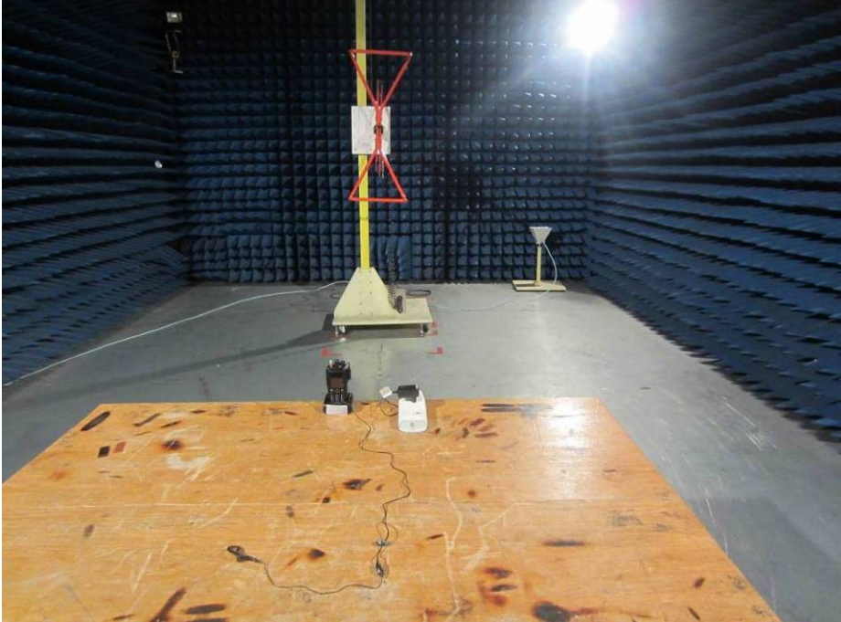
Radiated emission test
