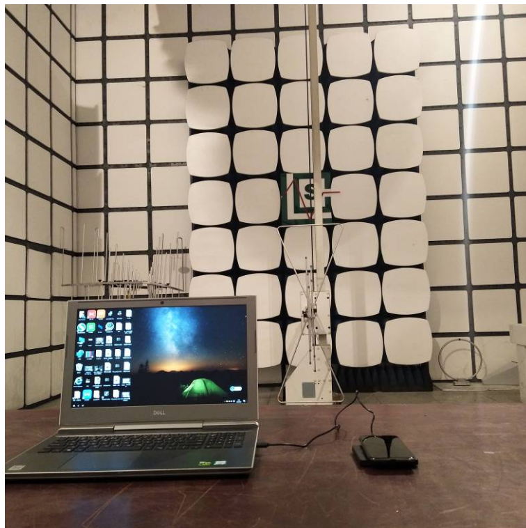
Radiated Emission below 1GHz-PC charge mode
