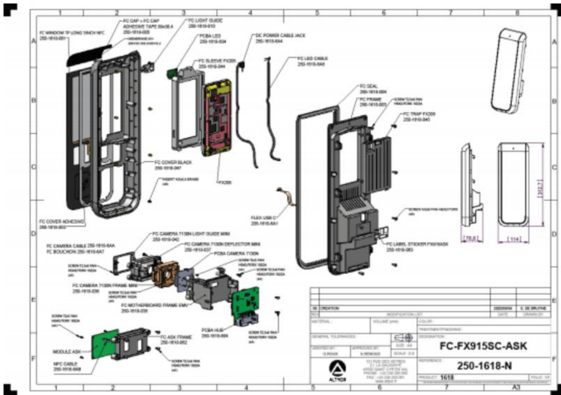
Figure 3: Front Casing FX915SC-ASK – NFC Android Validator
