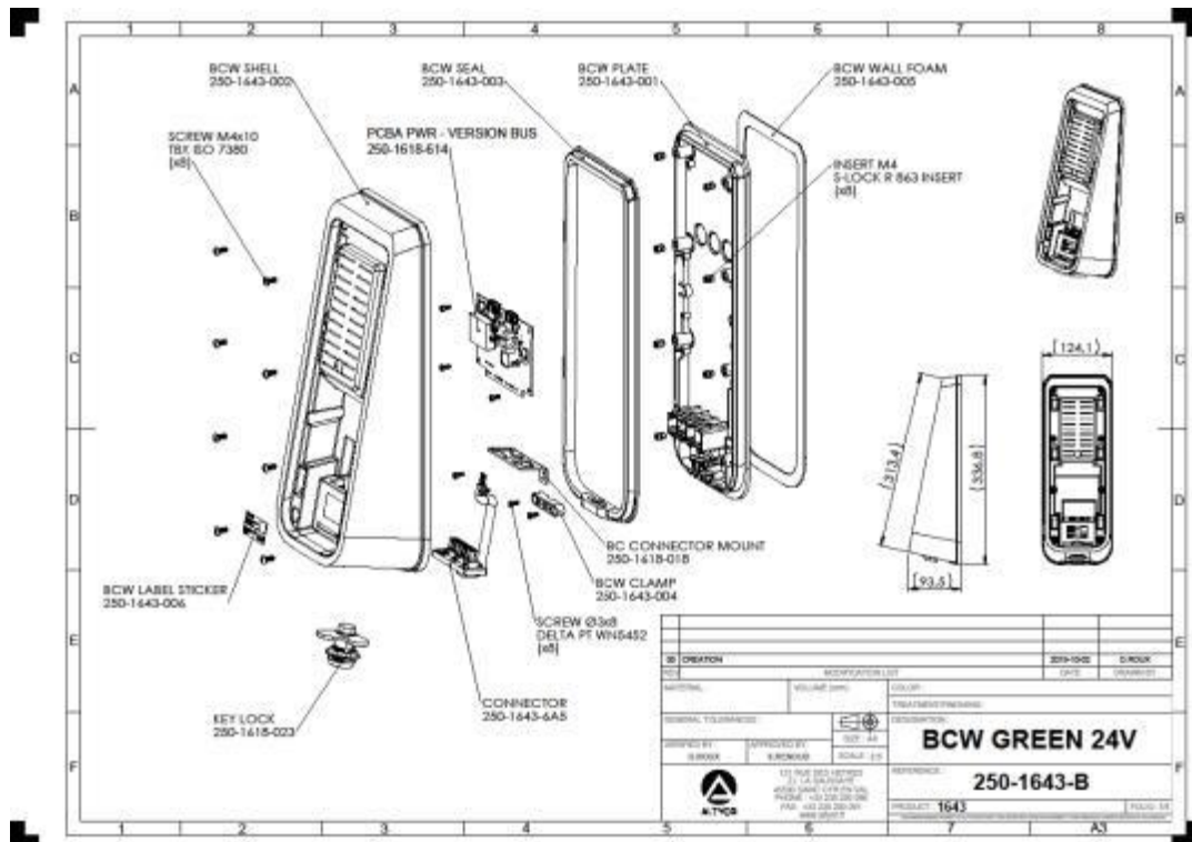
Figure 2:Back Casing Wall – NFC Android Validator
