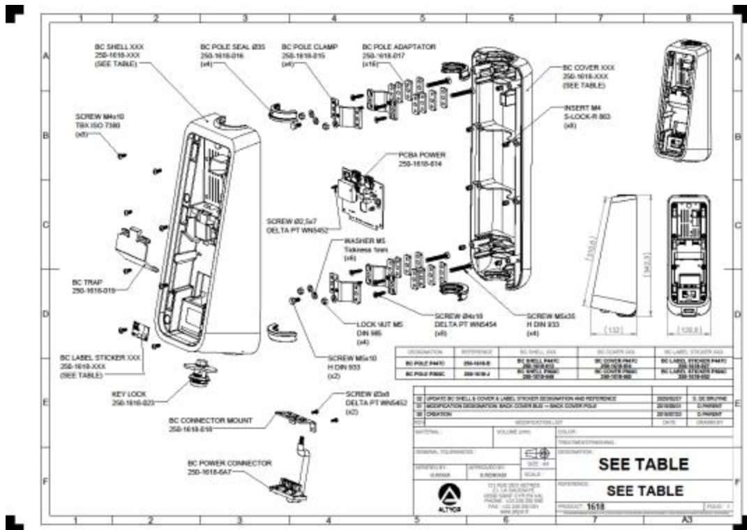
Figure 1:Back Casing Pole – NFC Android Validator
