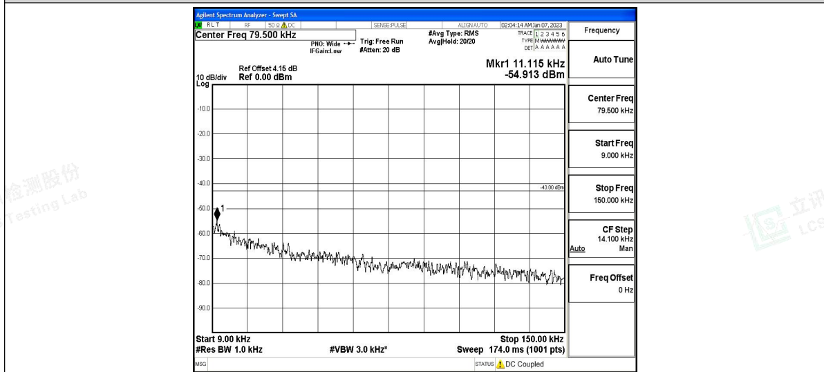
Band2-15MHz-16QAM-19125-1RB#0-Range2:0.15~30MHz
