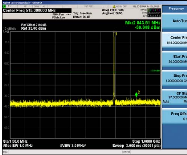
Band12_1.4MHz_QPSK_23017_1RB#0
