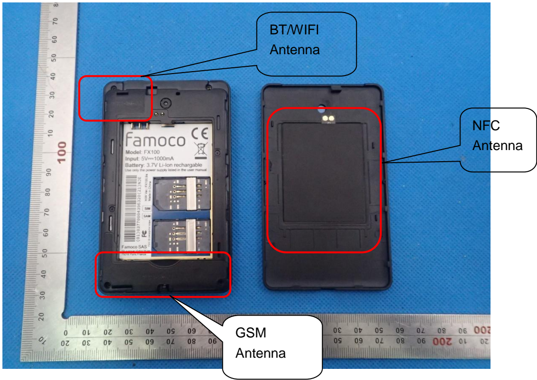
OPEN VIEW OF EUT(FIGURE 1)
