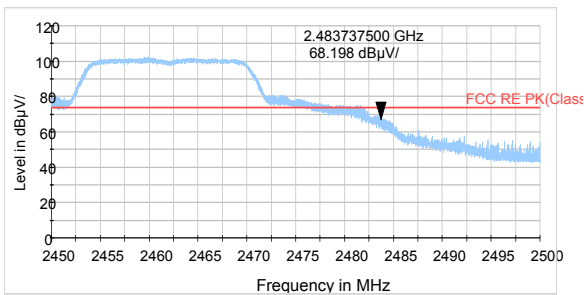
802.11g-Channel 11 Peak
