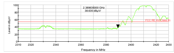
802.11b-Channel 1 Average
