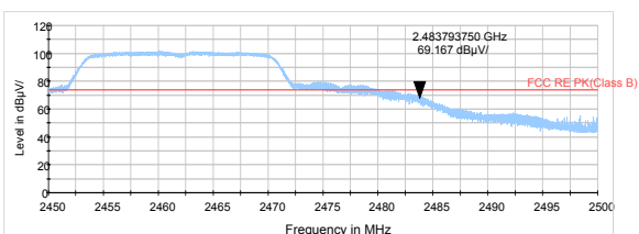
802.11n HT20 -Channel 11 Peak
