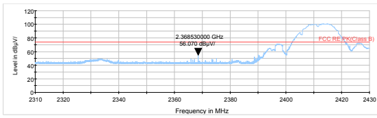
802.11b-Channel 1 Peak
