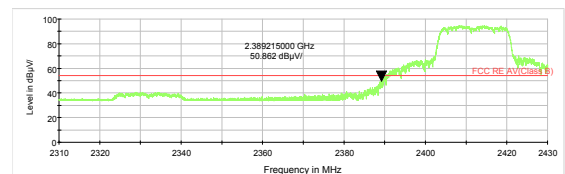
802.11g-Channel 1 Average
