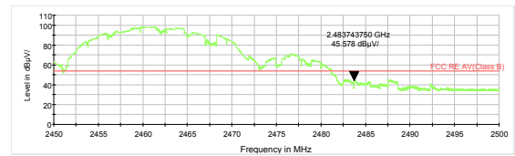
802.11b-Channel 11 Average
