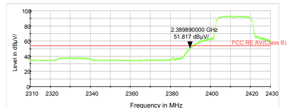
802.11n HT20 -Channel 1 Average
