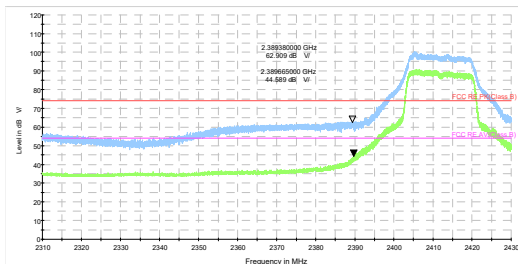
802.11g-Channel 1 Peak+ Average
