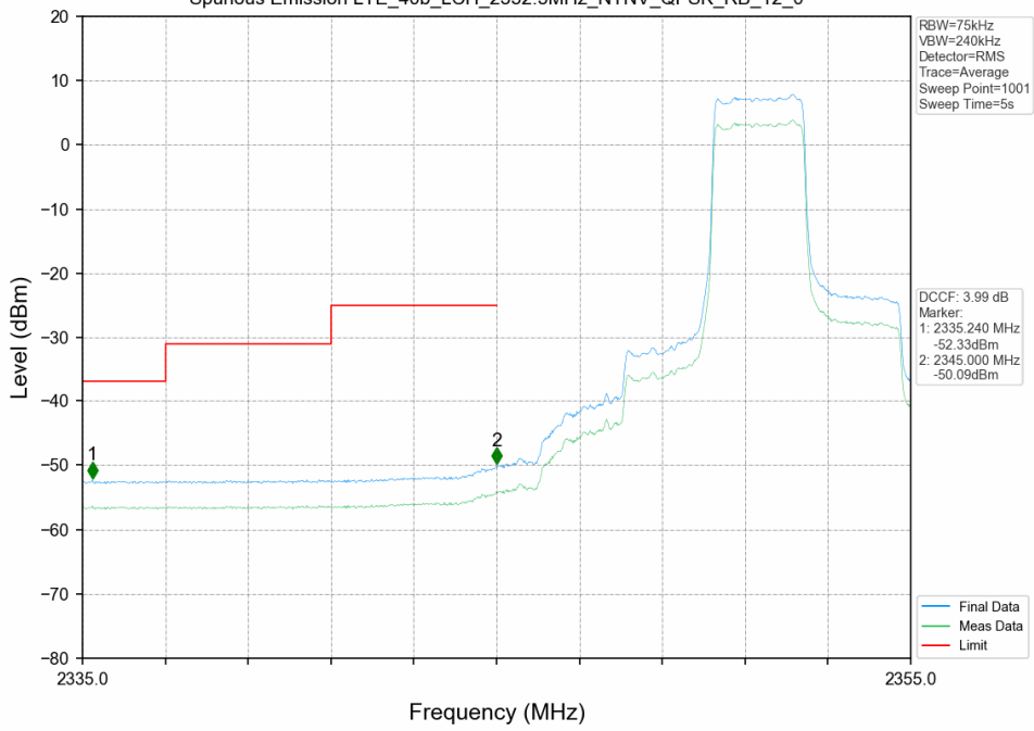
Spurious Emission LTE_40b_LCH_2352.5MHz_NTNV_QPSK_RB_12_0
