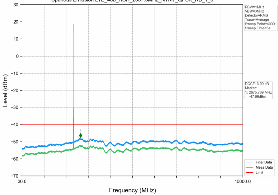
Spurious Emission LTE_40b_HCH_2357.5MHz_NTNV_QPSK_RB_1_0
