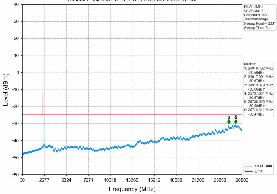
Spurious Emission LTE_7_LTE_LCH_2507.5MHz_NTNV
