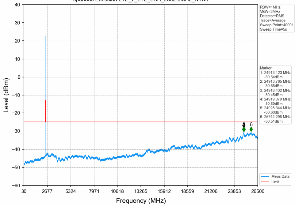
Spurious Emission LTE_7_LTE_LCH_2502.5MHz_NTNV
