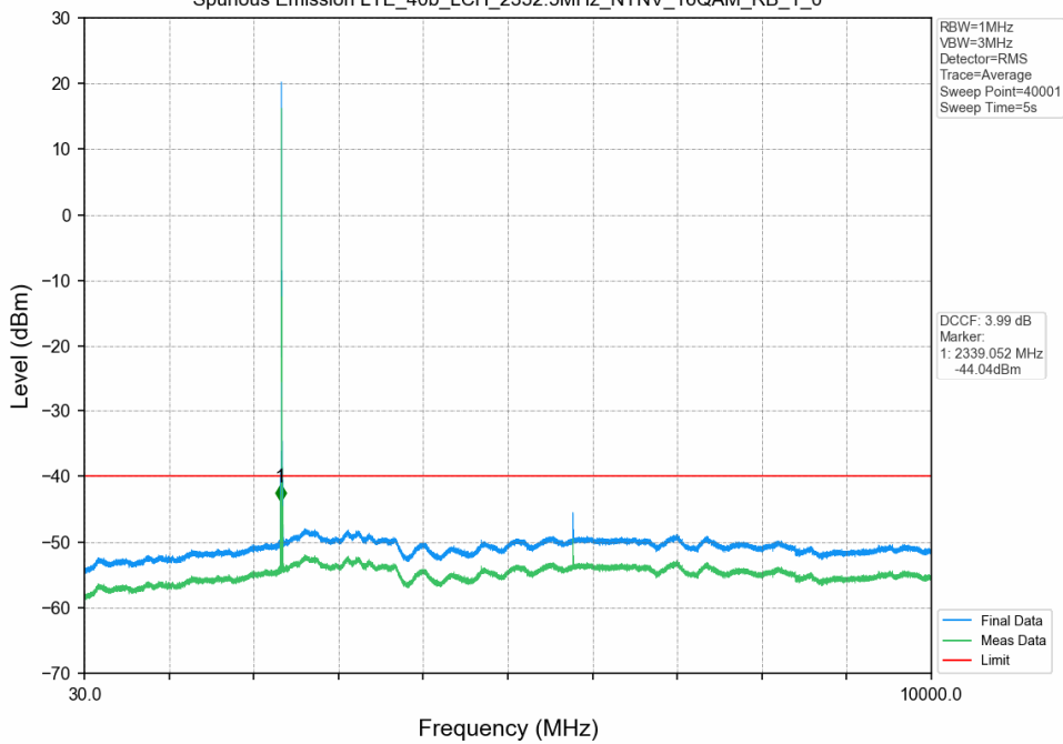
Spurious Emission LTE_40b_LCH_2352.5MHz_NTNV_16QAM_RB_1_0
