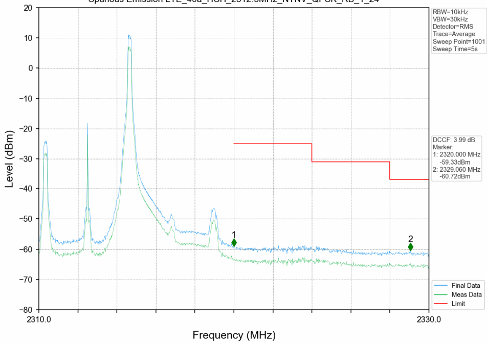
Spurious Emission LTE_40a_HCH_2312.5MHz_NTNV_QPSK_RB_1_24
