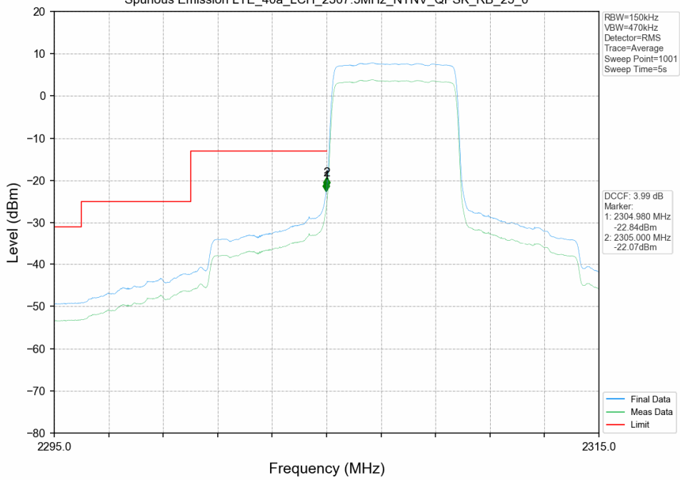
Spurious Emission LTE_40a_LCH_2307.5MHz_NTNV_QPSK_RB_25_0
