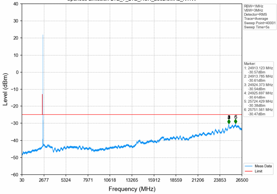
Spurious Emission LTE_7_LTE_HCH_2562.5MHz_NTNV
