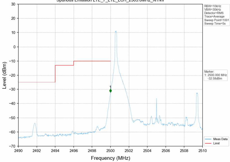
Spurious Emission LTE_7_LTE_LCH_2505.0MHz_NTNV
