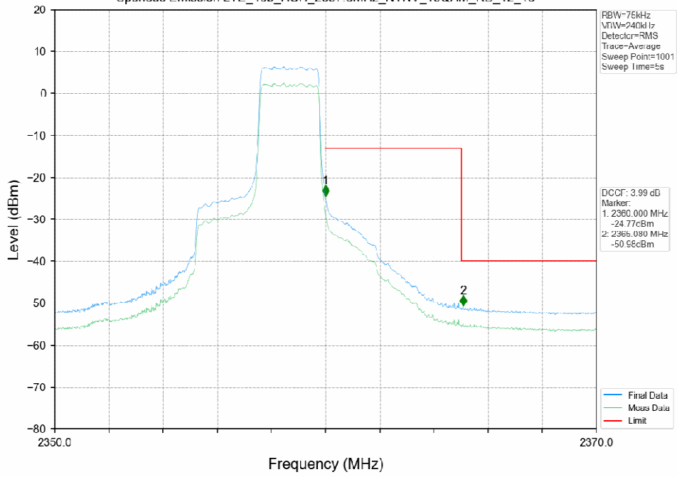
Spurious Emission LTE_40b_HCH_2357.5MHz_NTNV_16QAM_RB_12_13
