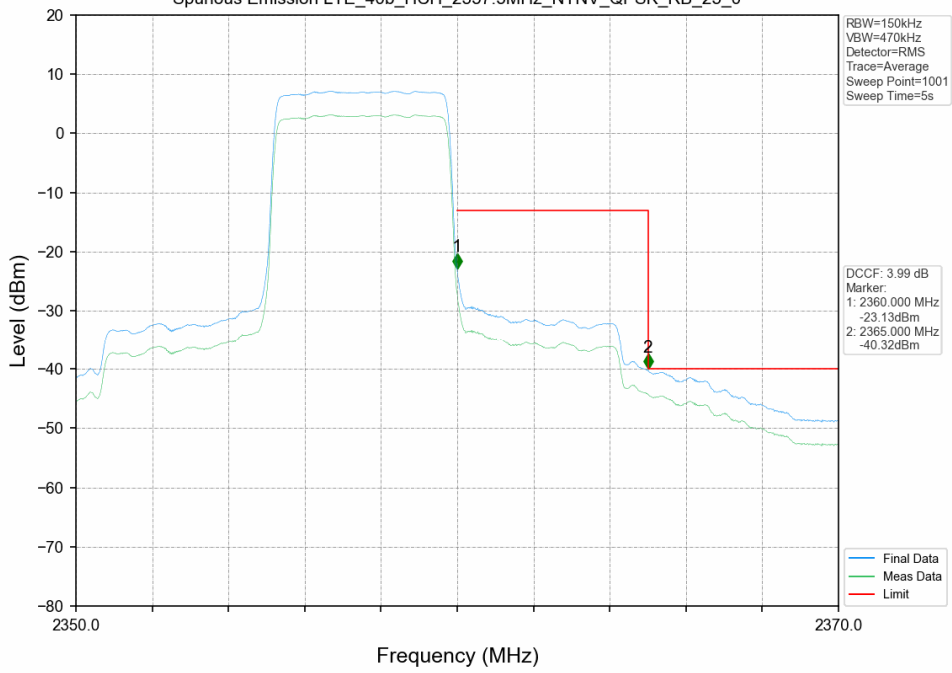
Spurious Emission LTE_40b_HCH_2357.5MHz_NTNV_QPSK_RB_25_0
