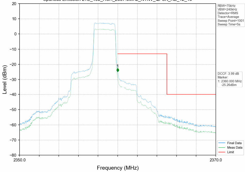
Spurious Emission LTE_40b_HCH_2357.5MHz_NTNV_QPSK_RB_12_13
