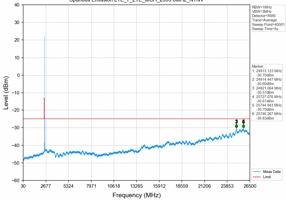
Spurious Emission LTE_7_LTE_MCH_2535.0MHz_NTNV
