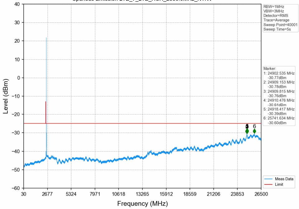
Spurious Emission LTE_7_LTE_HCH_2560.0MHz_NTNV
