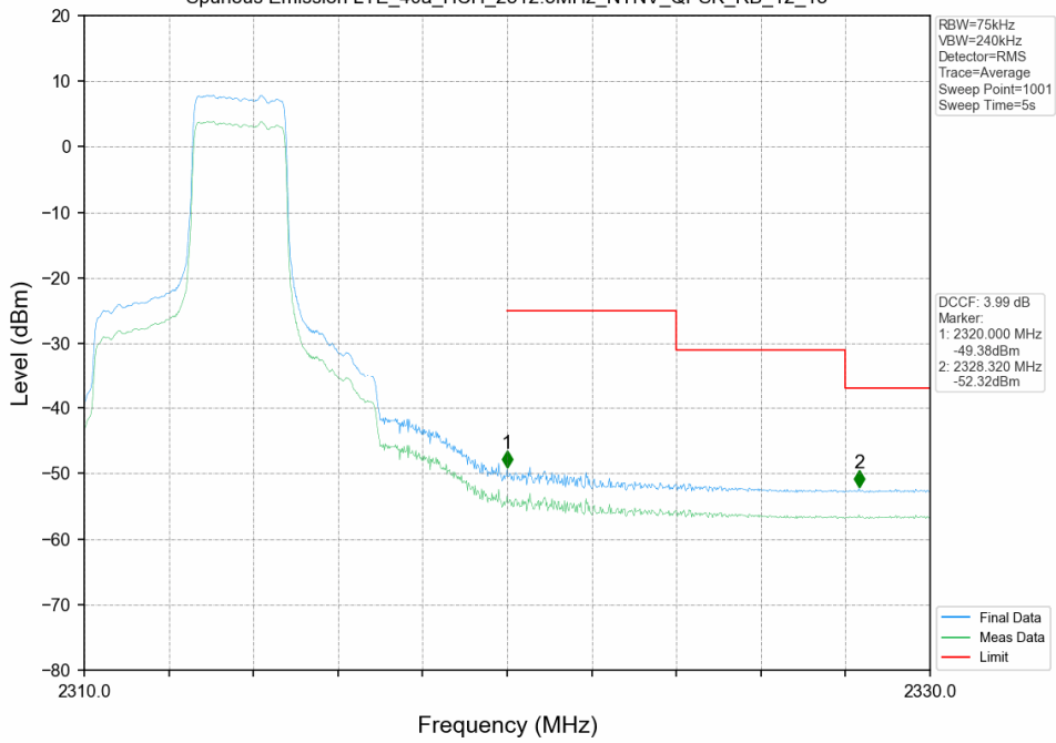
Spurious Emission LTE_40a_HCH_2312.5MHz_NTNV_QPSK_RB_12_13
