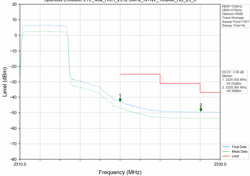
Spurious Emission LTE_40a_HCH_2312.5MHz_NTNV_16QAM_RB_25_0
