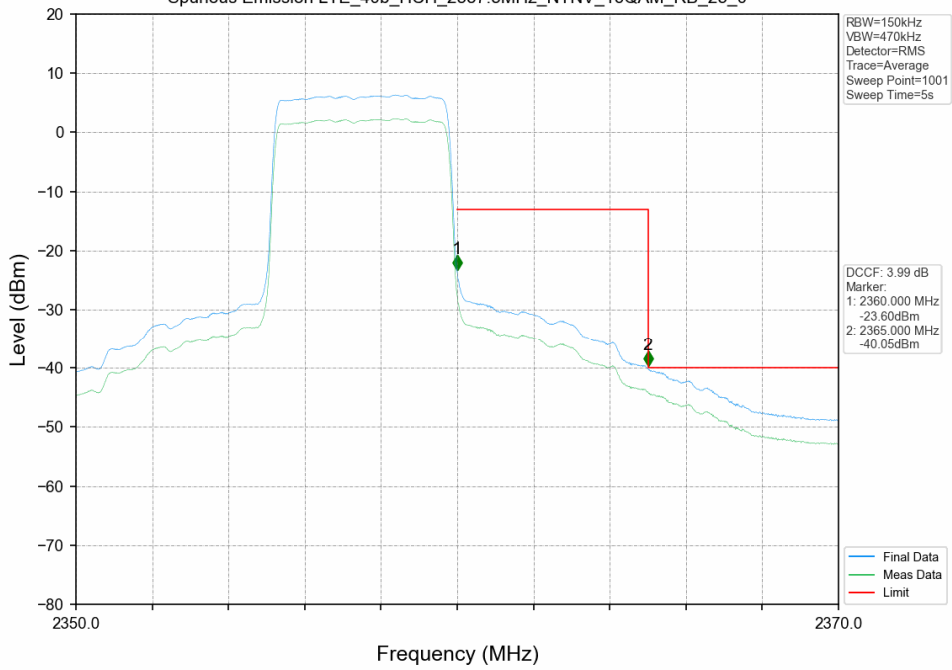
Spurious Emission LTE_40b_HCH_2357.5MHz_NTNV_16QAM_RB_25_0
