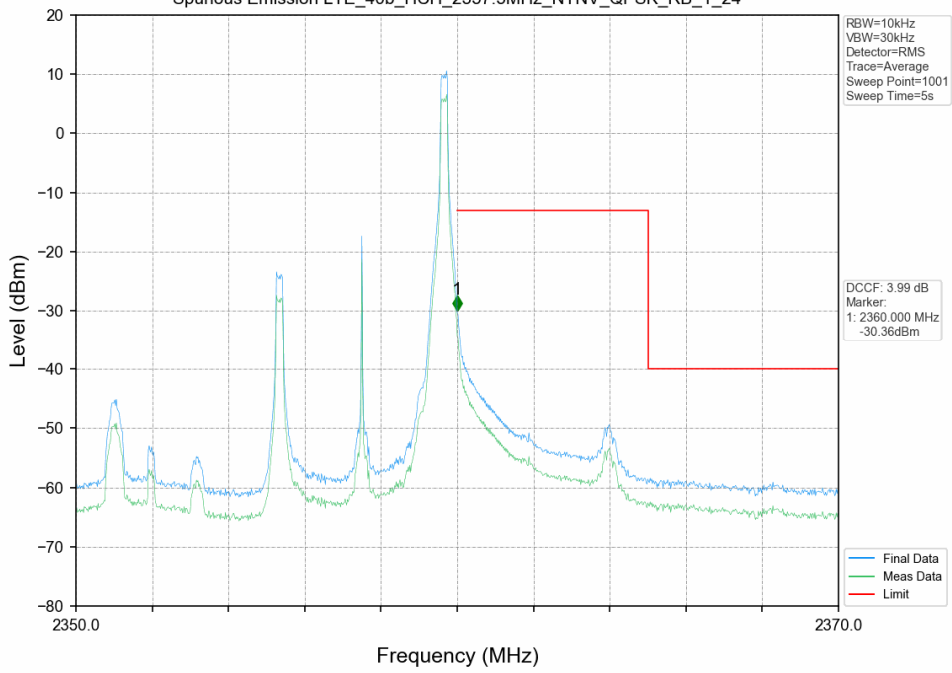
Spurious Emission LTE_40b_HCH_2357.5MHz_NTNV_QPSK_RB_1_24
