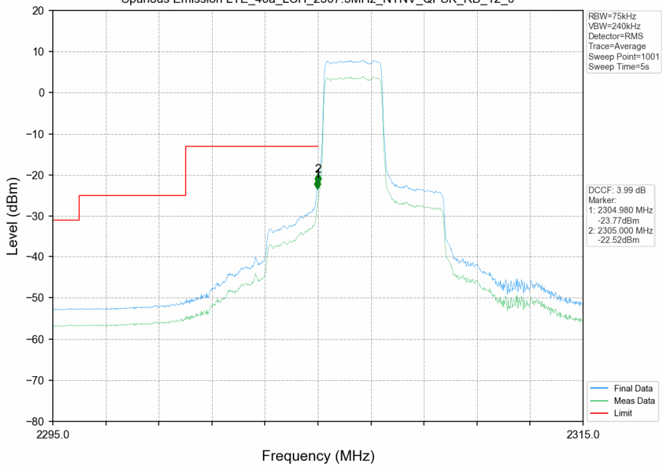
Spurious Emission LTE_40a_LCH_2307.5MHz_NTNV_QPSK_RB_12_0
