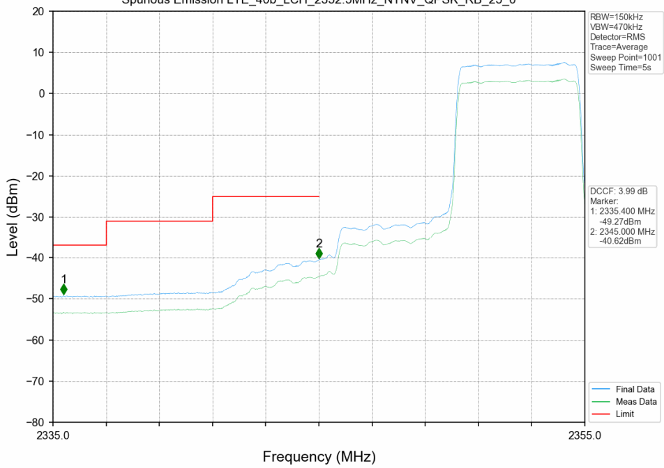
Spurious Emission LTE_40b_LCH_2352.5MHz_NTNV_QPSK_RB_25_0
