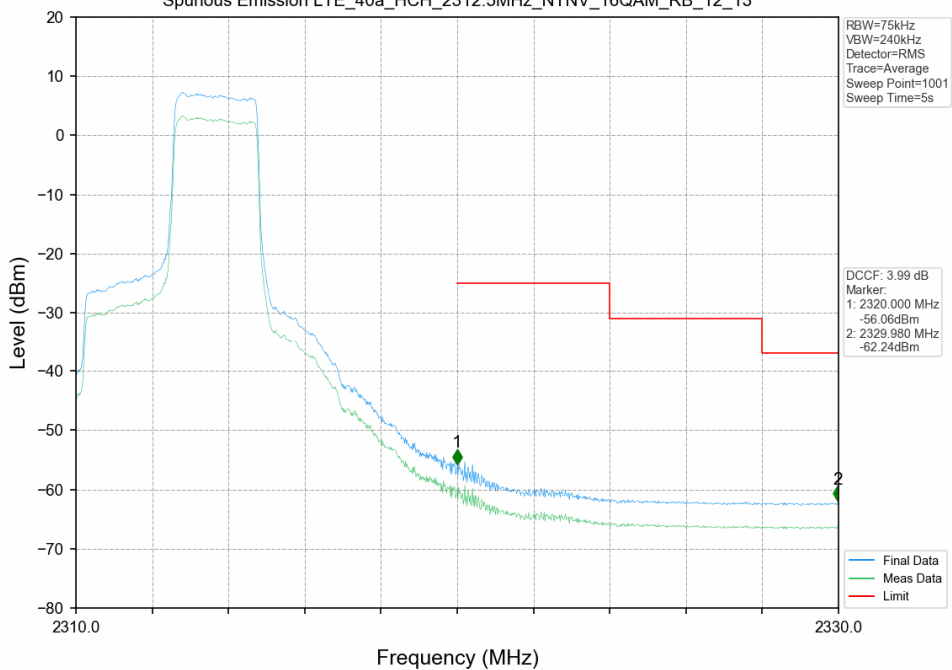
Spurious Emission LTE_40a_HCH_2312.5MHz_NTNV_16QAM_RB_12_13
