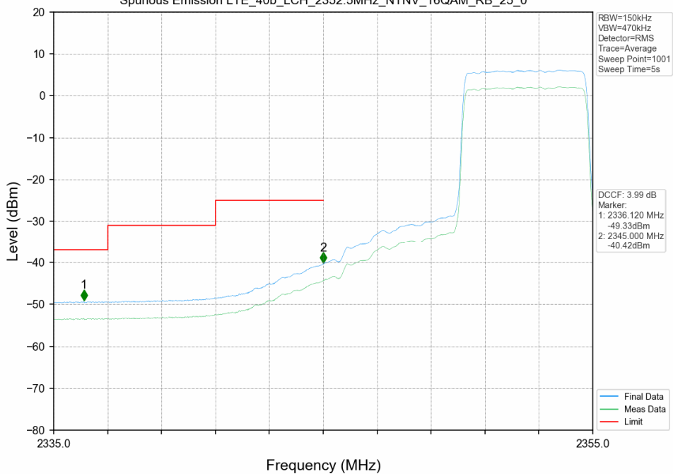
Spurious Emission LTE_40b_LCH_2352.5MHz_NTNV_16QAM_RB_25_0
