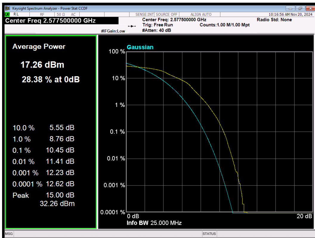
LTE Band38 16QAM BW=15MHz Channel=37825 RB Size=75 Position=#0
