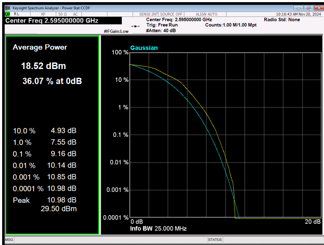
LTE Band38 16QAM BW=10MHz Channel=38000 RB Size=50 Position=#0
