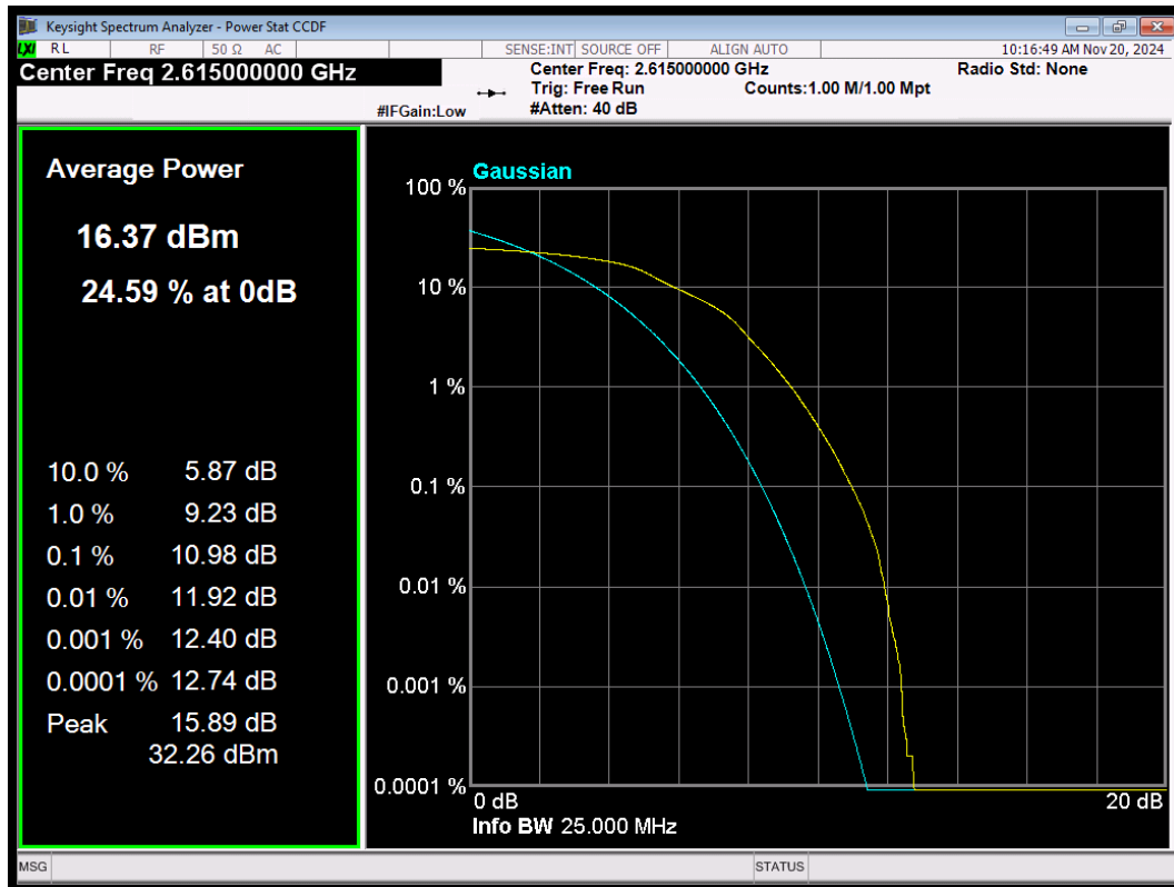
LTE Band38 16QAM BW=10MHz Channel=38200 RB Size=50 Position=#0
