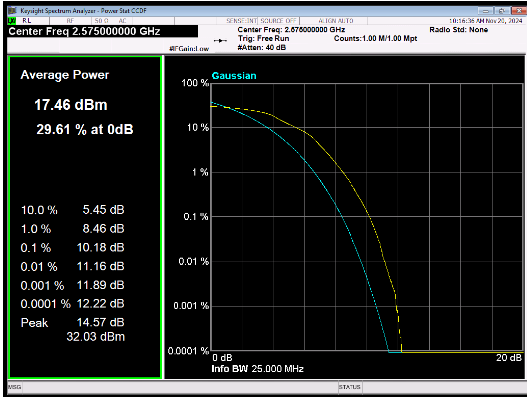
LTE Band38 16QAM BW=10MHz Channel=37800 RB Size=50 Position=#0
