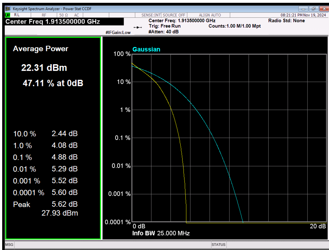
LTE Band25 QPSK BW=3MHz Channel=26675 RB Size=15 Position=#0
