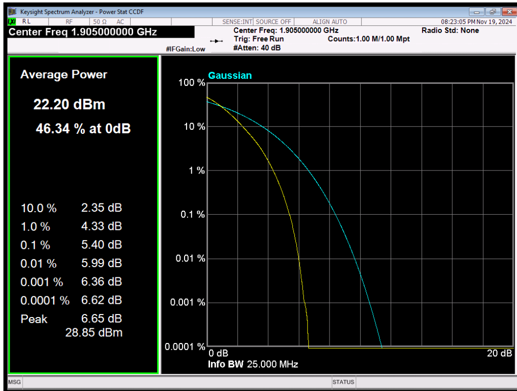
LTE Band25 QPSK BW=20MHz Channel=26590 RB Size=100 Position=#0
