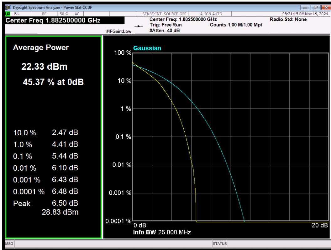
LTE Band25 QPSK BW=3MHz Channel=26365 RB Size=15 Position=#0
