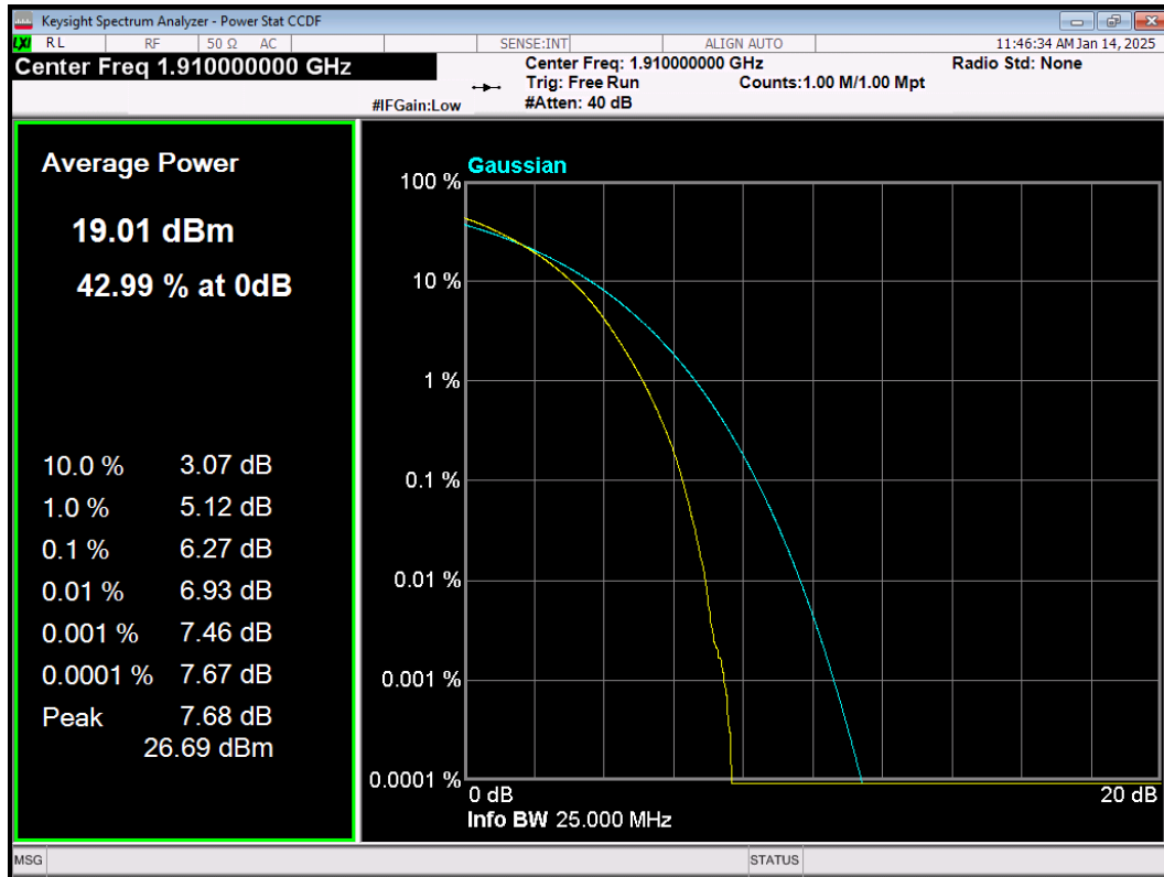
LTE Band25 64QAM BW=10MHz Channel=26640 RB Size=50 Position=#0
