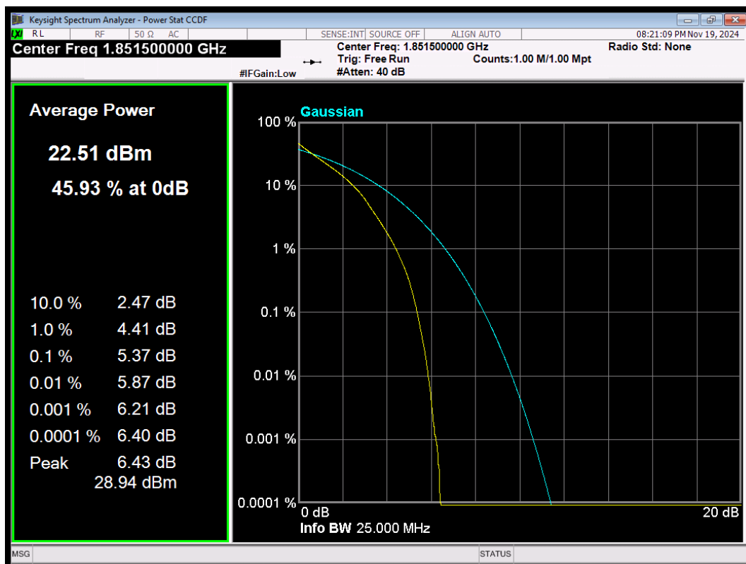
LTE Band25 QPSK BW=3MHz Channel=26055 RB Size=15 Position=#0
