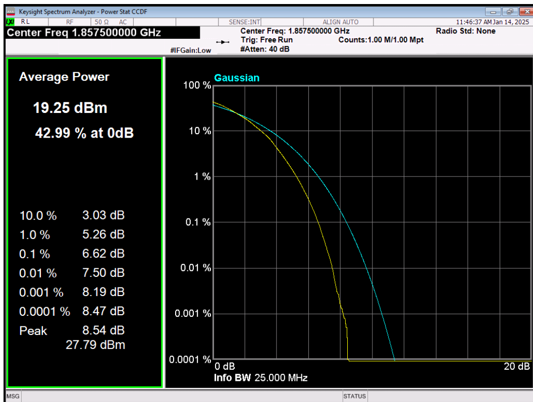
LTE Band25 64QAM BW=15MHz Channel=26115 RB Size=75 Position=#0
