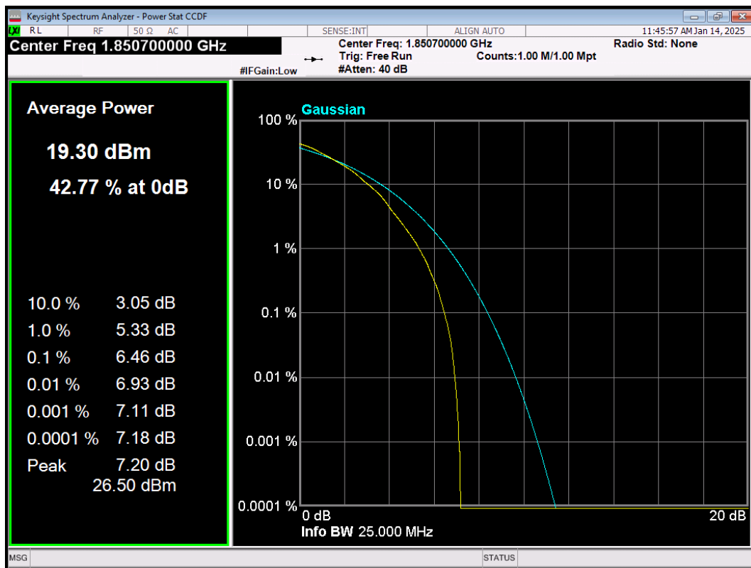
LTE Band25 64QAM BW=1.4MHz Channel=26047 RB Size=6 Position=#0
