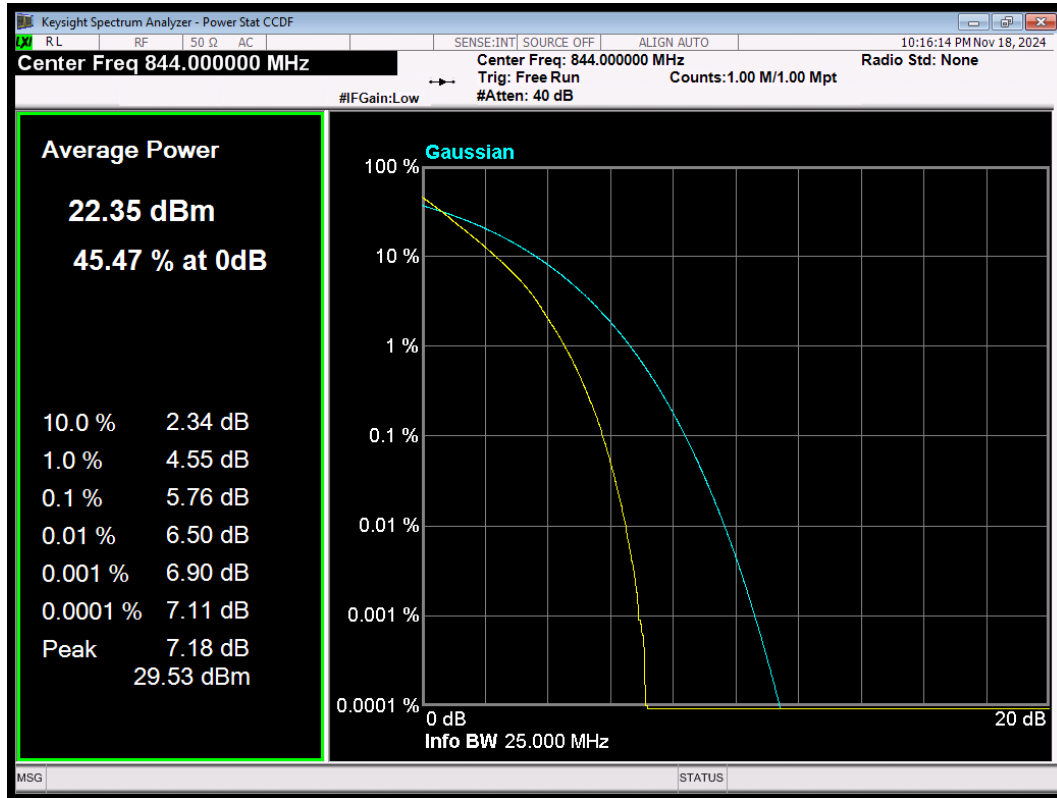
LTE Band5 QPSK BW=10MHz Channel=20600 RB Size=50 Position=#0
