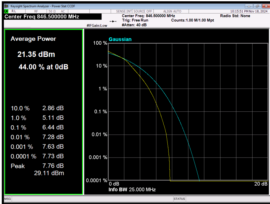
LTE Band5 16QAM BW=5MHz Channel=20625 RB Size=25 Position=#0
