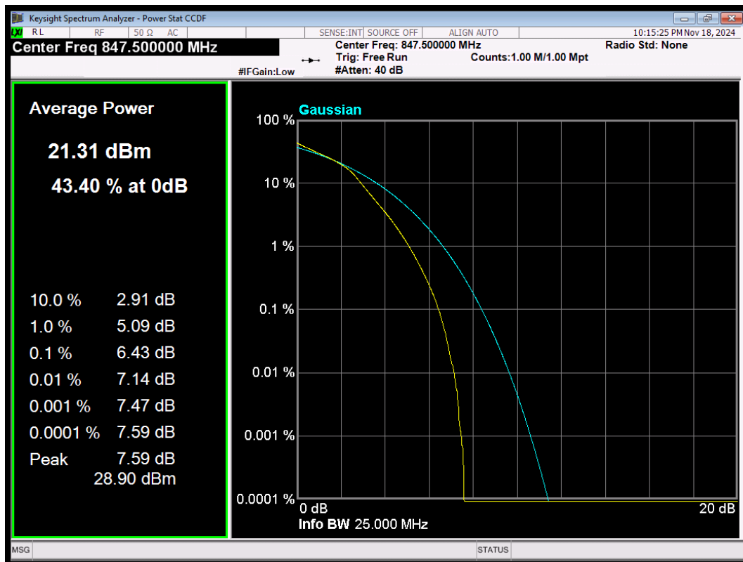
LTE Band5 16QAM BW=3MHz Channel=20635 RB Size=15 Position=#0
