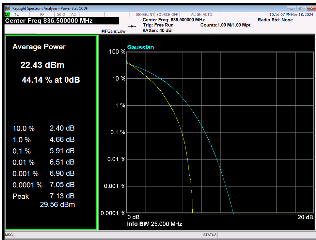
LTE Band5 QPSK BW=10MHz Channel=20525 RB Size=50 Position=#0
