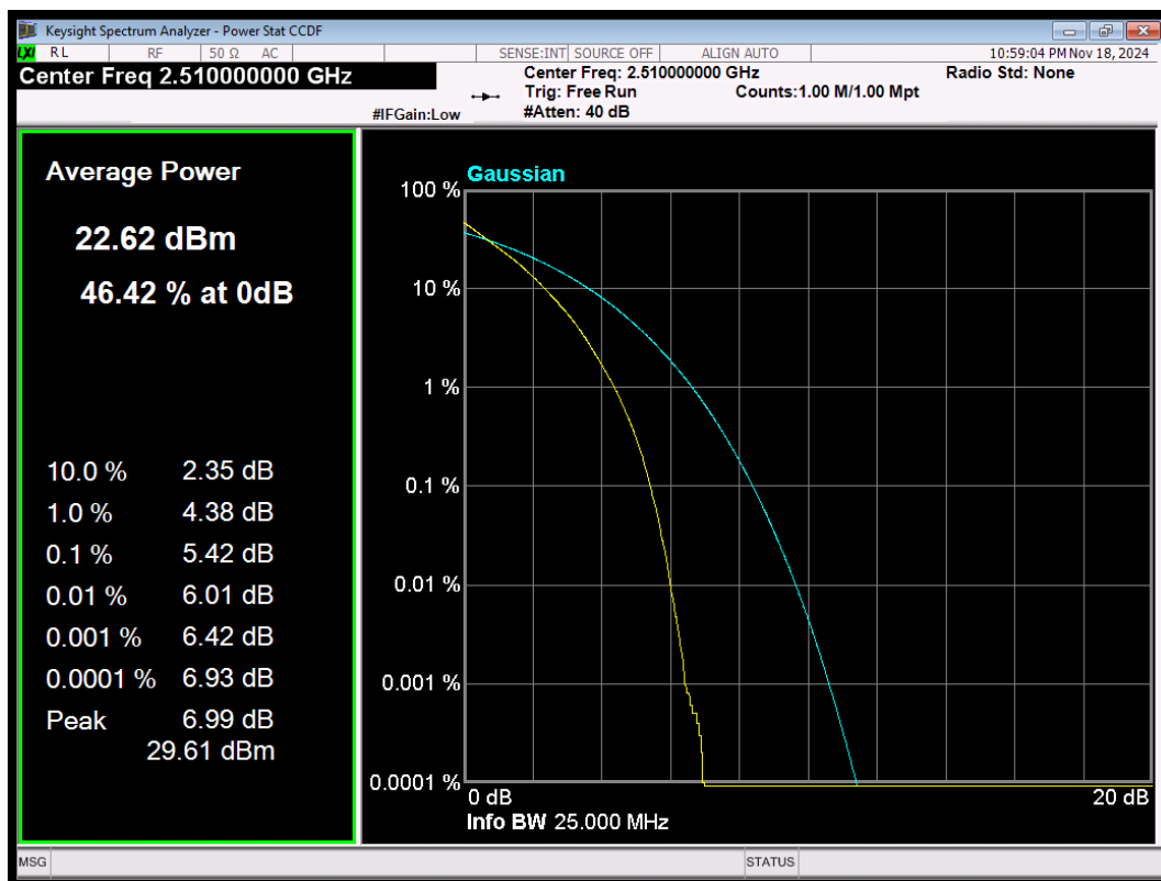
LTE Band7 QPSK BW=20MHz Channel=20850 RB Size=100 Position=#0
