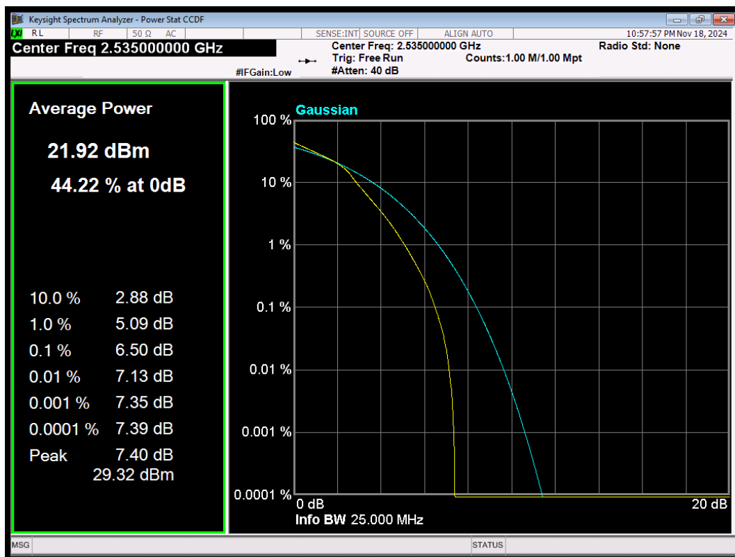
LTE Band7 16QAM BW=5MHz Channel=21100 RB Size=25 Position=#0
