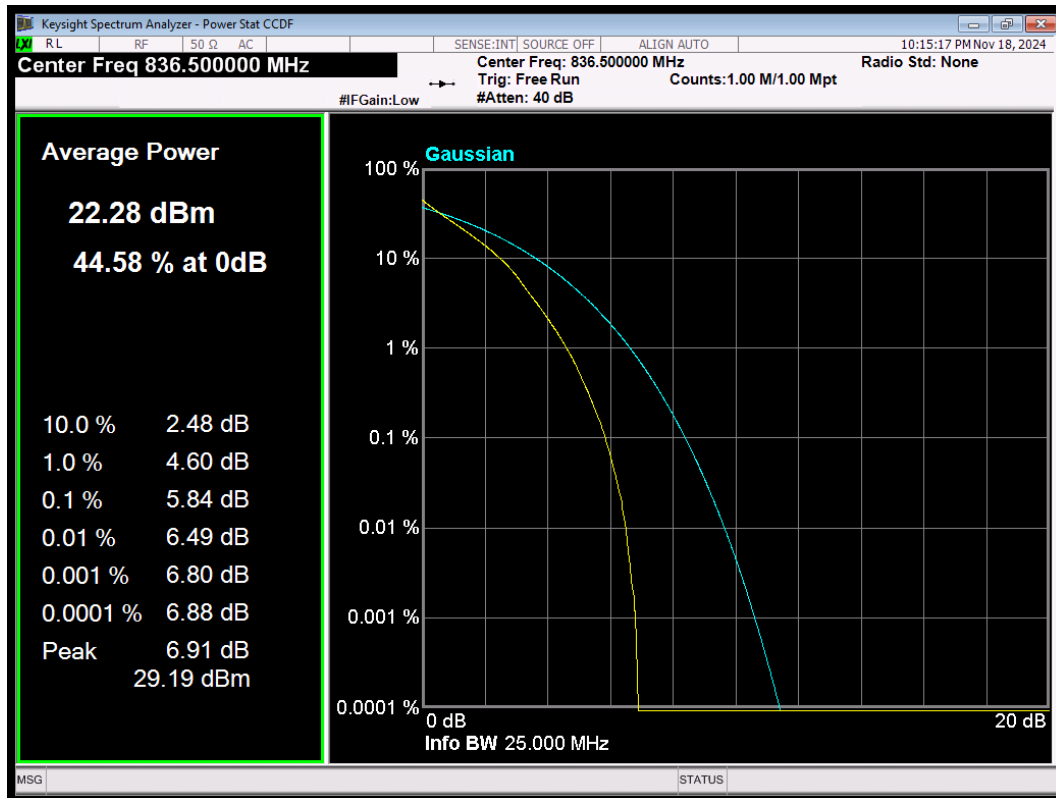
LTE Band5 QPSK BW=3MHz Channel=20525 RB Size=15 Position=#0
