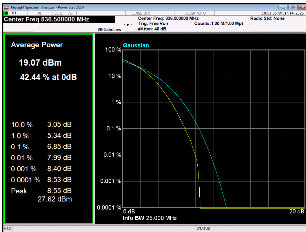
LTE Band5 64QAM BW=5MHz Channel=20525 RB Size=25 Position=#0
