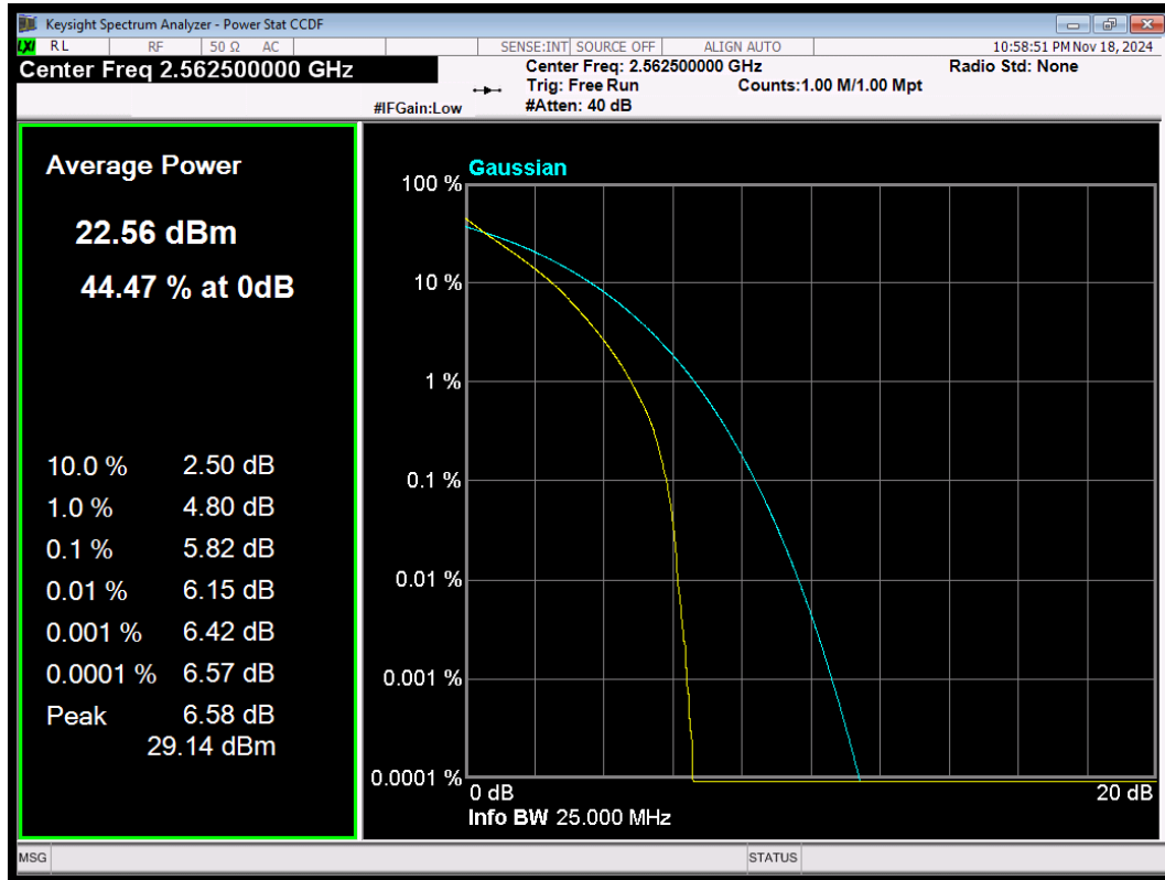
LTE Band7 QPSK BW=15MHz Channel=21375 RB Size=75 Position=#0
