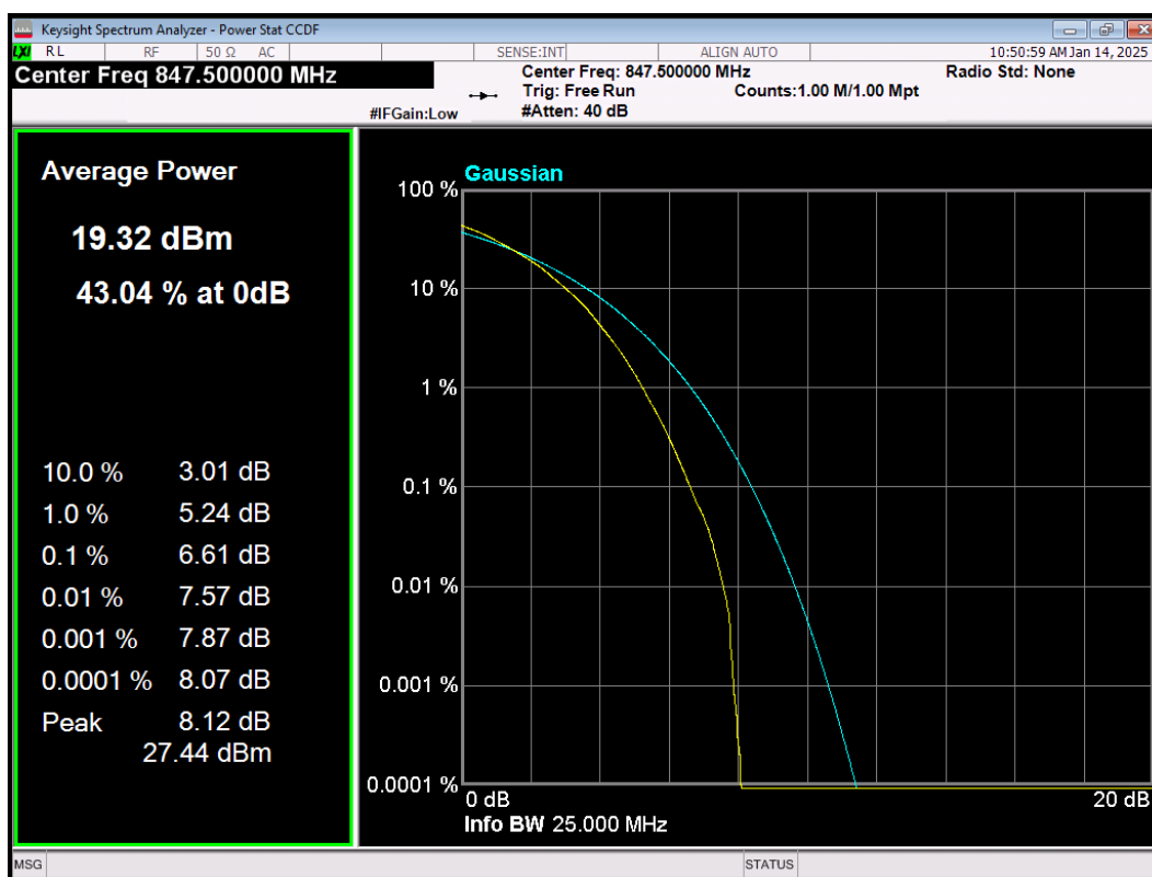
LTE Band5 64QAM BW=3MHz Channel=20635 RB Size=15 Position=#0
