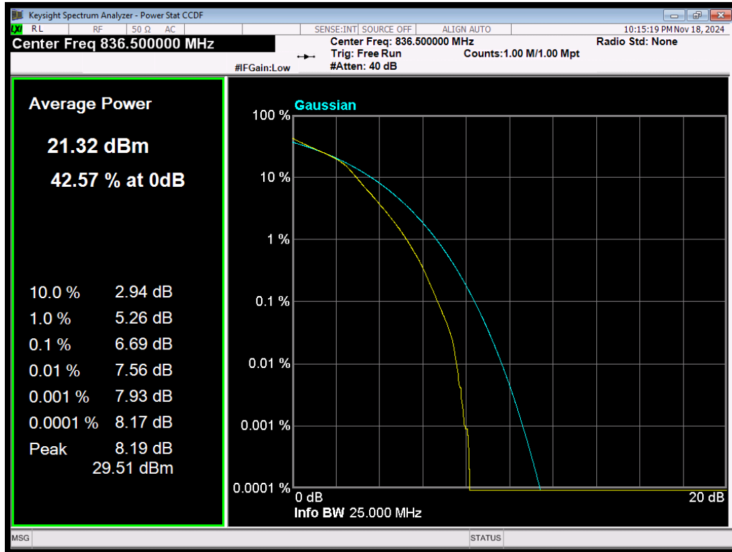
LTE Band5 16QAM BW=3MHz Channel=20525 RB Size=15 Position=#0
