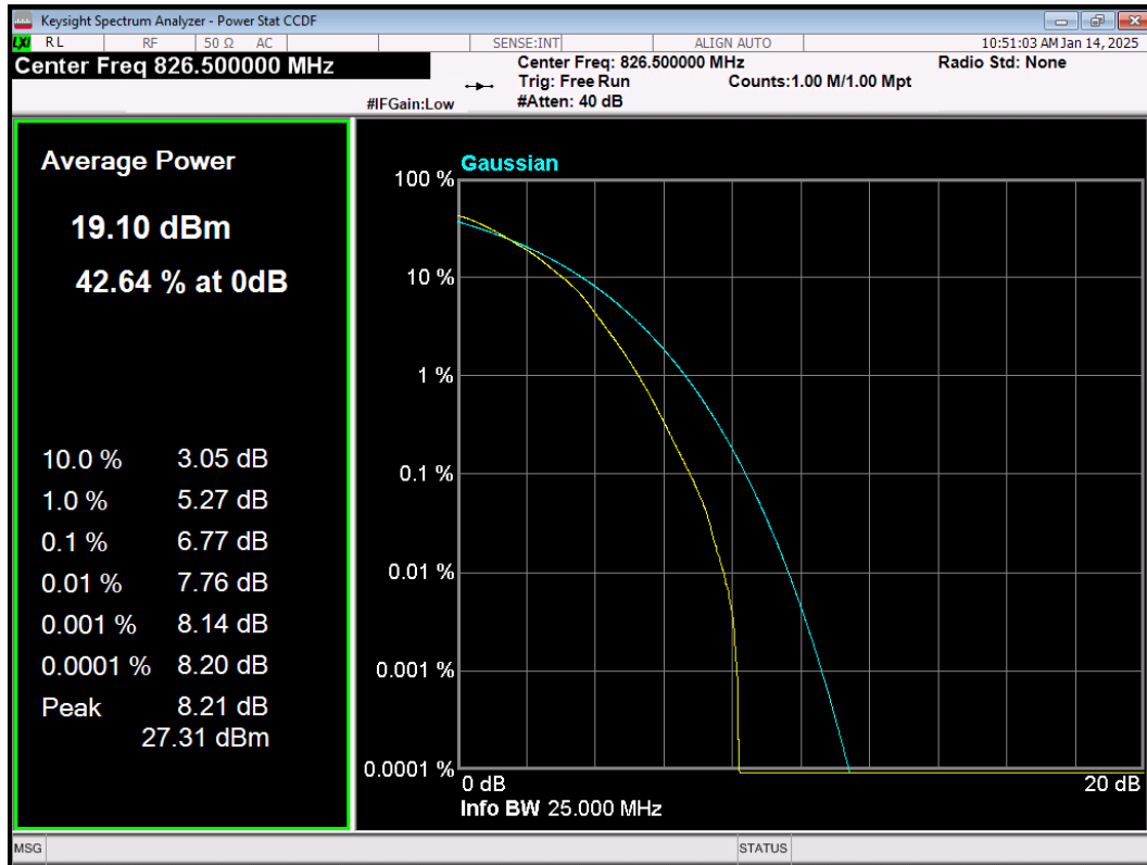
LTE Band5 64QAM BW=5MHz Channel=20425 RB Size=25 Position=#0
