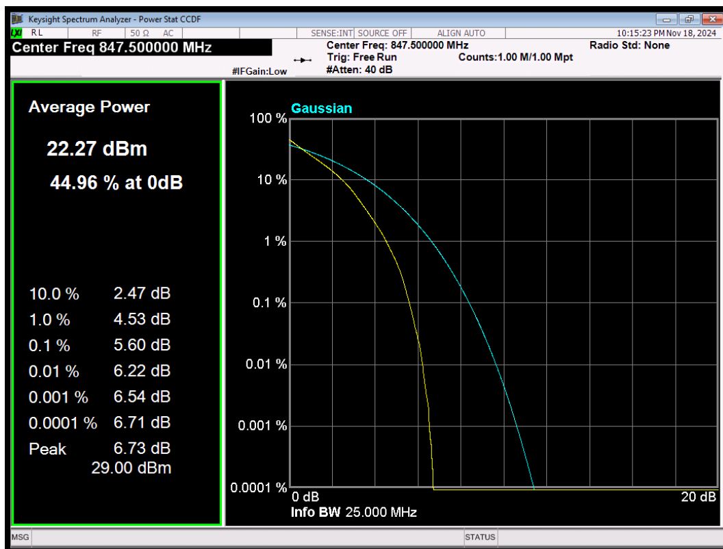
LTE Band5 QPSK BW=3MHz Channel=20635 RB Size=15 Position=#0
