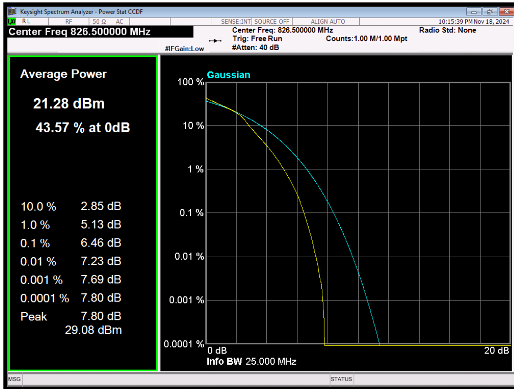
LTE Band5 16QAM BW=5MHz Channel=20425 RB Size=25 Position=#0
