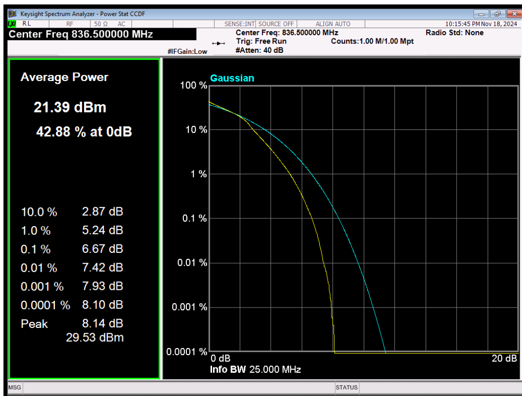
LTE Band5 16QAM BW=5MHz Channel=20525 RB Size=25 Position=#0
