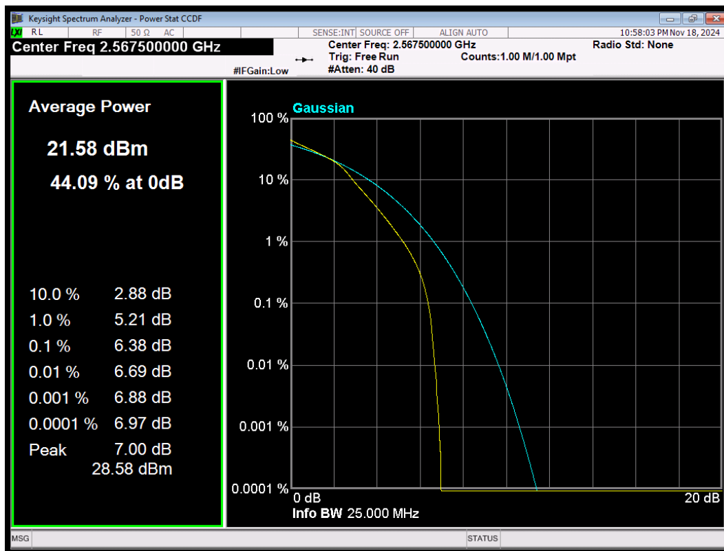
LTE Band7 16QAM BW=5MHz Channel=21425 RB Size=25 Position=#0
