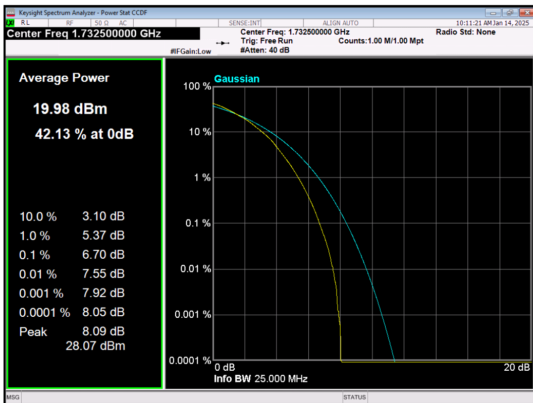
LTE Band4 64QAM BW=5MHz Channel=20175 RB Size=25 Position=#0
