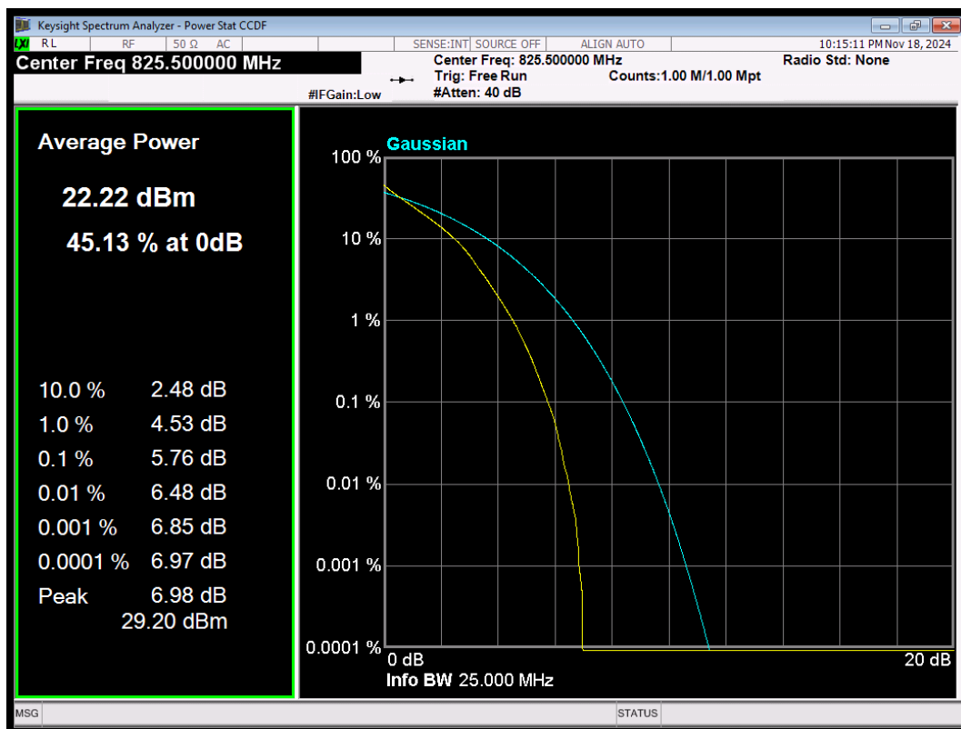
LTE Band5 QPSK BW=3MHz Channel=20415 RB Size=15 Position=#0
