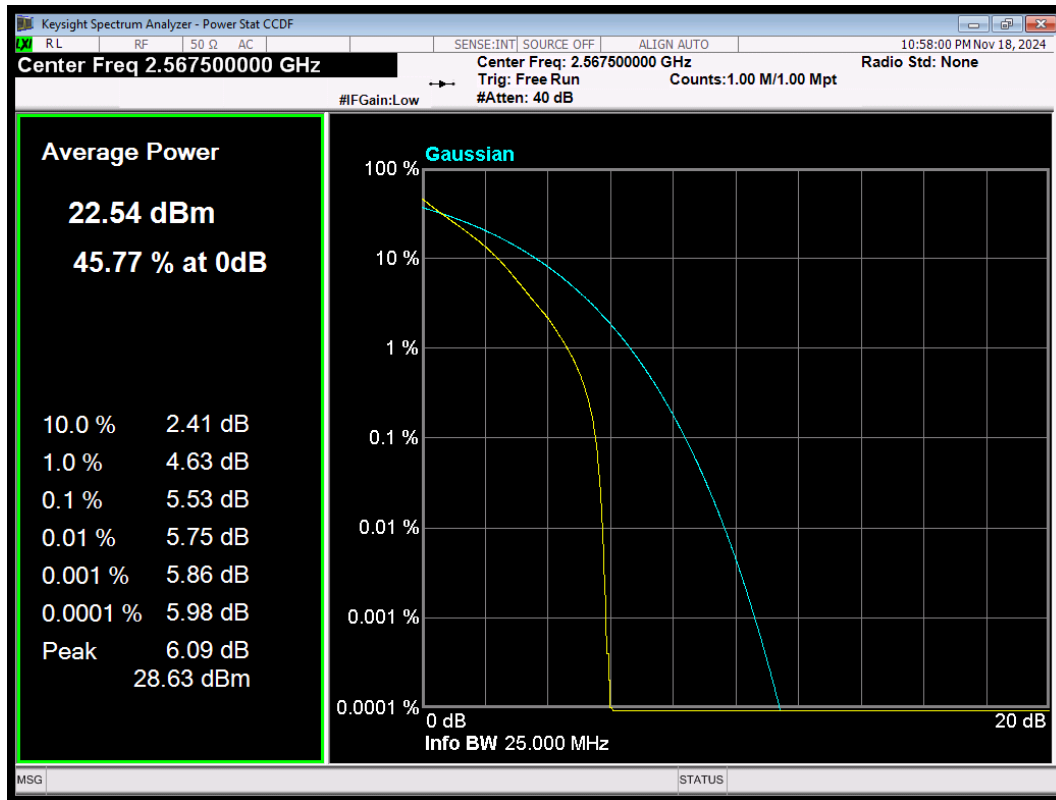
LTE Band7 QPSK BW=5MHz Channel=21425 RB Size=25 Position=#0
