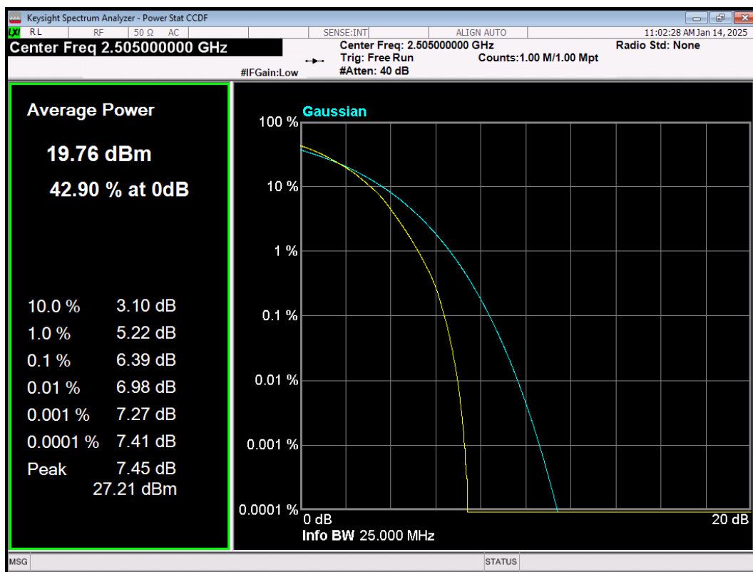
LTE Band7 64QAM BW=10MHz Channel=20800 RB Size=50 Position=#0
