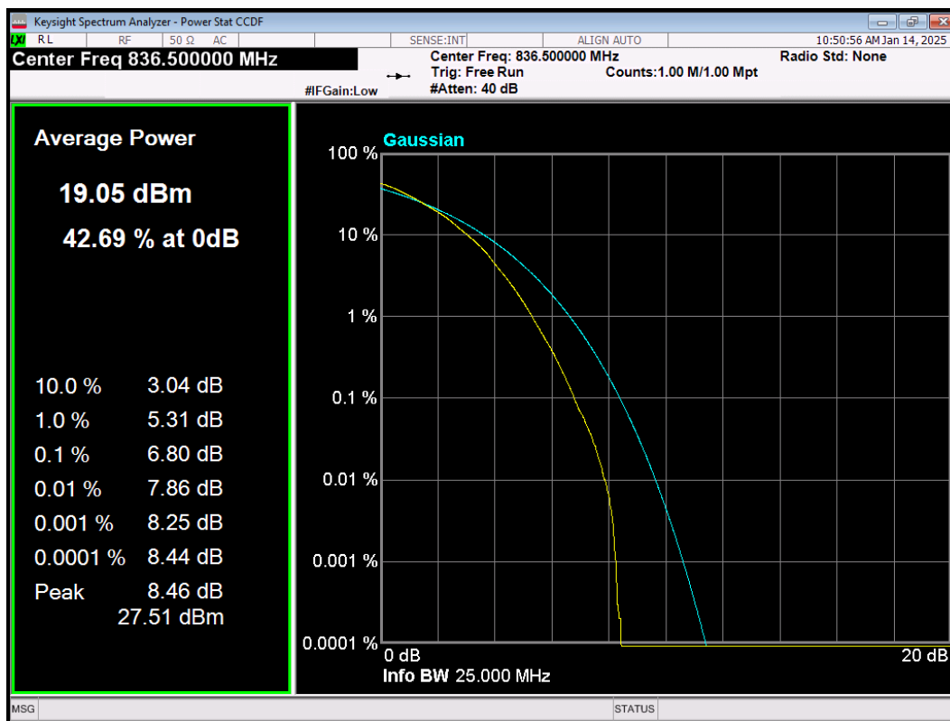
LTE Band5 64QAM BW=3MHz Channel=20525 RB Size=15 Position=#0
