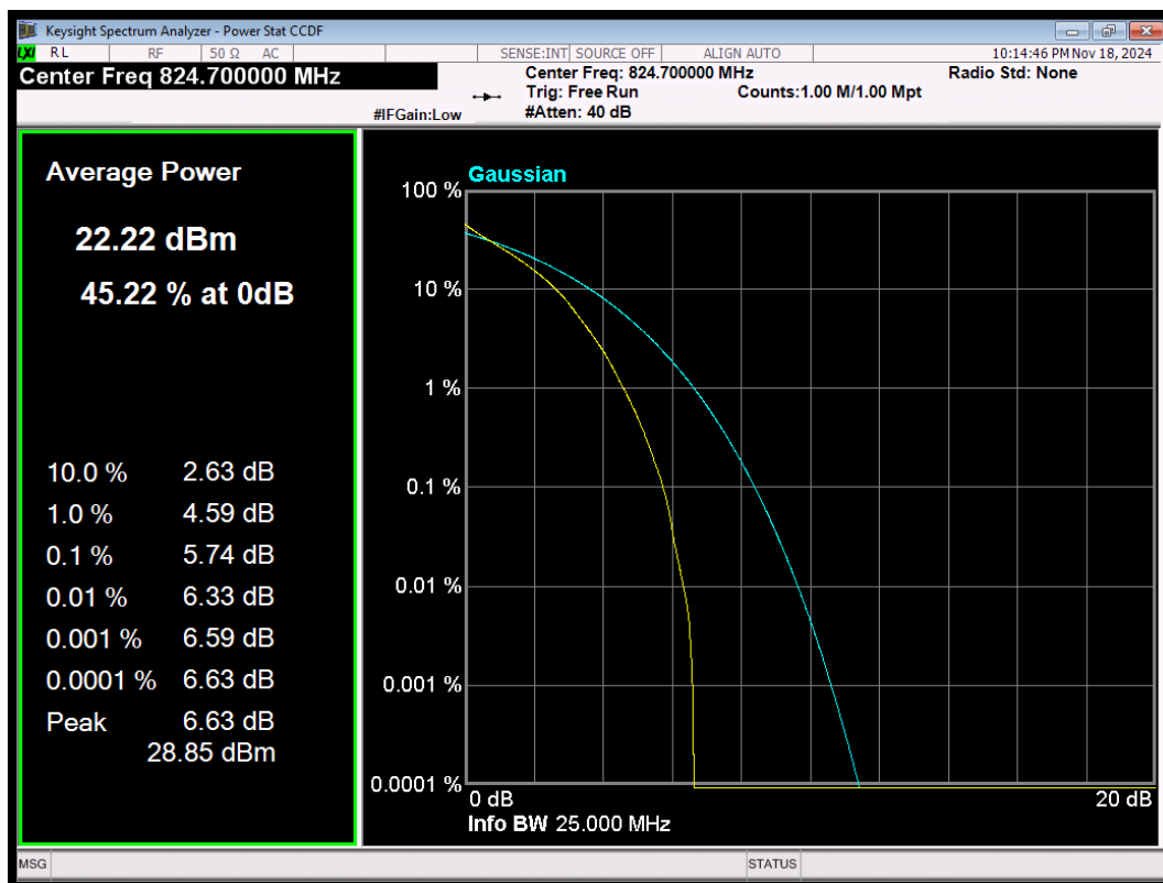
LTE Band5 QPSK BW=1.4MHz Channel=20407 RB Size=6 Position=#0
