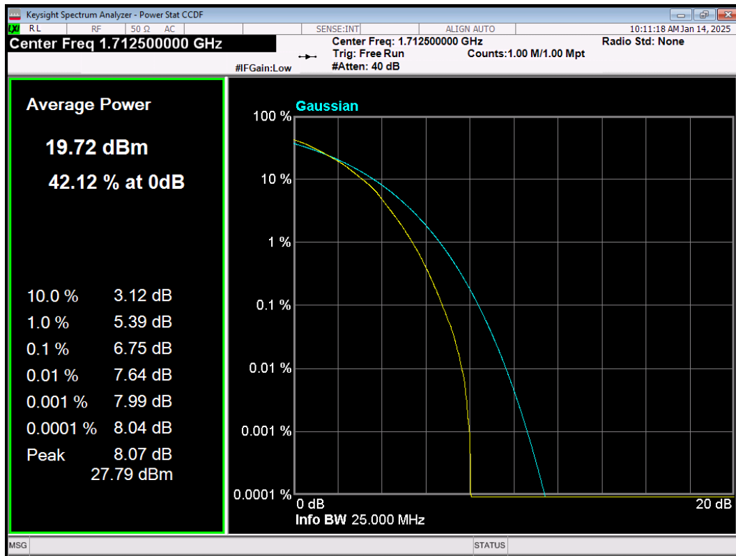
LTE Band4 64QAM BW=5MHz Channel=19975 RB Size=25 Position=#0
