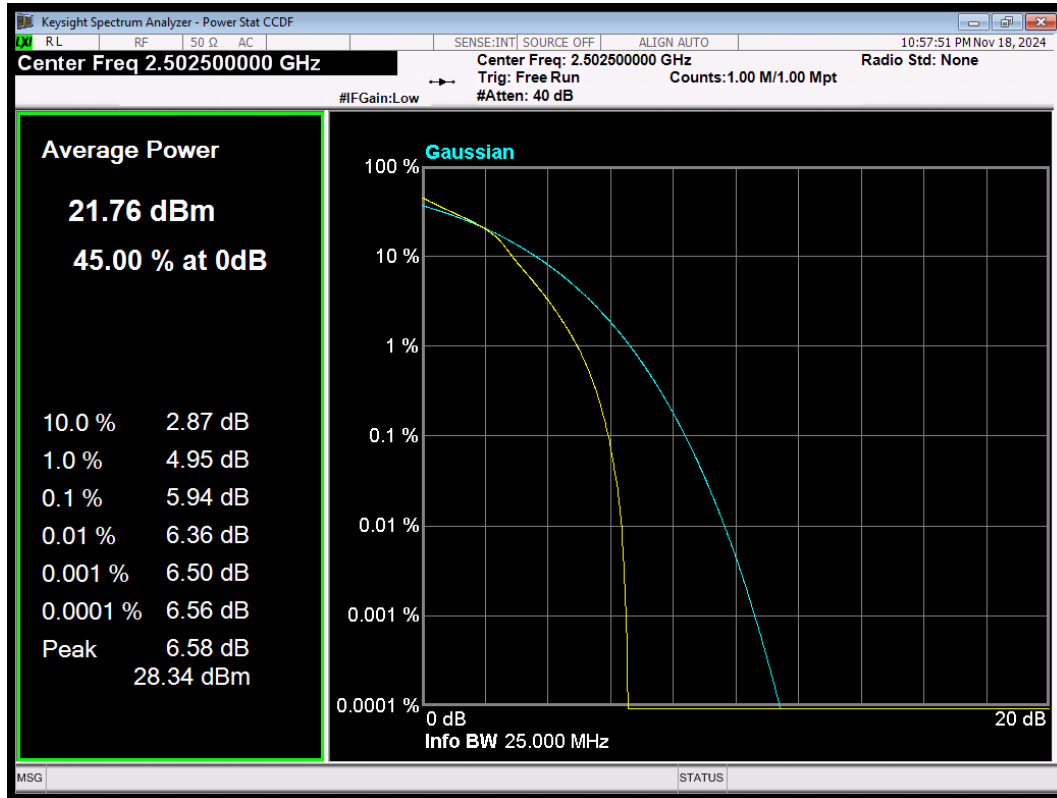
LTE Band7 16QAM BW=5MHz Channel=20775 RB Size=25 Position=#0
