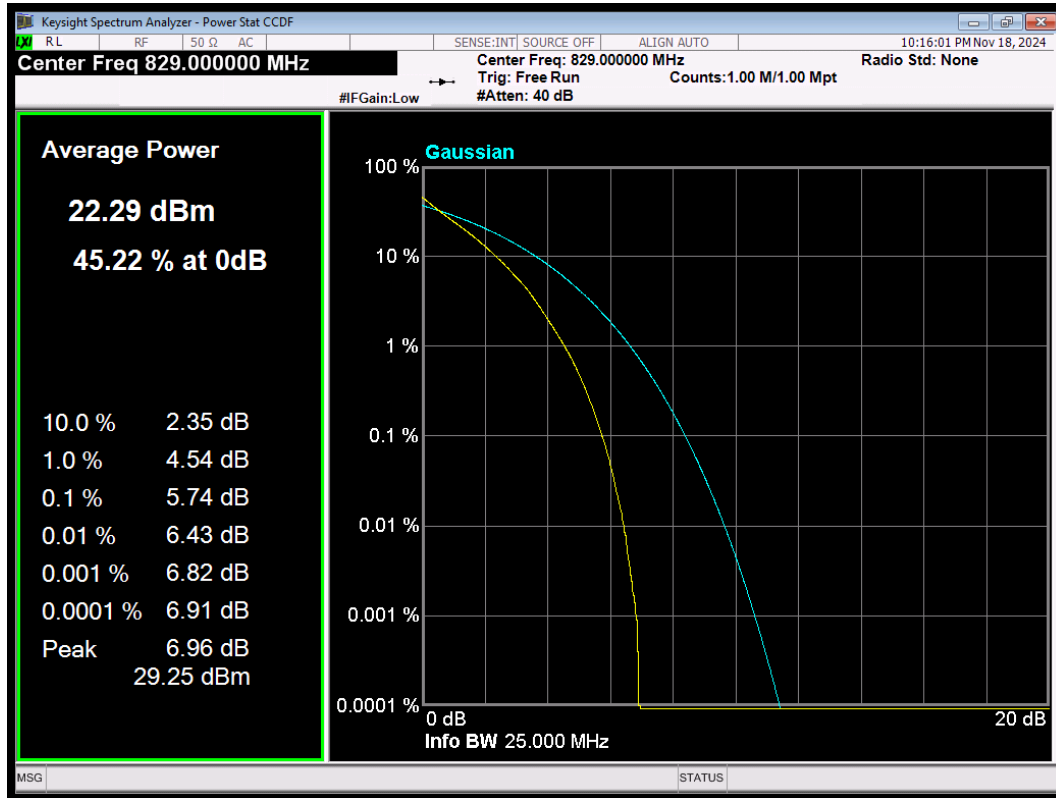
LTE Band5 QPSK BW=10MHz Channel=20450 RB Size=50 Position=#0
