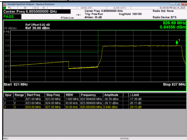
LTE Band26(824-849) 64QAM BW=3MHz LowChannel=26805 RB Size=15 Position=#0
