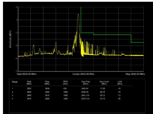
LTE Band41 16QAM BW=20MHz Channel=41140 RB Size=1 Position=#Max
