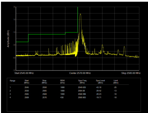
LTE Band38 16QAM BW=20MHz Channel=37850 RB Size=1 Position=#0
