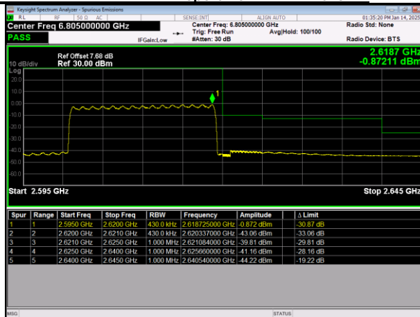
LTE Band38 64QAM BW=20MHz HighChannel=38150 RB Size=100 Position=#0
