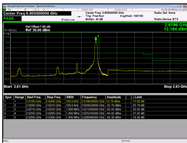
LTE Band38 64QAM BW=5MHz HighChannel=38225 RB Size=1 Position=#Max
