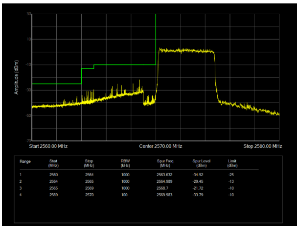
LTE Band38 16QAM BW=5MHz Channel=37775 RB Size=25 Position=#0
