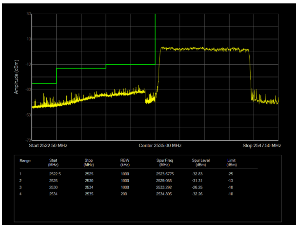
LTE Band41 16QAM BW=10MHz Channel=40090 RB Size=50 Position=#0
