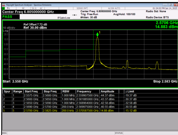
LTE Band38 64QAM BW=10MHz LowChannel=37800 RB Size=1 Position=#0
