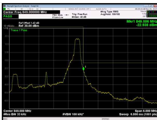
LTE Band26 (824-849) QPSK BW=3MHz Channel=27025 RB Size=1 Position=#Max
