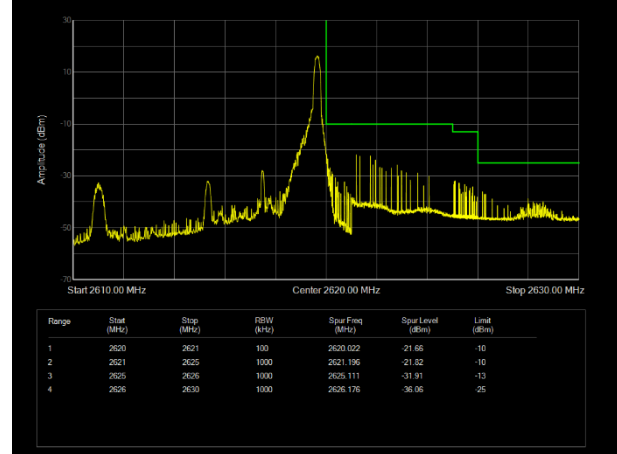
LTE Band38 16QAM BW=5MHz Channel=38225 RB Size=1 Position=#Max
