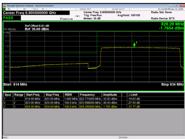
LTE Band26(824-849) 64QAM BW=10MHz LowChannel=26840 RB Size=50 Position=#0
