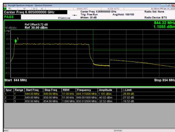
LTE Band26(824-849) 64QAM BW=5MHz HighChannel=27015 RB Size=25 Position=#0
