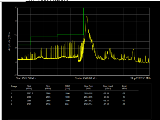
LTE Band38 16QAM BW=10MHz Channel=37800 RB Size=1 Position=#0
