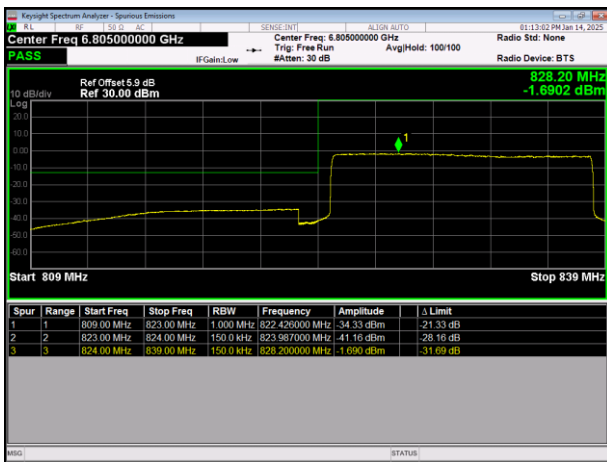
LTE Band26(824-849) 64QAM BW=15MHz LowChannel=26865 RB Size=75 Position=#0
