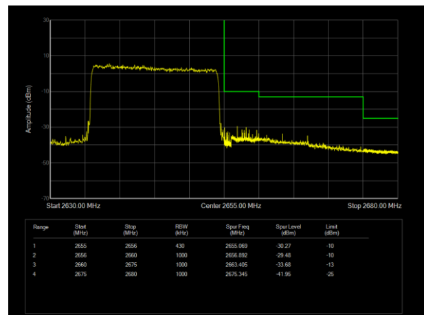
LTE Band41 16QAM BW=20MHz Channel=41140 RB Size=100 Position=#0
