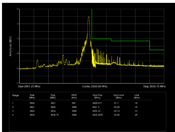
LTE Band38 16QAM BW=15MHz Channel=38175 RB Size=1 Position=#Max
