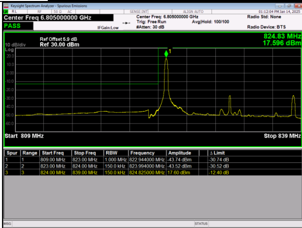
LTE Band26(824-849) 64QAM BW=15MHz LowChannel=26865 RB Size=1 Position=#0
