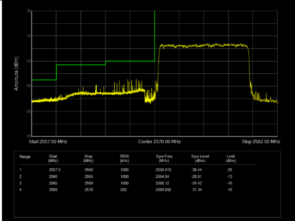
LTE Band38 QPSK BW=10MHz Channel=37800 RB Size=50 Position=#0
