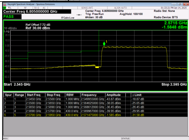
LTE Band38 64QAM BW=20MHz LowChannel=37850 RB Size=100 Position=#0
