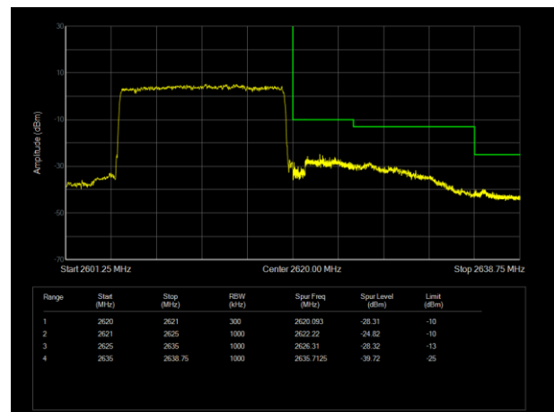
LTE Band38 QPSK BW=15MHz Channel=38175 RB Size=75 Position=#0
