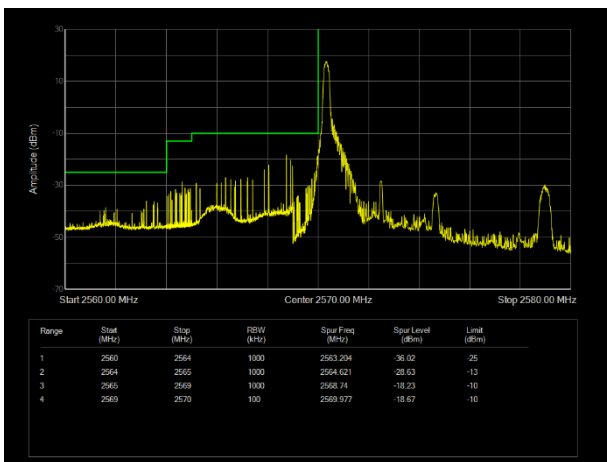
LTE Band38 QPSK BW=5MHz Channel=37775 RB Size=1 Position=#0
