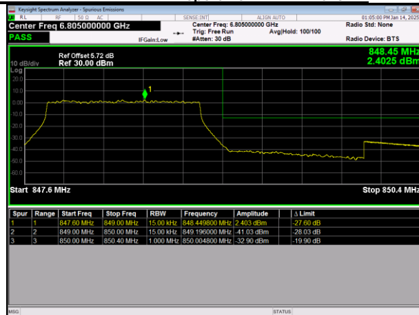
LTE Band26(824-849) 64QAM BW=1.4MHz HighChannel=27033 RB Size=6 Position=#0
