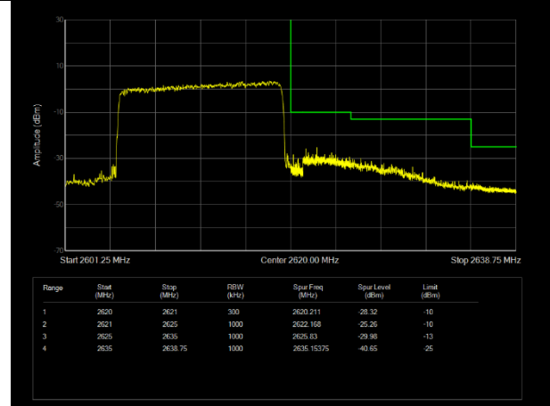
LTE Band38 16QAM BW=15MHz Channel=38175 RB Size=75 Position=#0
