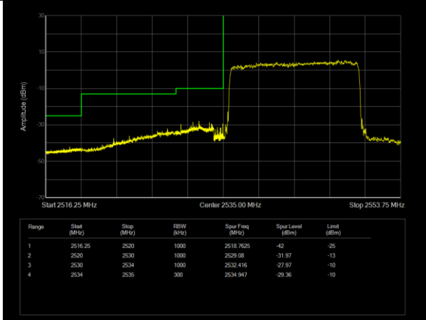
LTE Band41 16QAM BW=15MHz Channel=40115 RB Size=75 Position=#0
