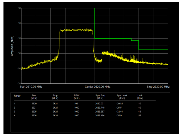
LTE Band38 16QAM BW=5MHz Channel=38225 RB Size=25 Position=#0
