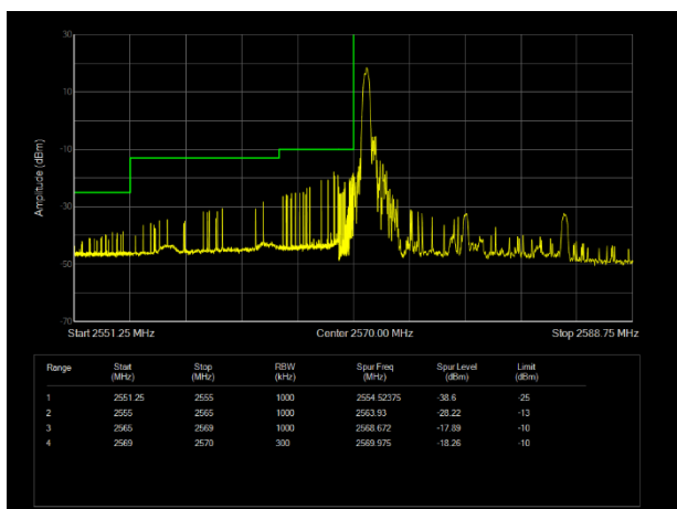
LTE Band38 16QAM BW=15MHz Channel=37825 RB Size=1 Position=#0
