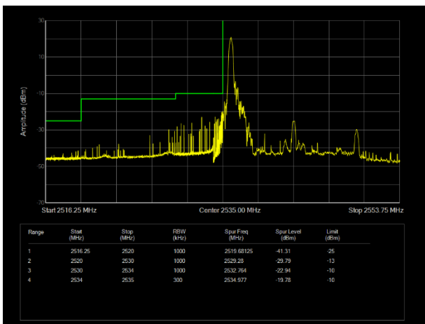
LTE Band41 16QAM BW=15MHz Channel=40115 RB Size=1 Position=#0
