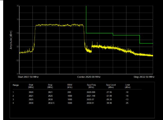
LTE Band38 QPSK BW=10MHz Channel=38200 RB Size=50 Position=#0
