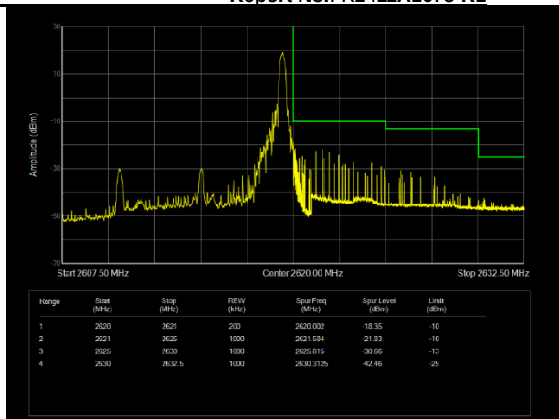
LTE Band38 16QAM BW=10MHz Channel=38200 RB Size=1 Position=#Max
