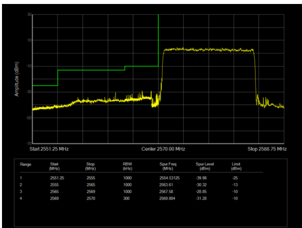
LTE Band38 QPSK BW=15MHz Channel=37825 RB Size=75 Position=#0
