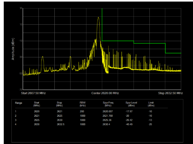
LTE Band38 QPSK BW=10MHz Channel=38200 RB Size=1 Position=#Max
