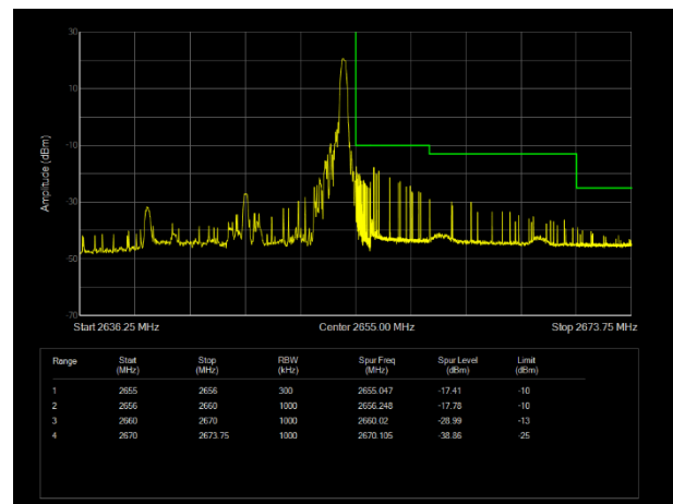
LTE Band41 16QAM BW=15MHz Channel=41165 RB Size=1 Position=#Max
