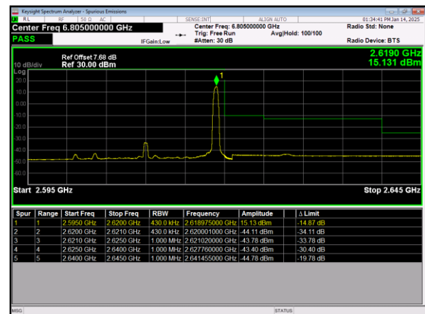
LTE Band38 64QAM BW=20MHz HighChannel=38150 RB Size=1 Position=#Max
