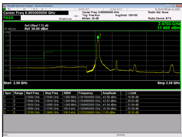
LTE Band38 64QAM BW=5MHz LowChannel=37775 RB Size=1 Position=#0
