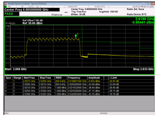
LTE Band38 64QAM BW=10MHz HighChannel=38200 RB Size=50 Position=#0
