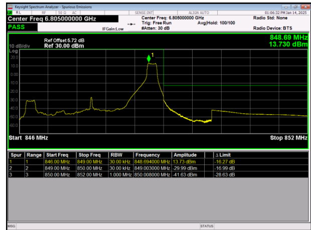
LTE Band26(824-849) 64QAM BW=3MHz HighChannel=27025 RB Size=1 Position=#Max
