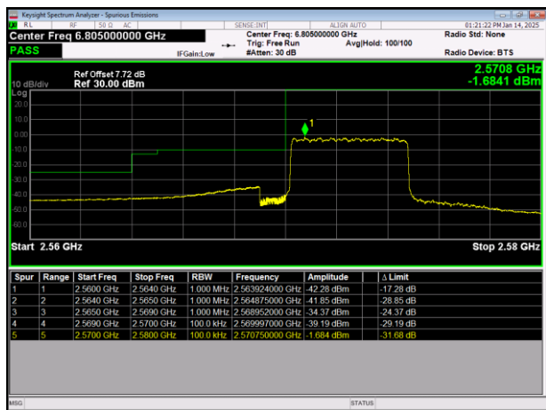
LTE Band38 64QAM BW=5MHz LowChannel=37775 RB Size=25 Position=#0
