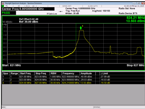
LTE Band26(824-849) 64QAM BW=3MHz LowChannel=26805 RB Size=1 Position=#0
