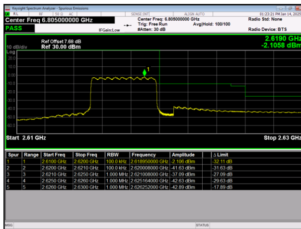
LTE Band38 64QAM BW=5MHz HighChannel=38225 RB Size=25 Position=#0
