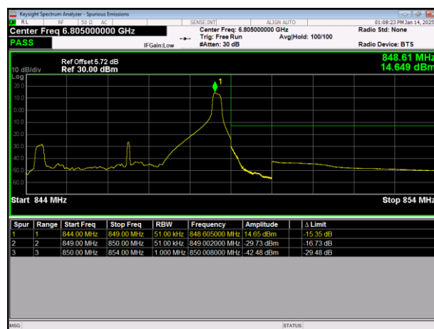
LTE Band26(824-849) 64QAM BW=5MHz HighChannel=27015 RB Size=1 Position=#Max
