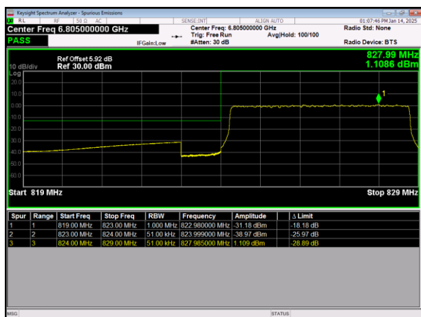
LTE Band26(824-849) 64QAM BW=5MHz LowChannel=26815 RB Size=25 Position=#0
