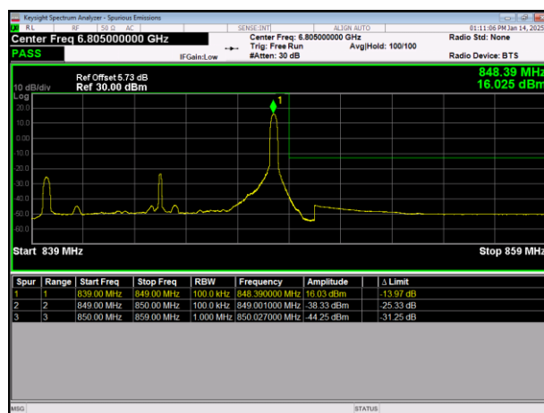
LTE Band26(824-849) 64QAM BW=10MHz HighChannel=26990 RB Size=1 Position=#Max
