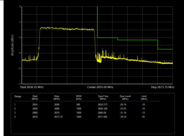
LTE Band41 16QAM BW=15MHz Channel=41165 RB Size=75 Position=#0
