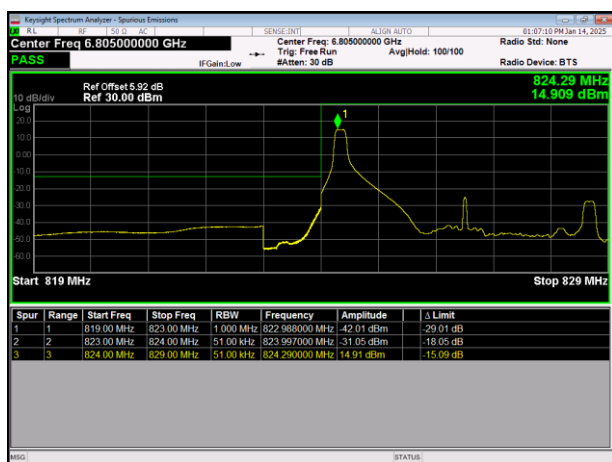
LTE Band26(824-849) 64QAM BW=5MHz LowChannel=26815 RB Size=1 Position=#0
