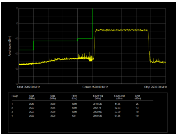
LTE Band38 16QAM BW=20MHz Channel=37850 RB Size=100 Position=#0
