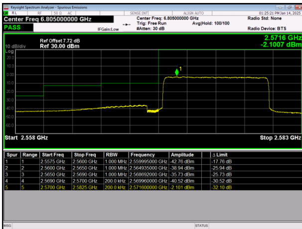
LTE Band38 64QAM BW=10MHz LowChannel=37800 RB Size=50 Position=#0
