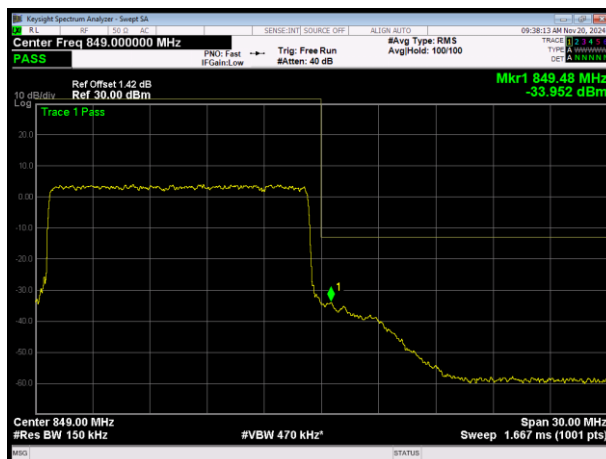
LTE Band26 (824-849) QPSK BW=15MHz Channel=26965 RB Size=75 Position=#0
