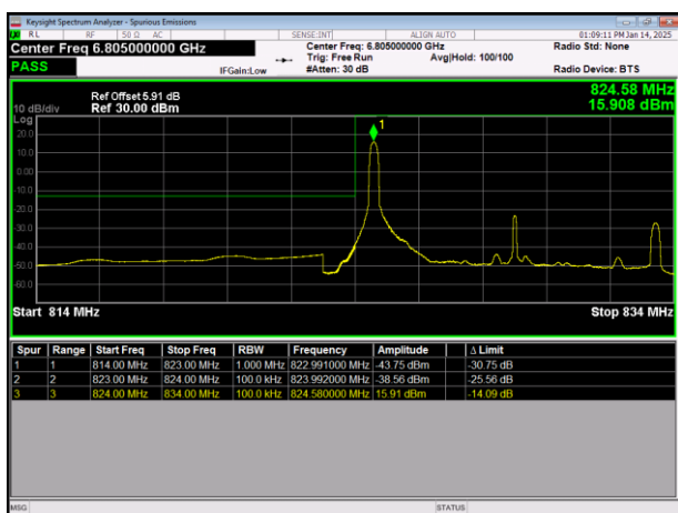
LTE Band26(824-849) 64QAM BW=10MHz LowChannel=26840 RB Size=1 Position=#0
