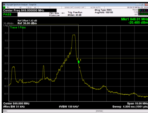
LTE Band26 (824-849) QPSK BW=5MHz Channel=27015 RB Size=1 Position=#Max
