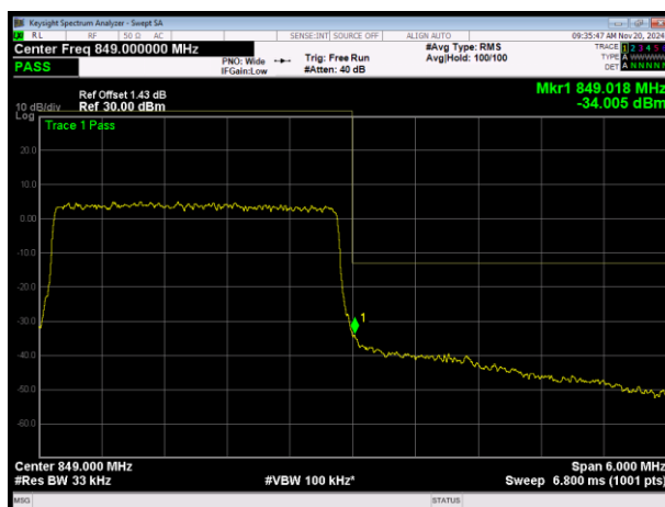
LTE Band26 (824-849) QPSK BW=3MHz Channel=27025 RB Size=15 Position=#0
