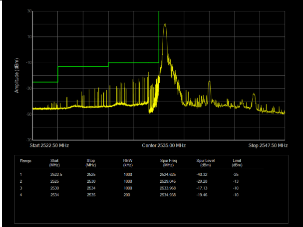
LTE Band41 16QAM BW=10MHz Channel=40090 RB Size=1 Position=#0
