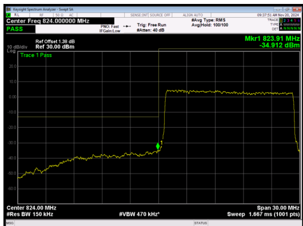
LTE Band26 (824-849) QPSK BW=15MHz Channel=26865 RB Size=75 Position=#0
