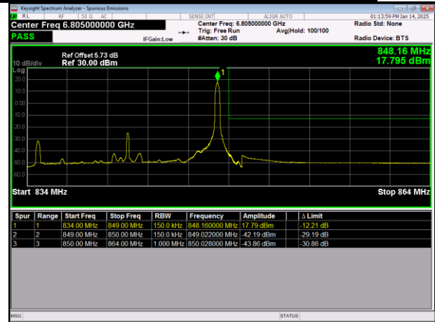
LTE Band26(824-849) 64QAM BW=15MHz HighChannel=26965 RB Size=1 Position=#Max
