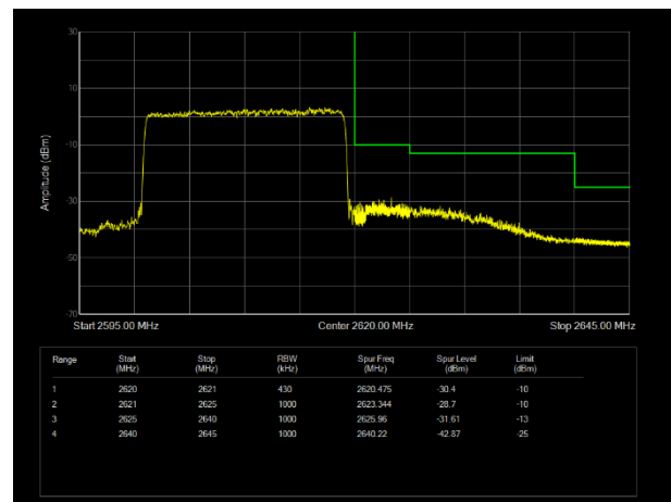
LTE Band38 16QAM BW=20MHz Channel=38150 RB Size=100 Position=#0
