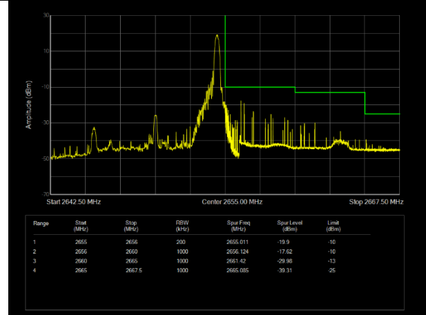
LTE Band41 16QAM BW=10MHz Channel=41190 RB Size=1 Position=#Max
