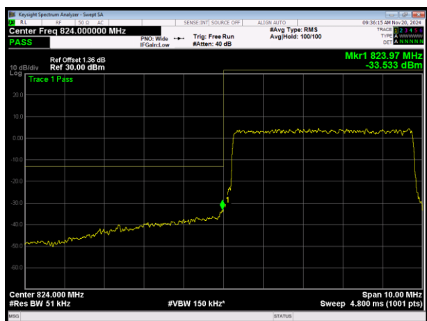
LTE Band26 (824-849) QPSK BW=5MHz Channel=26815 RB Size=25 Position=#0
