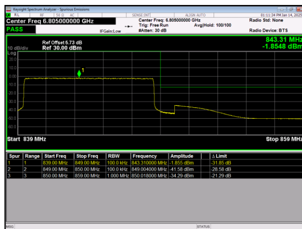
LTE Band26(824-849) 64QAM BW=10MHz HighChannel=26990 RB Size=50 Position=#0
