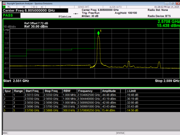
LTE Band38 64QAM BW=15MHz LowChannel=37825 RB Size=1 Position=#0
