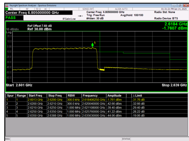
LTE Band38 64QAM BW=15MHz HighChannel=38175 RB Size=75 Position=#0
