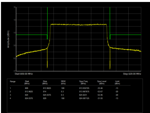
LTE Band26 (814-824) QPSK BW=10MHz Channel=26740 RB Size=50 Position=#0
