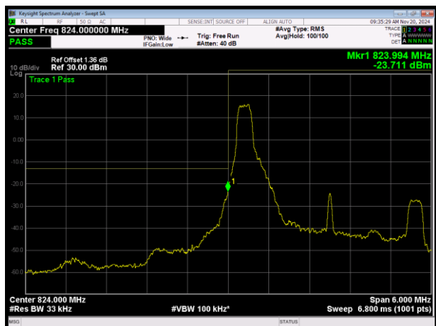
LTE Band26 (824-849) 16QAM BW=3MHz Channel=26805 RB Size=1 Position=#0
