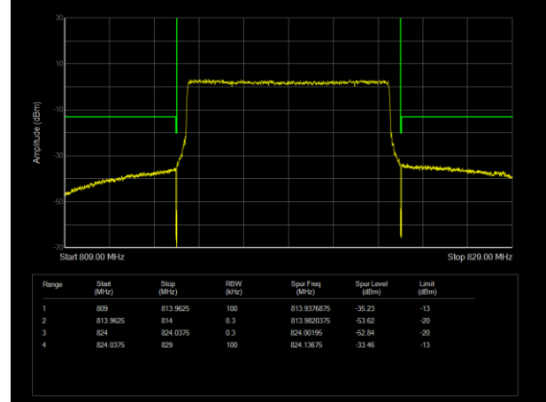
LTE Band26 (814-824) 16QAM BW=10MHz Channel=26740 RB Size=50 Position=#0
