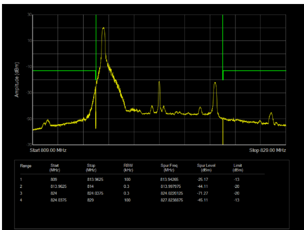
LTE Band26 (814-824) 16QAM BW=10MHz Channel=26740 RB Size=1 Position=#0
