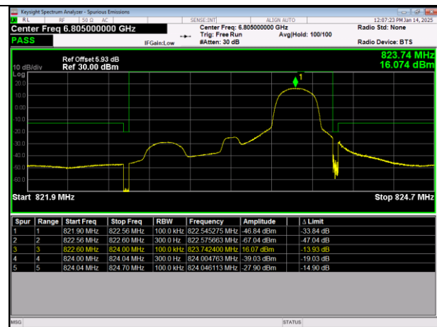
LTE Band26(814-824) 64QAM BW=1.4MHz HighChannel=26783 RB Size=1 Position=#Max
