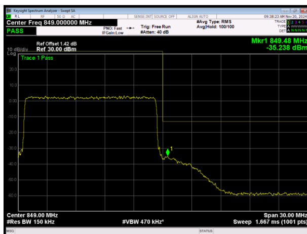
LTE Band26 (824-849) 16QAM BW=15MHz Channel=26965 RB Size=75 Position=#0
