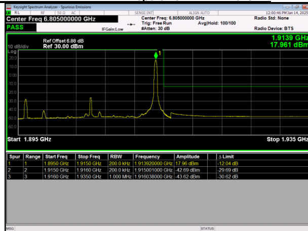
LTE Band25 64QAM BW=20MHz HighChannel=26590 RB Size=1 Position=#Max
