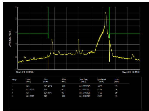
LTE Band26 (814-824) QPSK BW=10MHz Channel=26740 RB Size=1 Position=#Max
