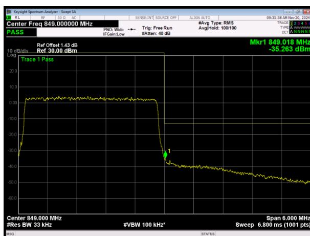
LTE Band26 (824-849) 16QAM BW=3MHz Channel=27025 RB Size=15 Position=#0
