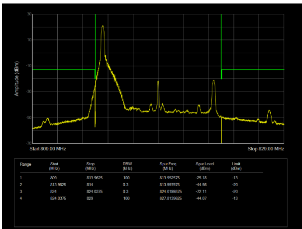
LTE Band26 (814-824) QPSK BW=10MHz Channel=26740 RB Size=1 Position=#0
