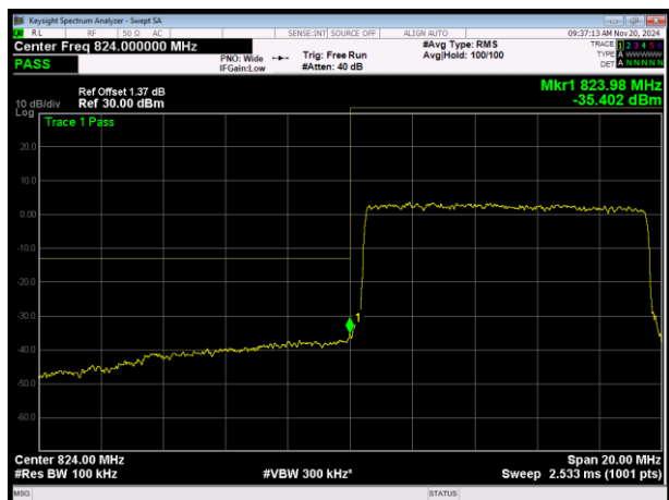
LTE Band26 (824-849) 16QAM BW=10MHz Channel=26840 RB Size=50 Position=#0
