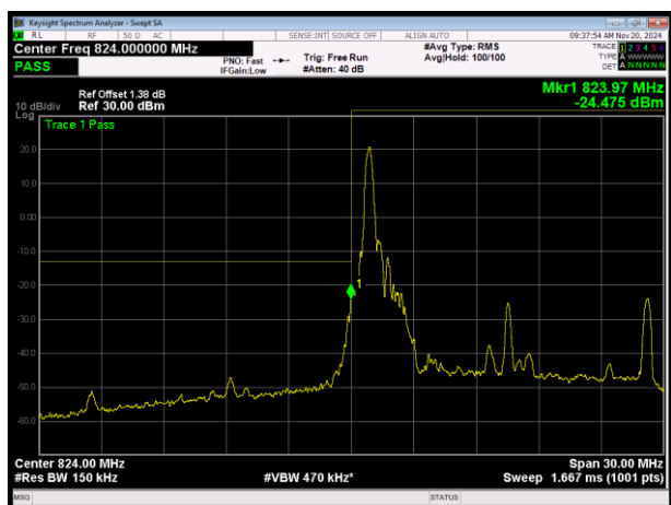
LTE Band26 (824-849) 16QAM BW=15MHz Channel=26865 RB Size=1 Position=#0
