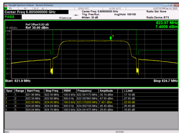
LTE Band26(814-824) 64QAM BW=1.4MHz HighChannel=26783 RB Size=6 Position=#0
