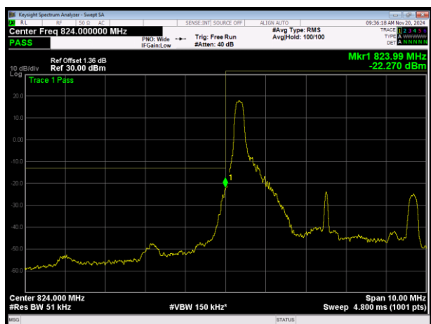
LTE Band26 (824-849) 16QAM BW=5MHz Channel=26815 RB Size=1 Position=#0
