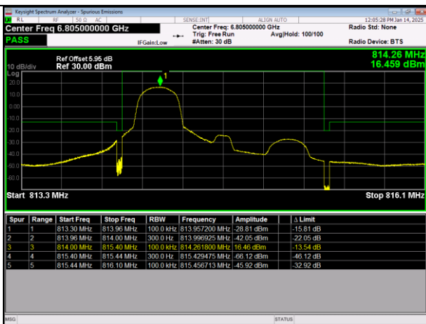
LTE Band26(814-824) 64QAM BW=1.4MHz LowChannel=26697 RB Size=1 Position=#0
