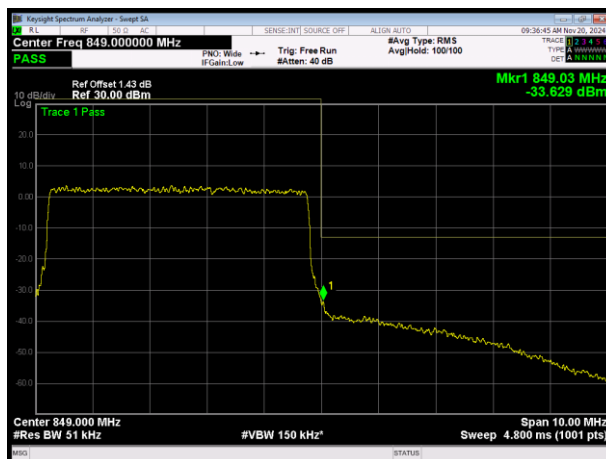
LTE Band26 (824-849) 16QAM BW=5MHz Channel=27015 RB Size=25 Position=#0
