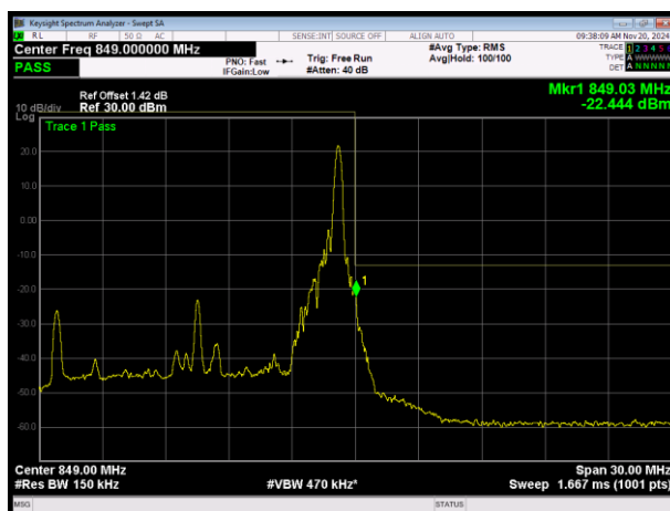
LTE Band26 (824-849) QPSK BW=15MHz Channel=26965 RB Size=1 Position=#Max
