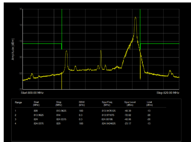
LTE Band26 (814-824) 16QAM BW=10MHz Channel=26740 RB Size=1 Position=#Max
