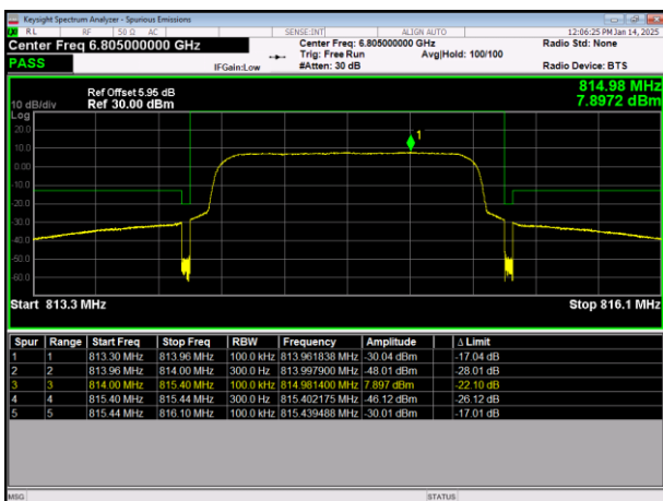
LTE Band26(814-824) 64QAM BW=1.4MHz LowChannel=26697 RB Size=6 Position=#0
