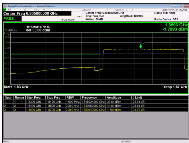
LTE Band25 64QAM BW=20MHz LowChannel=26140 RB Size=100 Position=#0
