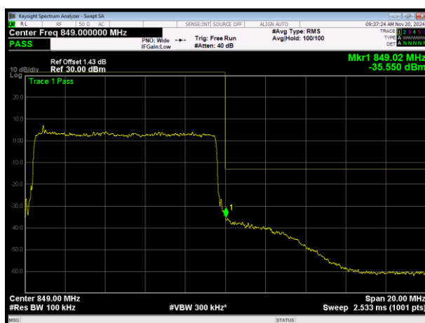
LTE Band26 (824-849) QPSK BW=10MHz Channel=26990 RB Size=50 Position=#0
