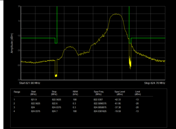
LTE Band26 (814-824) 16QAM BW=1.4MHz Channel=26783 RB Size=1 Position=#Max
