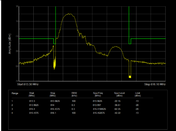
LTE Band26 (814-824) 16QAM BW=1.4MHz Channel=26697 RB Size=1 Position=#0
