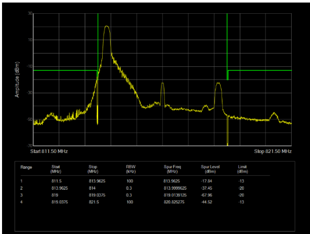
LTE Band26 (814-824) QPSK BW=5MHz Channel=26715 RB Size=1 Position=#0
