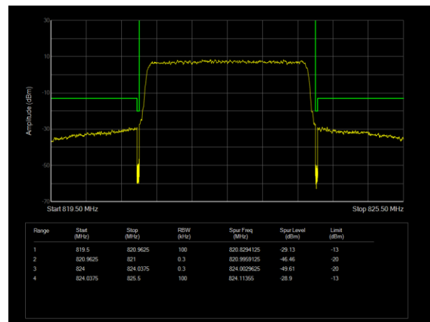
LTE Band26 (814-824) 16QAM BW=3MHz Channel=26775 RB Size=15 Position=#0
