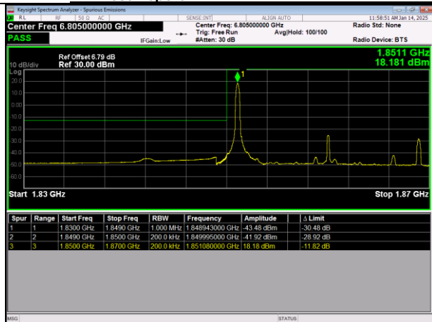
LTE Band25 64QAM BW=20MHz LowChannel=26140 RB Size=1 Position=#0
