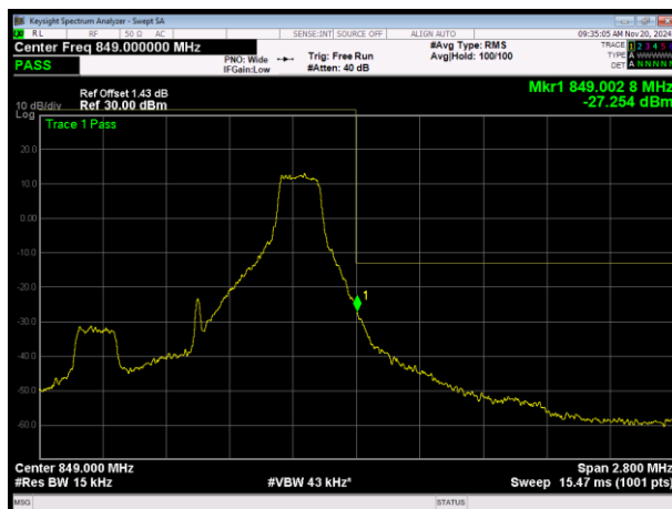
LTE Band26 (824-849) 16QAM BW=1.4MHz Channel=27033 RB Size=1 Position=#Max
