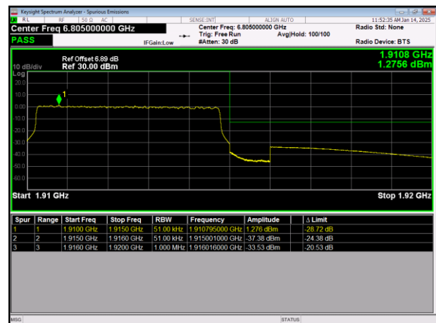
LTE Band25 64QAM BW=5MHz HighChannel=26665 RB Size=25 Position=#0
