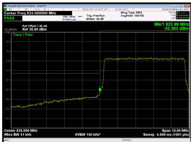
LTE Band26 (824-849) 16QAM BW=5MHz Channel=26815 RB Size=25 Position=#0
