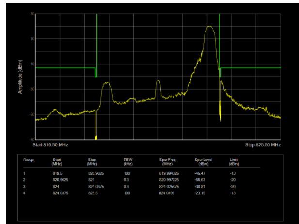
LTE Band26 (814-824) 16QAM BW=3MHz Channel=26775 RB Size=1 Position=#Max
