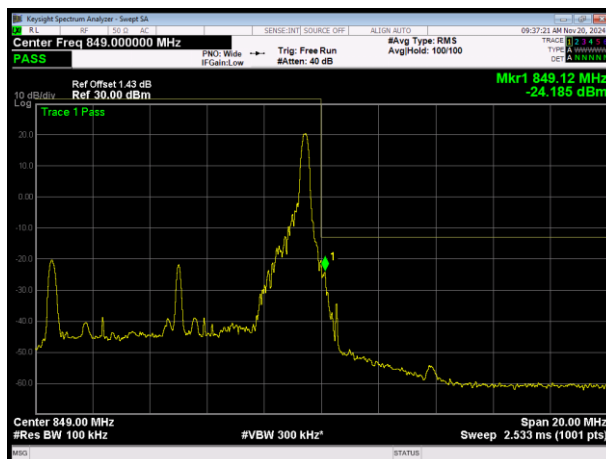
LTE Band26 (824-849) QPSK BW=10MHz Channel=26990 RB Size=1 Position=#Max
