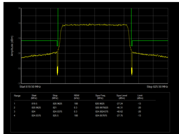
LTE Band26 (814-824) QPSK BW=3MHz Channel=26775 RB Size=15 Position=#0
