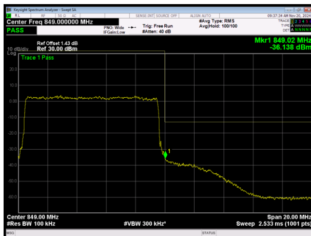
LTE Band26 (824-849) 16QAM BW=10MHz Channel=26990 RB Size=50 Position=#0
