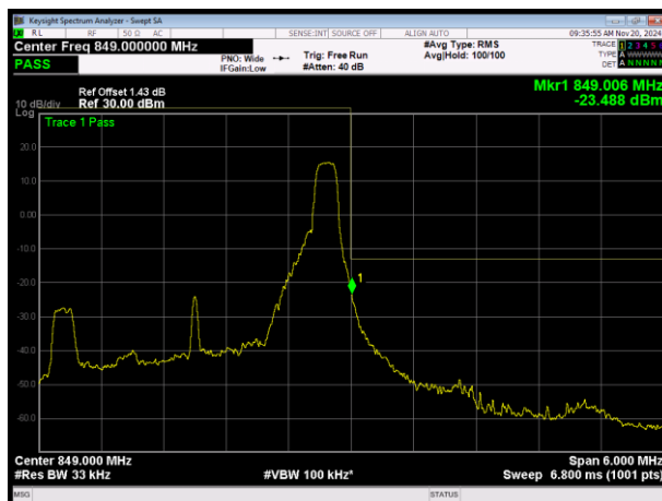
LTE Band26 (824-849) 16QAM BW=3MHz Channel=27025 RB Size=1 Position=#Max
