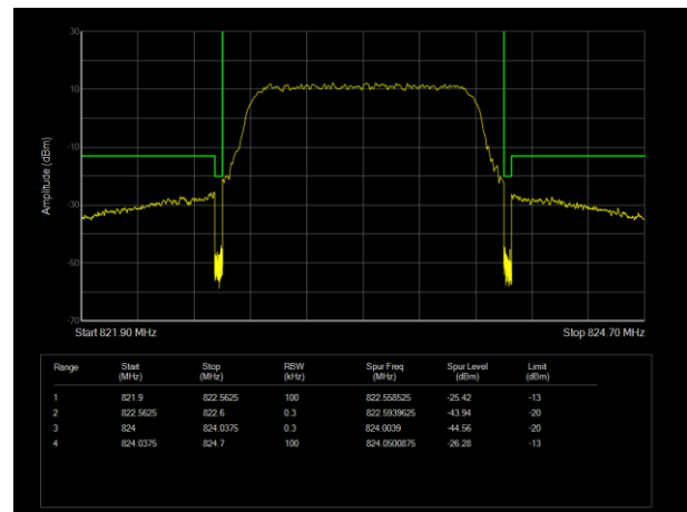
LTE Band26 (814-824) 16QAM BW=1.4MHz Channel=26783 RB Size=6 Position=#0
