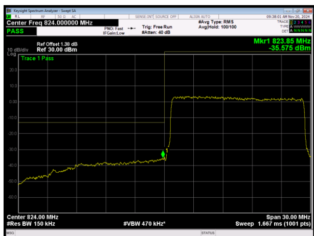
LTE Band26 (824-849) 16QAM BW=15MHz Channel=26865 RB Size=75 Position=#0
