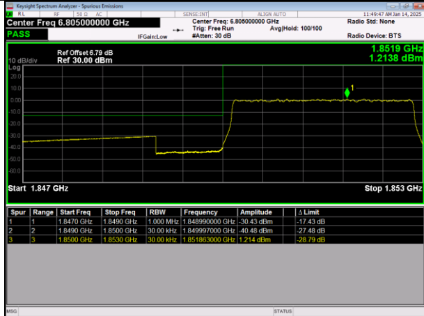
LTE Band25 64QAM BW=3MHz LowChannel=26055 RB Size=15 Position=#0
