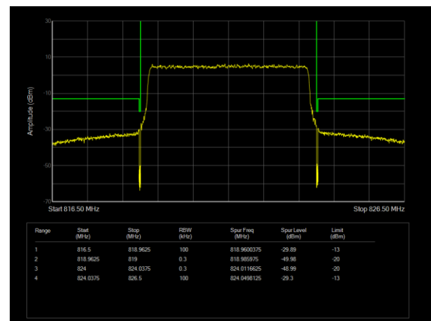
LTE Band26 (814-824) 16QAM BW=5MHz Channel=26765 RB Size=25 Position=#0
