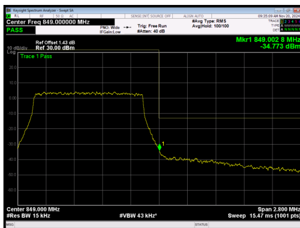
LTE Band26 (824-849) 16QAM BW=1.4MHz Channel=27033 RB Size=6 Position=#0
