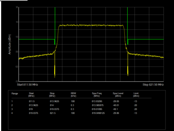
LTE Band26 (814-824) QPSK BW=5MHz Channel=26715 RB Size=25 Position=#0
