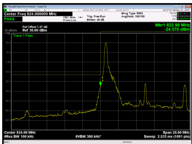
LTE Band26 (824-849) 16QAM BW=10MHz Channel=26840 RB Size=1 Position=#0
