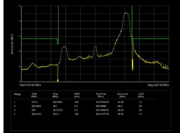
LTE Band26 (814-824) QPSK BW=3MHz Channel=26775 RB Size=1 Position=#Max
