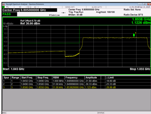
LTE Band25 64QAM BW=5MHz LowChannel=26065 RB Size=25 Position=#0
