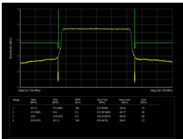
LTE Band26 (814-824) 16QAM BW=5MHz Channel=26715 RB Size=25 Position=#0
