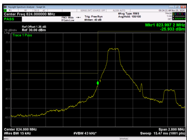
LTE Band26 (824-849) QPSK BW=1.4MHz Channel=26797 RB Size=1 Position=#0
