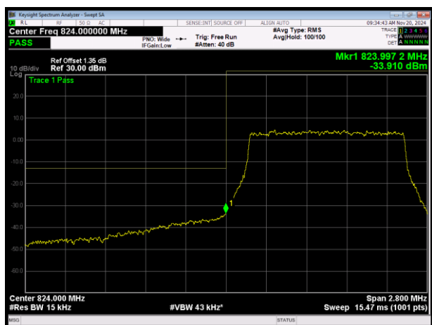
LTE Band26 (824-849) 16QAM BW=1.4MHz Channel=26797 RB Size=6 Position=#0
