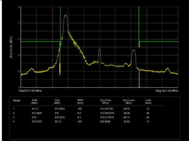
LTE Band26 (814-824) 16QAM BW=5MHz Channel=26715 RB Size=1 Position=#0
