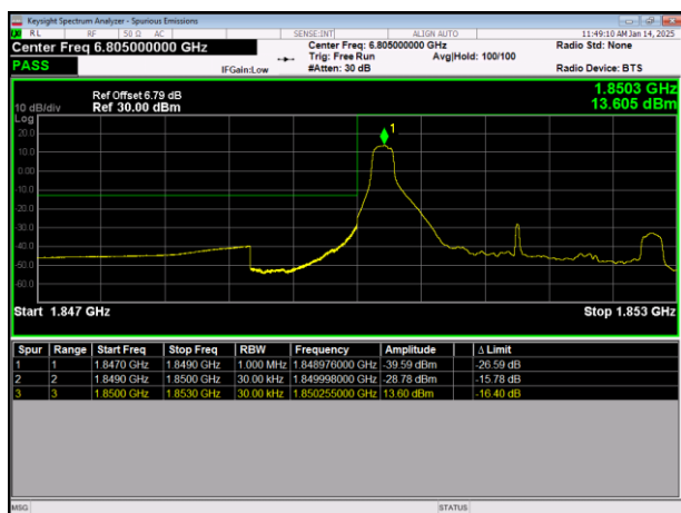
LTE Band25 64QAM BW=3MHz LowChannel=26055 RB Size=1 Position=#0
