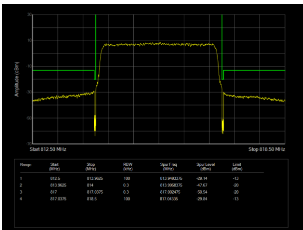
LTE Band26 (814-824) 16QAM BW=3MHz Channel=26705 RB Size=15 Position=#0
