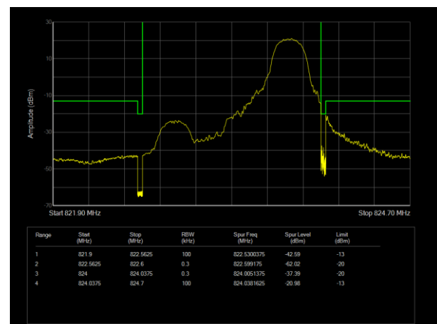
LTE Band26 (814-824) QPSK BW=1.4MHz Channel=26783 RB Size=1 Position=#Max
