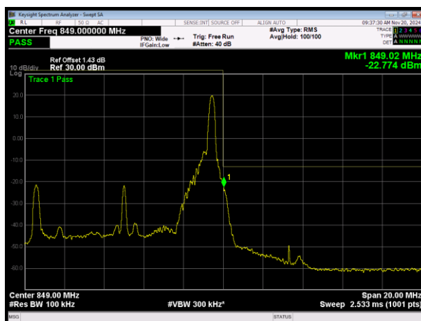
LTE Band26 (824-849) 16QAM BW=10MHz Channel=26990 RB Size=1 Position=#Max
