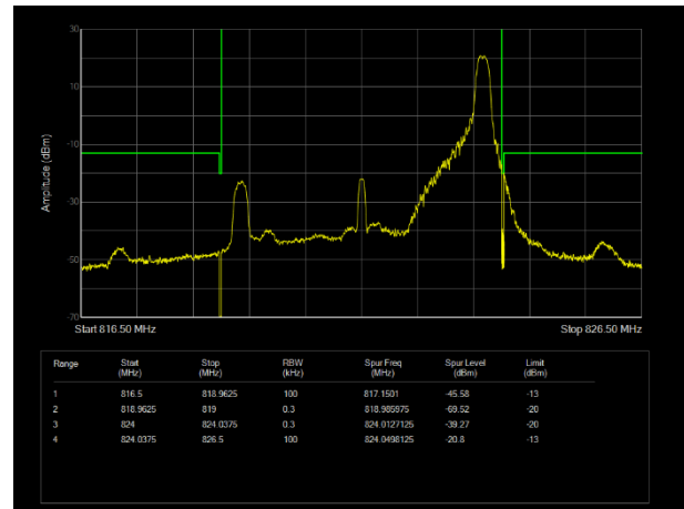
LTE Band26 (814-824) QPSK BW=5MHz Channel=26765 RB Size=1 Position=#Max
