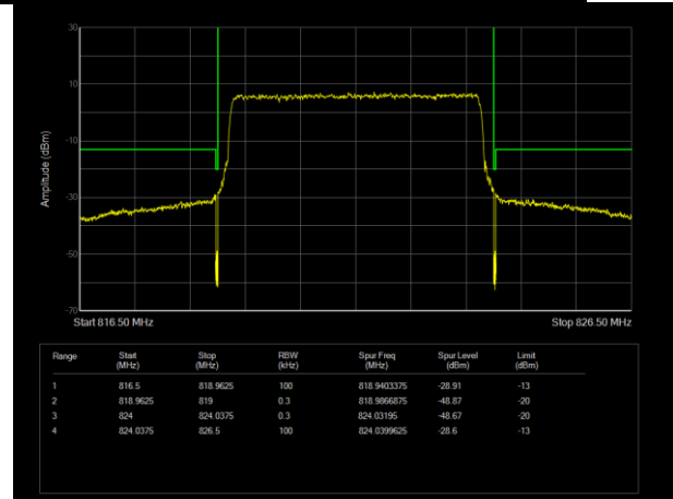
LTE Band26 (814-824) QPSK BW=5MHz Channel=26765 RB Size=25 Position=#0
