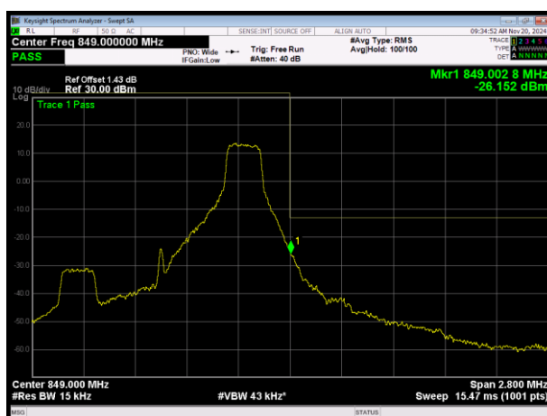
LTE Band26 (824-849) QPSK BW=1.4MHz Channel=27033 RB Size=1 Position=#Max
