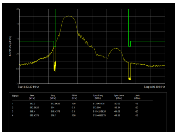
LTE Band26 (814-824) QPSK BW=1.4MHz Channel=26697 RB Size=1 Position=#0
