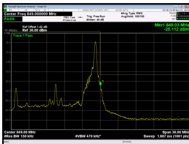
LTE Band26 (824-849) 16QAM BW=15MHz Channel=26965 RB Size=1 Position=#Max
