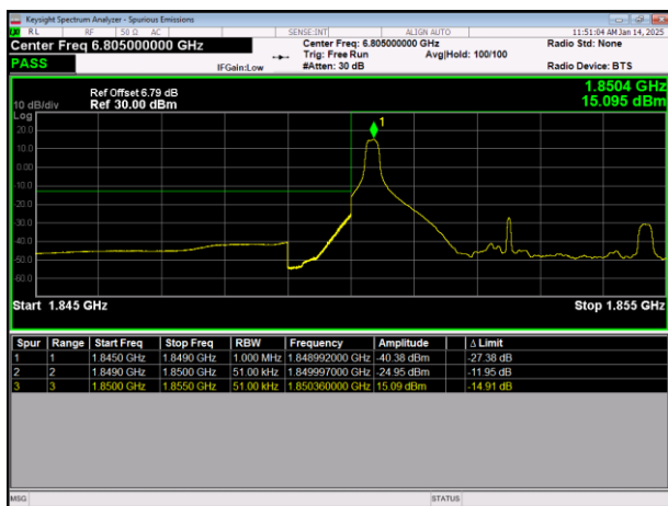
LTE Band25 64QAM BW=5MHz LowChannel=26065 RB Size=1 Position=#0
