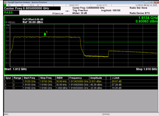
LTE Band25 64QAM BW=3MHz HighChannel=26675 RB Size=15 Position=#0
