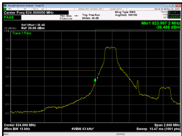
LTE Band26 (824-849) 16QAM BW=1.4MHz Channel=26797 RB Size=1 Position=#0
