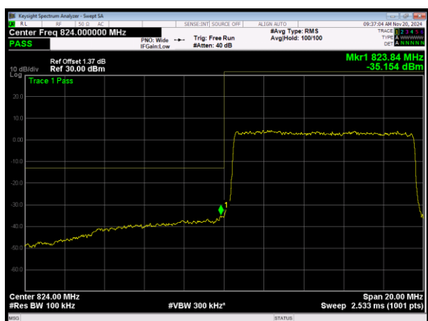
LTE Band26 (824-849) QPSK BW=10MHz Channel=26840 RB Size=50 Position=#0
