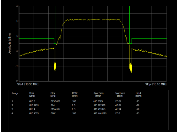
LTE Band26 (814-824) QPSK BW=1.4MHz Channel=26697 RB Size=6 Position=#0
