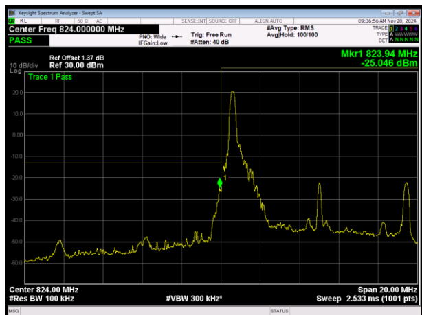
LTE Band26 (824-849) QPSK BW=10MHz Channel=26840 RB Size=1 Position=#0
