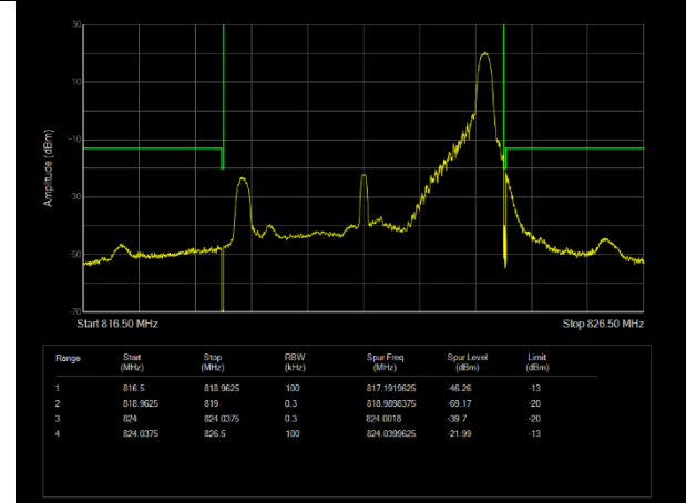
LTE Band26 (814-824) 16QAM BW=5MHz Channel=26765 RB Size=1 Position=#Max
