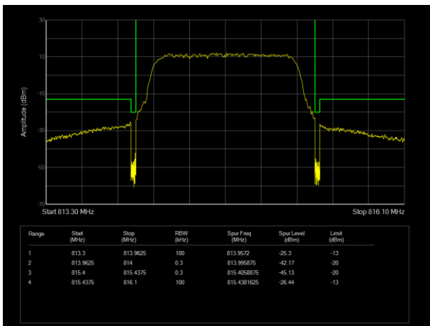
LTE Band26 (814-824) 16QAM BW=1.4MHz Channel=26697 RB Size=6 Position=#0
