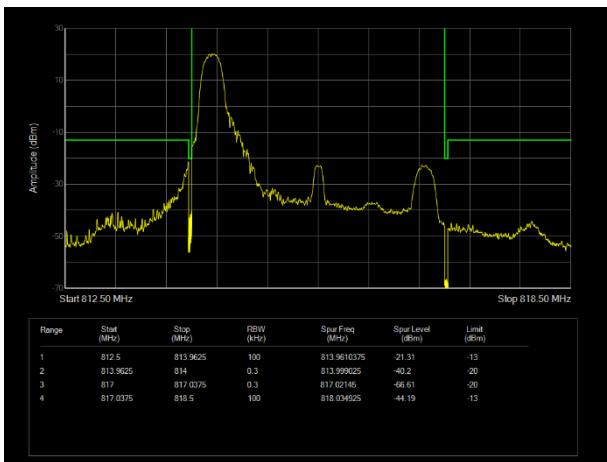
LTE Band26 (814-824) 16QAM BW=3MHz Channel=26705 RB Size=1 Position=#0
