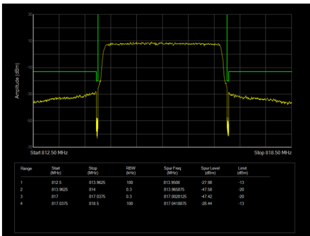
LTE Band26 (814-824) QPSK BW=3MHz Channel=26705 RB Size=15 Position=#0
