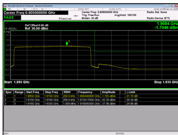
LTE Band25 64QAM BW=20MHz HighChannel=26590 RB Size=100 Position=#0
