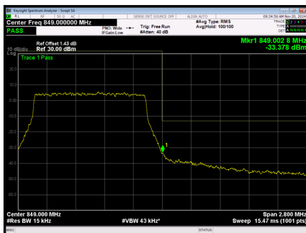
LTE Band26 (824-849) QPSK BW=1.4MHz Channel=27033 RB Size=6 Position=#0
