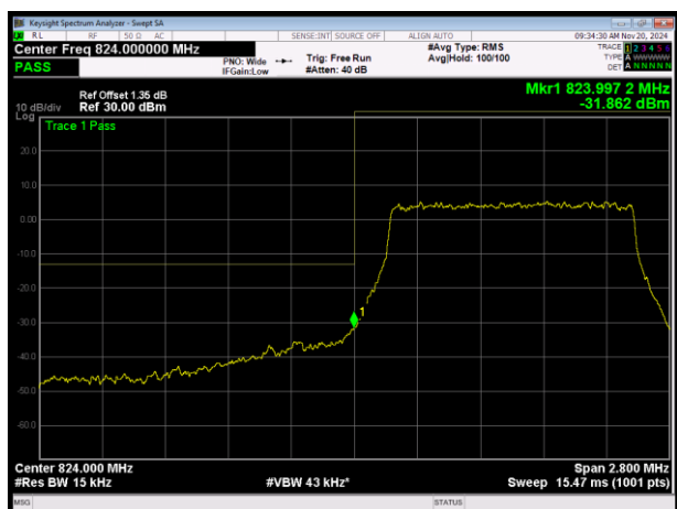
LTE Band26 (824-849) QPSK BW=1.4MHz Channel=26797 RB Size=6 Position=#0
