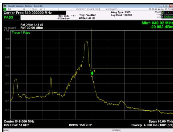
LTE Band26 (824-849) 16QAM BW=5MHz Channel=27015 RB Size=1 Position=#Max
