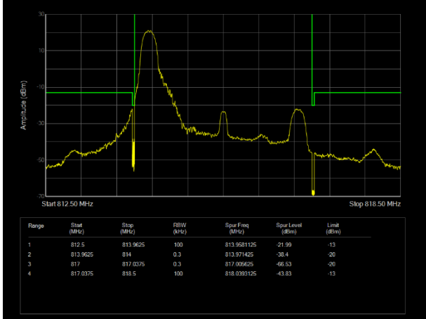
LTE Band26 (814-824) QPSK BW=3MHz Channel=26705 RB Size=1 Position=#0
