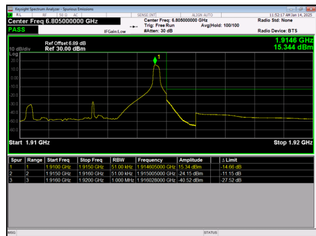
LTE Band25 64QAM BW=5MHz HighChannel=26665 RB Size=1 Position=#Max
