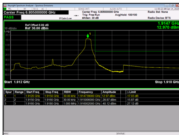
LTE Band25 64QAM BW=3MHz HighChannel=26675 RB Size=1 Position=#Max
