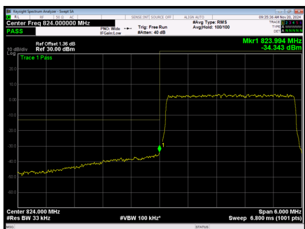
LTE Band26 (824-849) 16QAM BW=3MHz Channel=26805 RB Size=15 Position=#0
