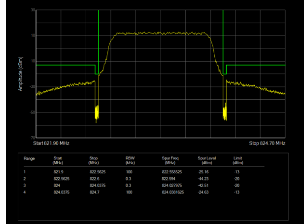
LTE Band26 (814-824) QPSK BW=1.4MHz Channel=26783 RB Size=6 Position=#0
