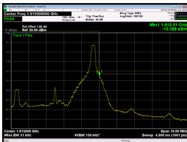
LTE Band25 16QAM BW=5MHz Channel=26665 RB Size=1 Position=#Max
