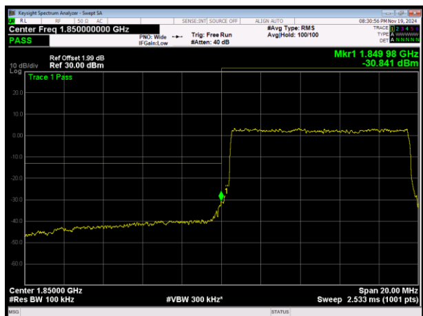
LTE Band25 16QAM BW=10MHz Channel=26090 RB Size=50 Position=#0
