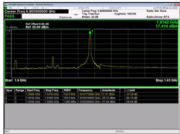
LTE Band25 64QAM BW=15MHz HighChannel=26615 RB Size=1 Position=#Max
