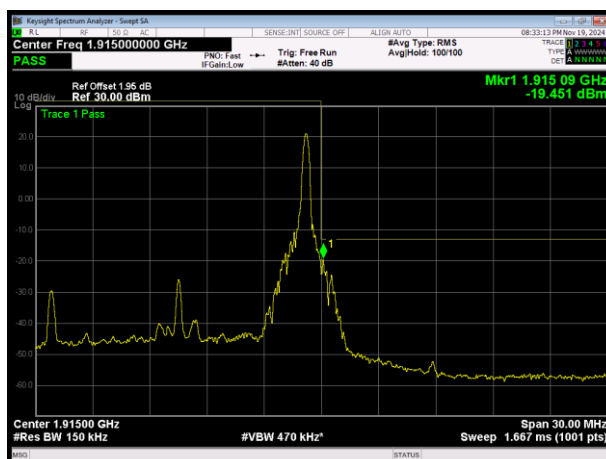
LTE Band25 16QAM BW=15MHz Channel=26615 RB Size=1 Position=#Max
