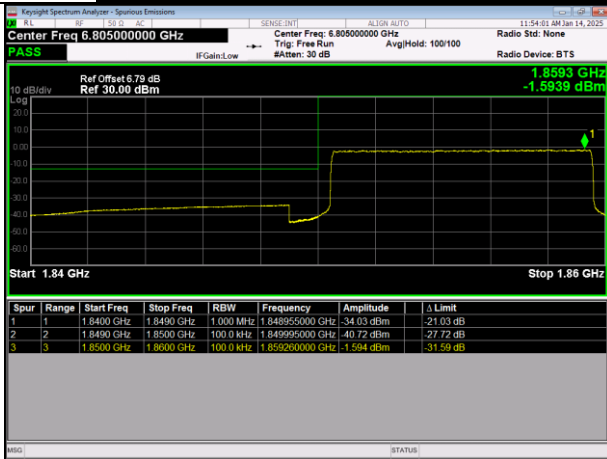
LTE Band25 64QAM BW=10MHz LowChannel=26090 RB Size=50 Position=#0
