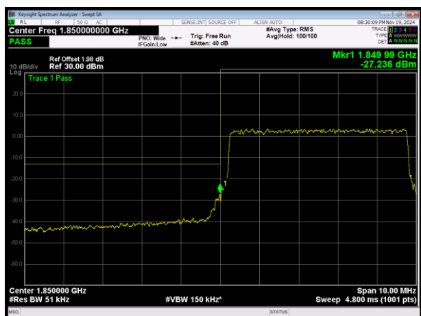
LTE Band25 16QAM BW=5MHz Channel=26065 RB Size=25 Position=#0
