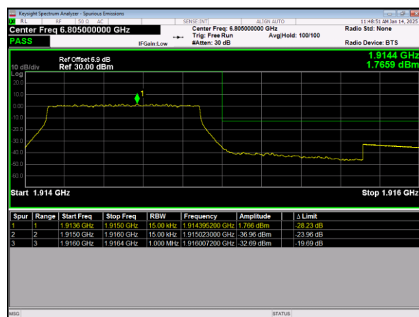
LTE Band25 64QAM BW=1.4MHz HighChannel=26683 RB Size=6 Position=#0
