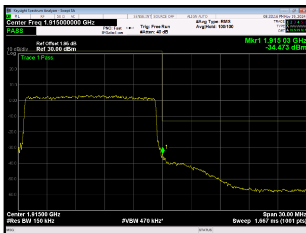
LTE Band25 16QAM BW=15MHz Channel=26615 RB Size=75 Position=#0
