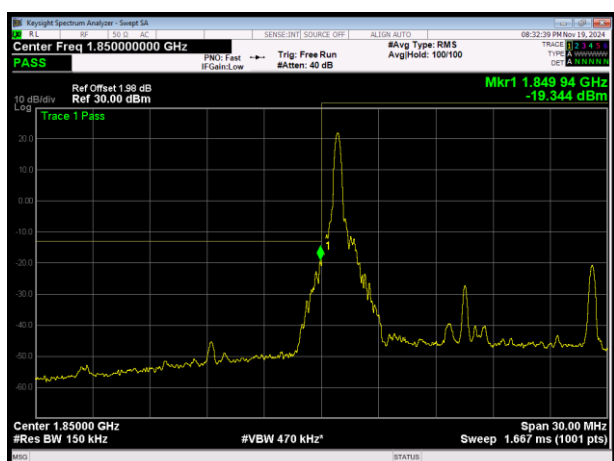
LTE Band25 QPSK BW=15MHz Channel=26115 RB Size=1 Position=#0
