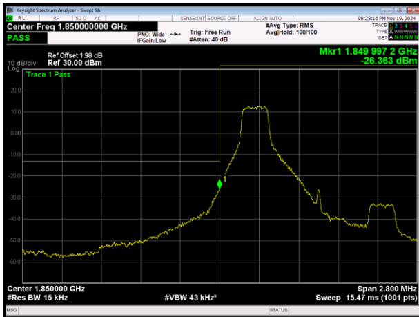
LTE Band25 16QAM BW=1.4MHz Channel=26047 RB Size=1 Position=#0
