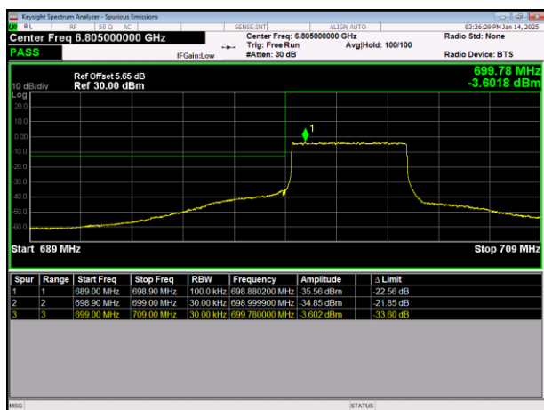
LTE Band12 64QAM BW=5MHz LowChannel=23035 RB Size=25 Position=#0
