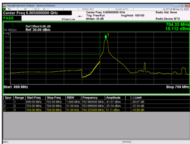
LTE Band17 64QAM BW=5MHz LowChannel=23755 RB Size=1 Position=#0
