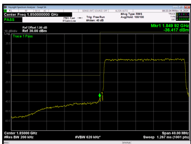
LTE Band25 QPSK BW=20MHz Channel=26140 RB Size=100 Position=#0
