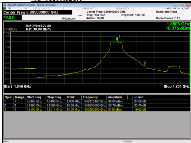
LTE Band25 64QAM BW=1.4MHz LowChannel=26047 RB Size=1 Position=#0
