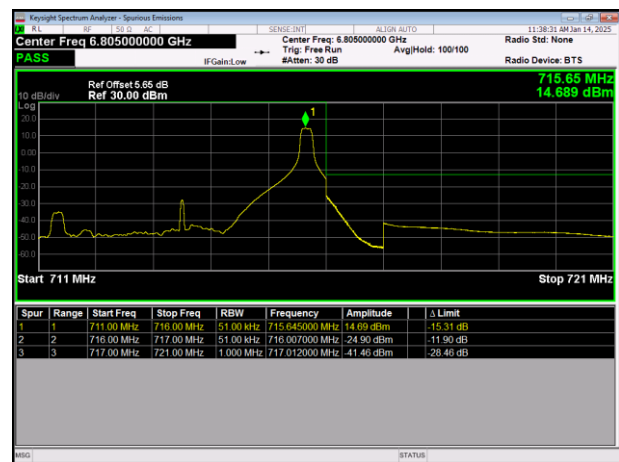
LTE Band17 64QAM BW=5MHz HighChannel=23825 RB Size=1 Position=#Max
