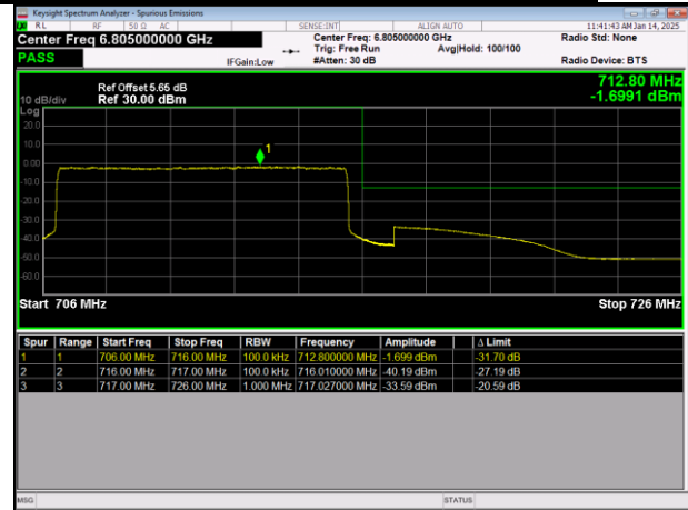
LTE Band17 64QAM BW=10MHz HighChannel=23800 RB Size=50 Position=#0
