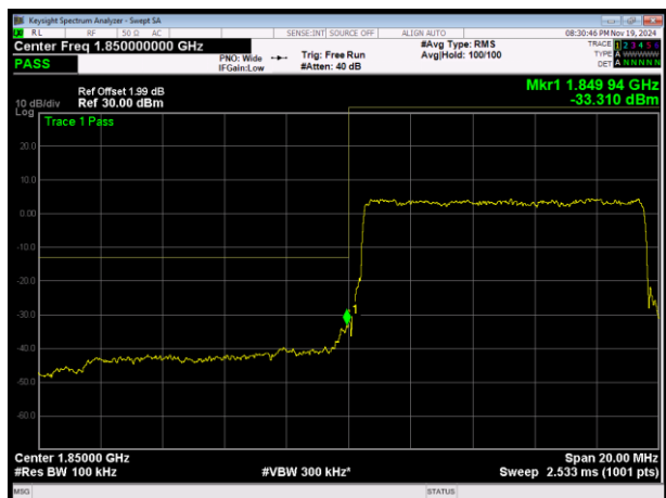
LTE Band25 QPSK BW=10MHz Channel=26090 RB Size=50 Position=#0
