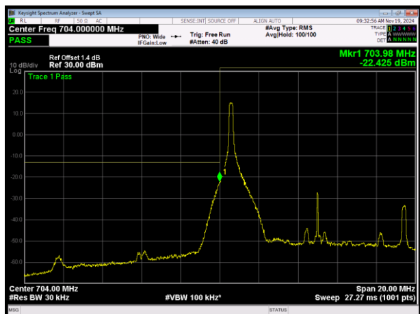
LTE Band17 16QAM BW=10MHz Channel=23780 RB Size=1 Position=#0
