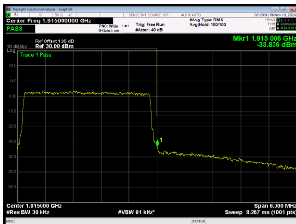
LTE Band25 16QAM BW=3MHz Channel=26675 RB Size=15 Position=#0
