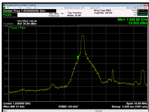
LTE Band25 16QAM BW=5MHz Channel=26065 RB Size=1 Position=#0
