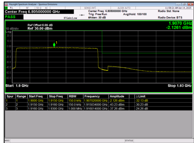
LTE Band25 64QAM BW=15MHz HighChannel=26615 RB Size=75 Position=#0
