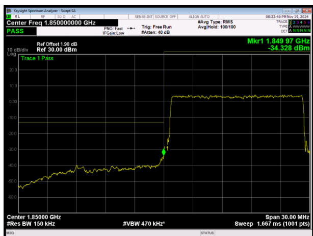
LTE Band25 QPSK BW=15MHz Channel=26115 RB Size=75 Position=#0
