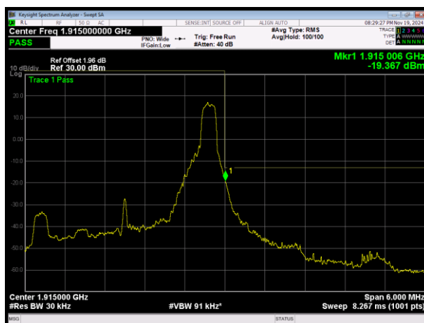
LTE Band25 QPSK BW=3MHz Channel=26675 RB Size=1 Position=#Max
