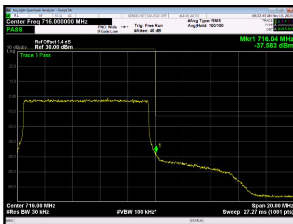
LTE Band17 16QAM BW=10MHz Channel=23800 RB Size=50 Position=#0
