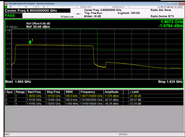
LTE Band25 64QAM BW=10MHz HighChannel=26640 RB Size=50 Position=#0
