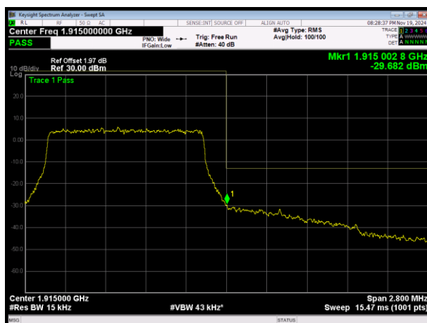
LTE Band25 QPSK BW=1.4MHz Channel=26683 RB Size=6 Position=#0
