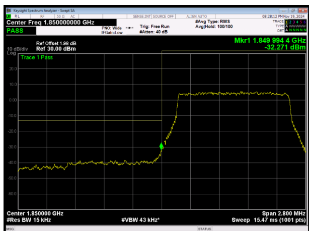
LTE Band25 QPSK BW=1.4MHz Channel=26047 RB Size=6 Position=#0
