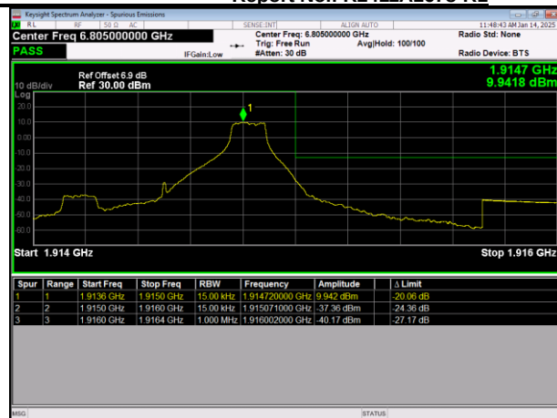
LTE Band25 64QAM BW=1.4MHz HighChannel=26683 RB Size=1 Position=#Max
