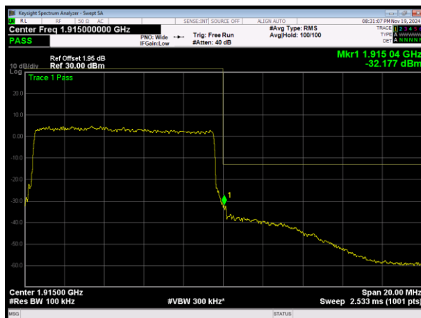
LTE Band25 QPSK BW=10MHz Channel=26640 RB Size=50 Position=#0
