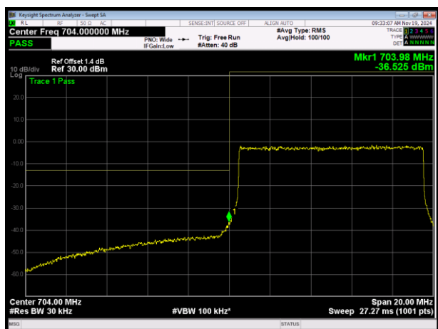
LTE Band17 16QAM BW=10MHz Channel=23780 RB Size=50 Position=#0
