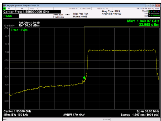
LTE Band25 16QAM BW=15MHz Channel=26115 RB Size=75 Position=#0
