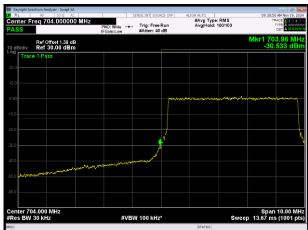
LTE Band17 16QAM BW=5MHz Channel=23755 RB Size=25 Position=#0
