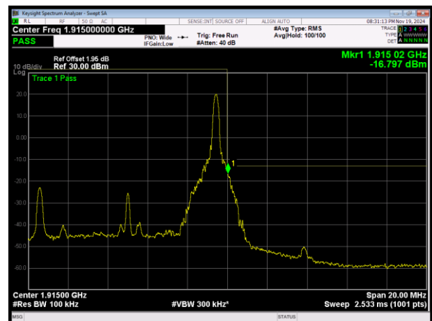
LTE Band25 16QAM BW=10MHz Channel=26640 RB Size=1 Position=#Max
