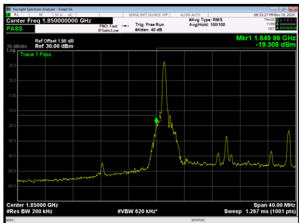
LTE Band25 QPSK BW=20MHz Channel=26140 RB Size=1 Position=#0
