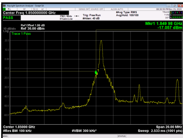
LTE Band25 16QAM BW=10MHz Channel=26090 RB Size=1 Position=#0
