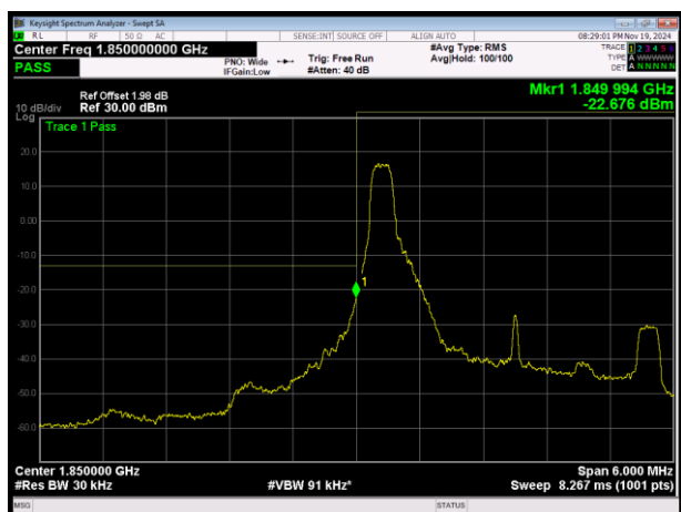
LTE Band25 QPSK BW=3MHz Channel=26055 RB Size=1 Position=#0
