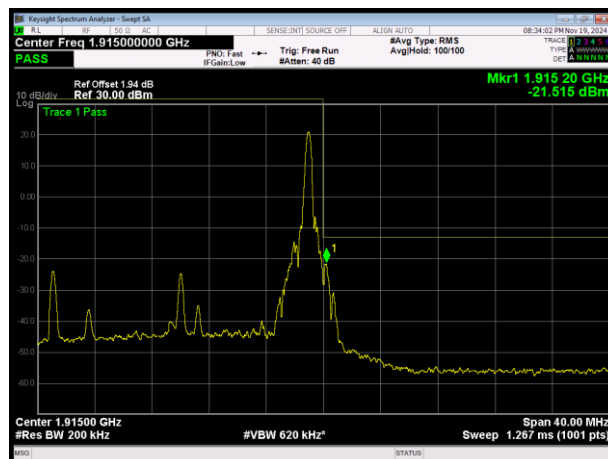
LTE Band25 16QAM BW=20MHz Channel=26590 RB Size=1 Position=#Max
