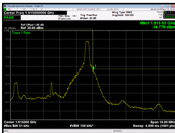
LTE Band25 QPSK BW=5MHz Channel=26665 RB Size=1 Position=#Max
