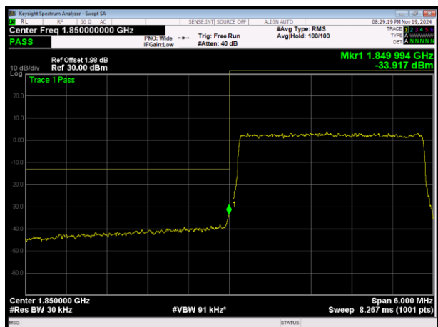
LTE Band25 16QAM BW=3MHz Channel=26055 RB Size=15 Position=#0
