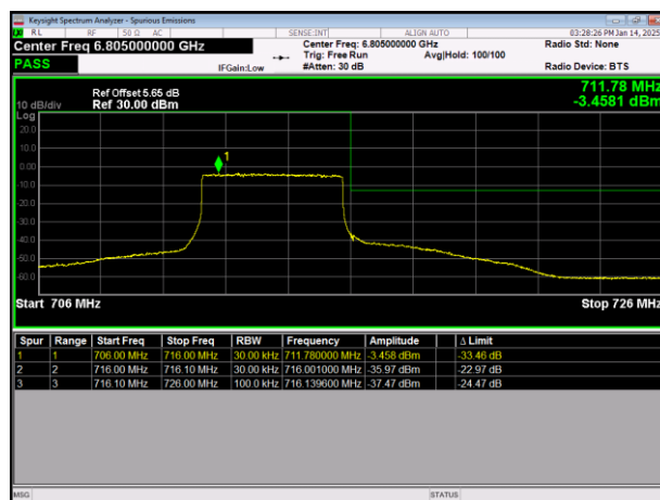
LTE Band12 64QAM BW=5MHz HighChannel=23155 RB Size=25 Position=#0
