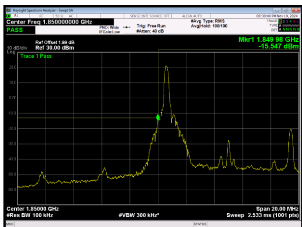
LTE Band25 QPSK BW=10MHz Channel=26090 RB Size=1 Position=#0
