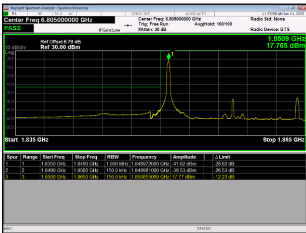
LTE Band25 64QAM BW=15MHz LowChannel=26115 RB Size=1 Position=#0
