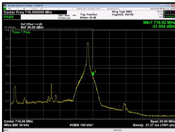
LTE Band17 16QAM BW=10MHz Channel=23800 RB Size=1 Position=#Max
