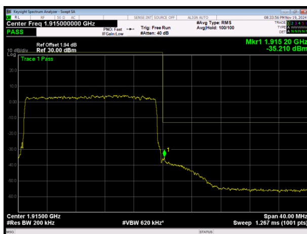
LTE Band25 QPSK BW=20MHz Channel=26590 RB Size=100 Position=#0
