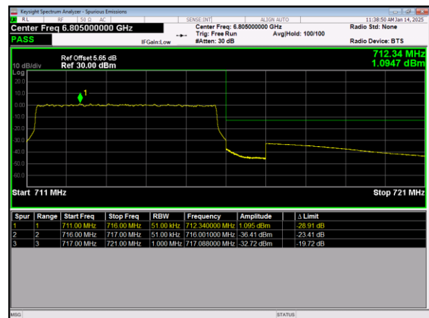
LTE Band17 64QAM BW=5MHz HighChannel=23825 RB Size=25 Position=#0
