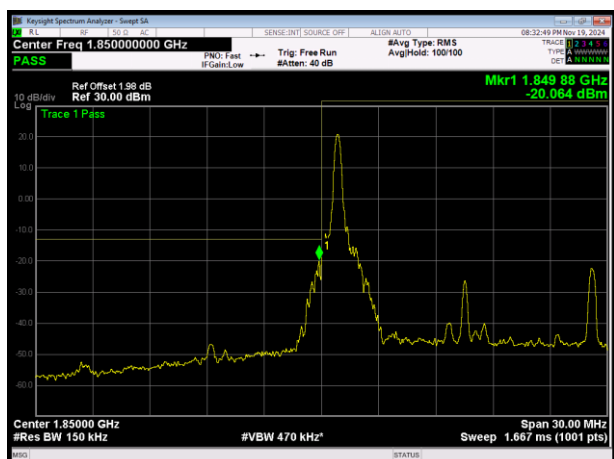
LTE Band25 16QAM BW=15MHz Channel=26115 RB Size=1 Position=#0
