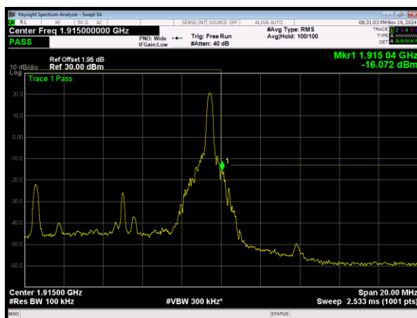
LTE Band25 QPSK BW=10MHz Channel=26640 RB Size=1 Position=#Max
