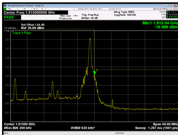
LTE Band25 QPSK BW=20MHz Channel=26590 RB Size=1 Position=#Max
