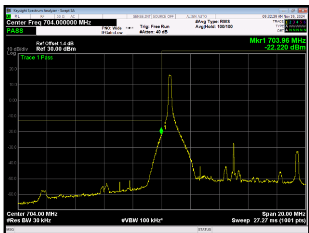
LTE Band17 QPSK BW=10MHz Channel=23780 RB Size=1 Position=#0
