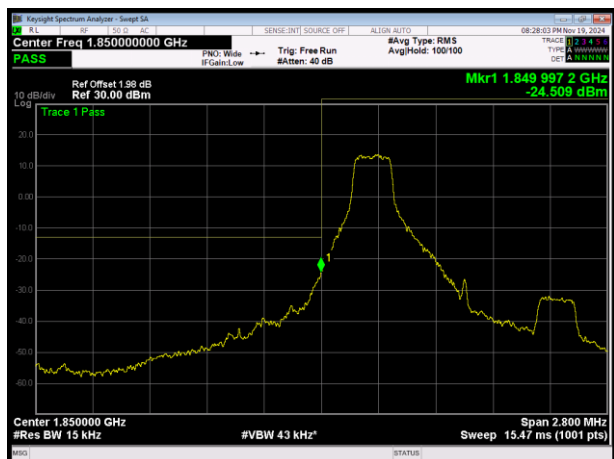
LTE Band25 QPSK BW=1.4MHz Channel=26047 RB Size=1 Position=#0
