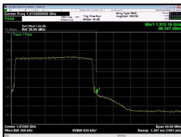
LTE Band25 16QAM BW=20MHz Channel=26590 RB Size=100 Position=#0
