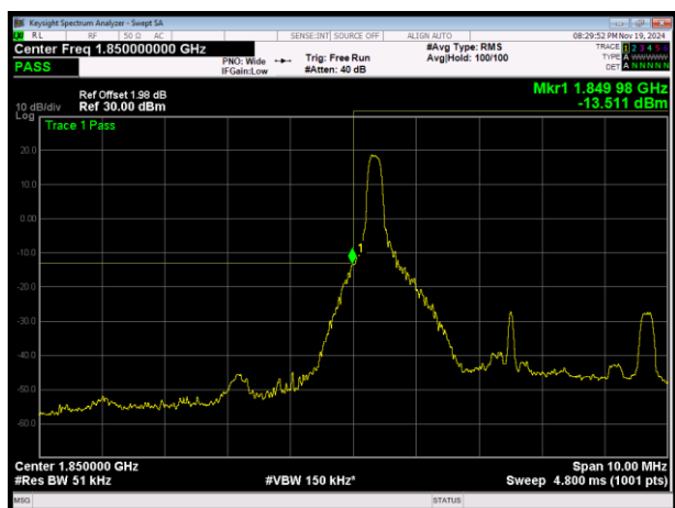
LTE Band25 QPSK BW=5MHz Channel=26065 RB Size=1 Position=#0
