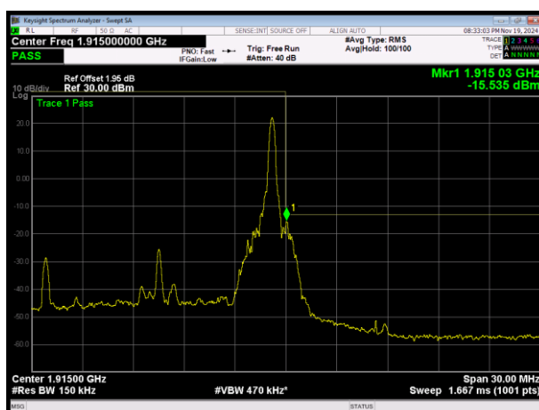
LTE Band25 QPSK BW=15MHz Channel=26615 RB Size=1 Position=#Max
