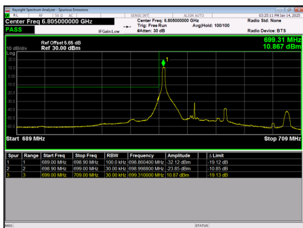
LTE Band12 64QAM BW=5MHz LowChannel=23035 RB Size=1 Position=#0
