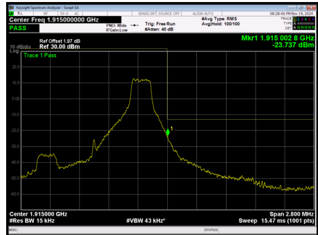
LTE Band25 16QAM BW=1.4MHz Channel=26683 RB Size=1 Position=#Max
