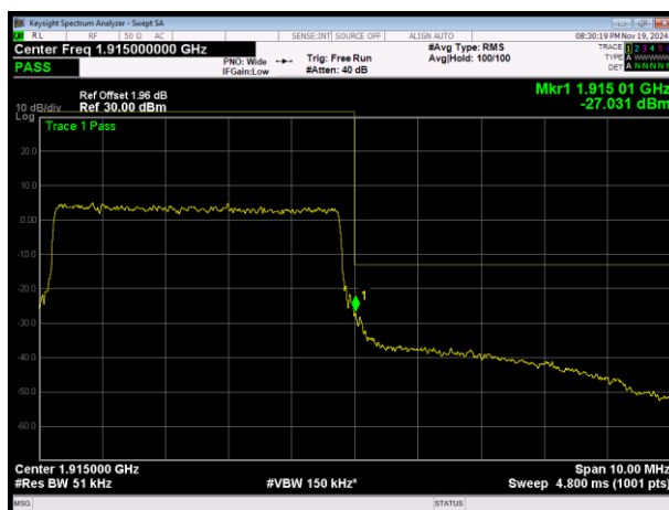
LTE Band25 QPSK BW=5MHz Channel=26665 RB Size=25 Position=#0
