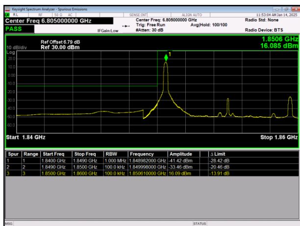
LTE Band25 64QAM BW=10MHz LowChannel=26090 RB Size=1 Position=#0
