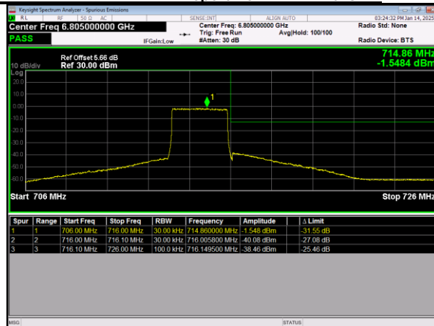
LTE Band12 64QAM BW=3MHz HighChannel=23165 RB Size=15 Position=#0
