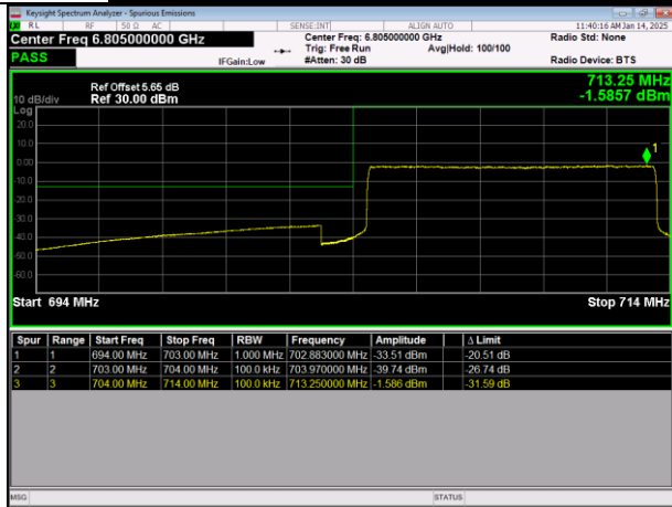
LTE Band17 64QAM BW=10MHz LowChannel=23780 RB Size=50 Position=#0
