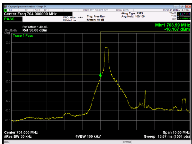
LTE Band17 16QAM BW=5MHz Channel=23755 RB Size=1 Position=#0
