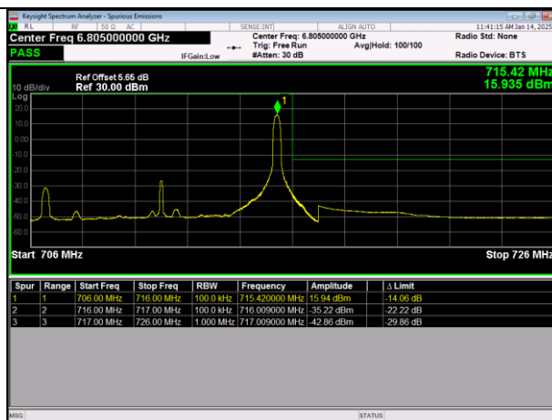
LTE Band17 64QAM BW=10MHz HighChannel=23800 RB Size=1 Position=#Max
