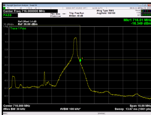
LTE Band17 16QAM BW=5MHz Channel=23825 RB Size=1 Position=#Max
