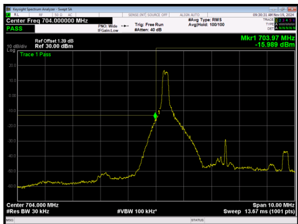
LTE Band17 QPSK BW=5MHz Channel=23755 RB Size=1 Position=#0
