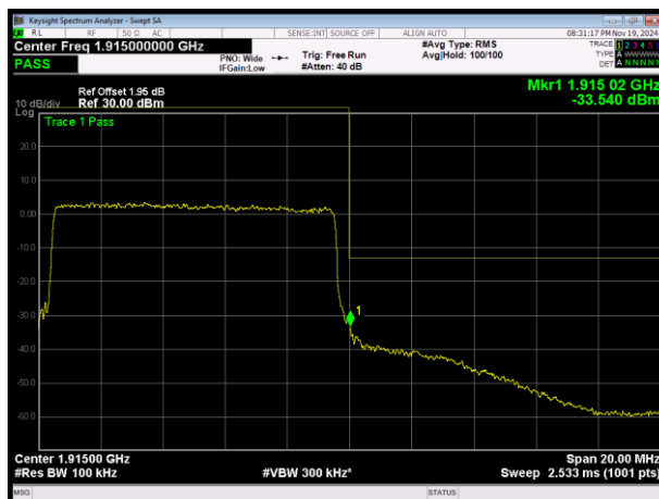
LTE Band25 16QAM BW=10MHz Channel=26640 RB Size=50 Position=#0
