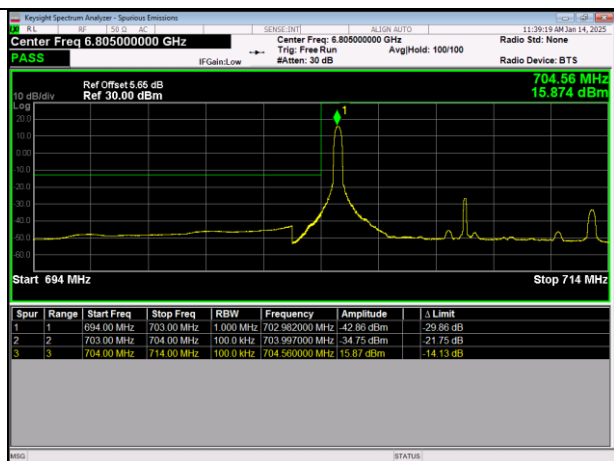
LTE Band17 64QAM BW=10MHz LowChannel=23780 RB Size=1 Position=#0
