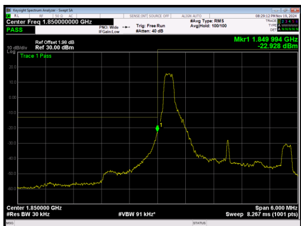
LTE Band25 16QAM BW=3MHz Channel=26055 RB Size=1 Position=#0
