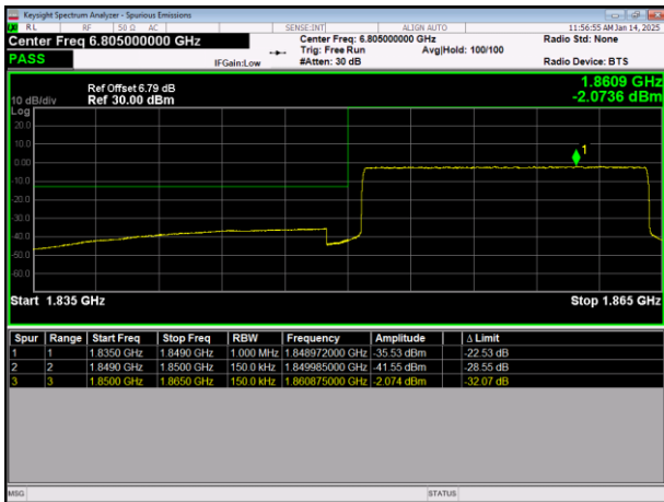
LTE Band25 64QAM BW=15MHz LowChannel=26115 RB Size=75 Position=#0
