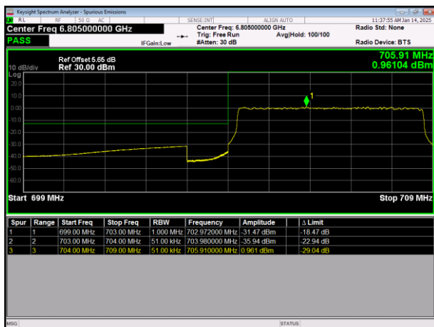
LTE Band17 64QAM BW=5MHz LowChannel=23755 RB Size=25 Position=#0
