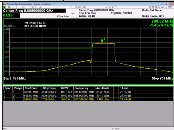
LTE Band12 64QAM BW=3MHz LowChannel=23025 RB Size=15 Position=#0
