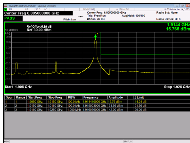
LTE Band25 64QAM BW=10MHz HighChannel=26640 RB Size=1 Position=#Max
