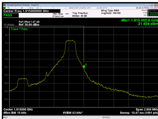
LTE Band25 QPSK BW=1.4MHz Channel=26683 RB Size=1 Position=#Max
