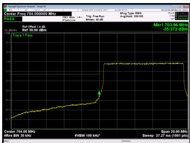
LTE Band17 QPSK BW=10MHz Channel=23780 RB Size=50 Position=#0
