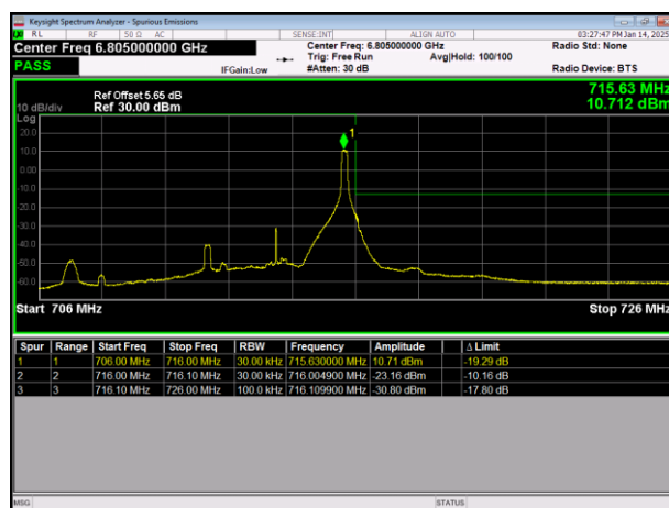
LTE Band12 64QAM BW=5MHz HighChannel=23155 RB Size=1 Position=#Max
