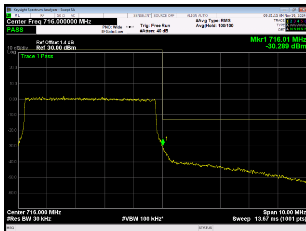
LTE Band17 16QAM BW=5MHz Channel=23825 RB Size=25 Position=#0
