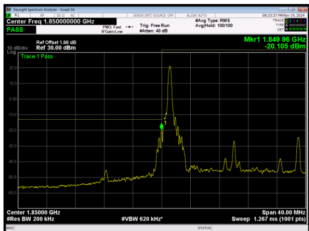
LTE Band25 16QAM BW=20MHz Channel=26140 RB Size=1 Position=#0
