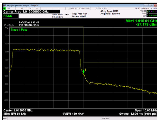
LTE Band25 16QAM BW=5MHz Channel=26665 RB Size=25 Position=#0
