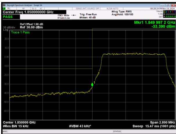
LTE Band25 16QAM BW=1.4MHz Channel=26047 RB Size=6 Position=#0
