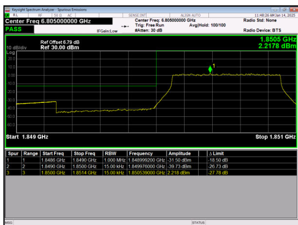
LTE Band25 64QAM BW=1.4MHz LowChannel=26047 RB Size=6 Position=#0
