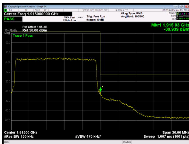
LTE Band25 QPSK BW=15MHz Channel=26615 RB Size=75 Position=#0
