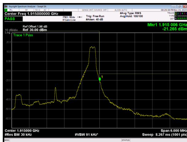
LTE Band25 16QAM BW=3MHz Channel=26675 RB Size=1 Position=#Max
