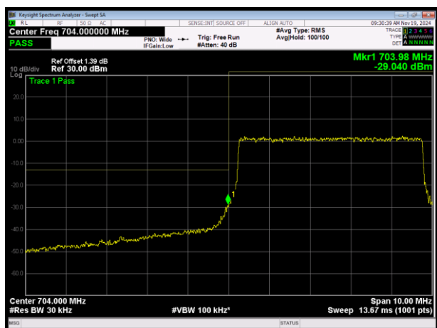
LTE Band17 QPSK BW=5MHz Channel=23755 RB Size=25 Position=#0
